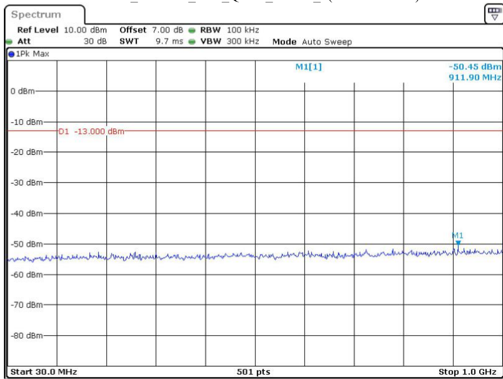
Band 2_1.4 MHz_Low_QPSK_RB6#0_1(30MHz-1GHz)
