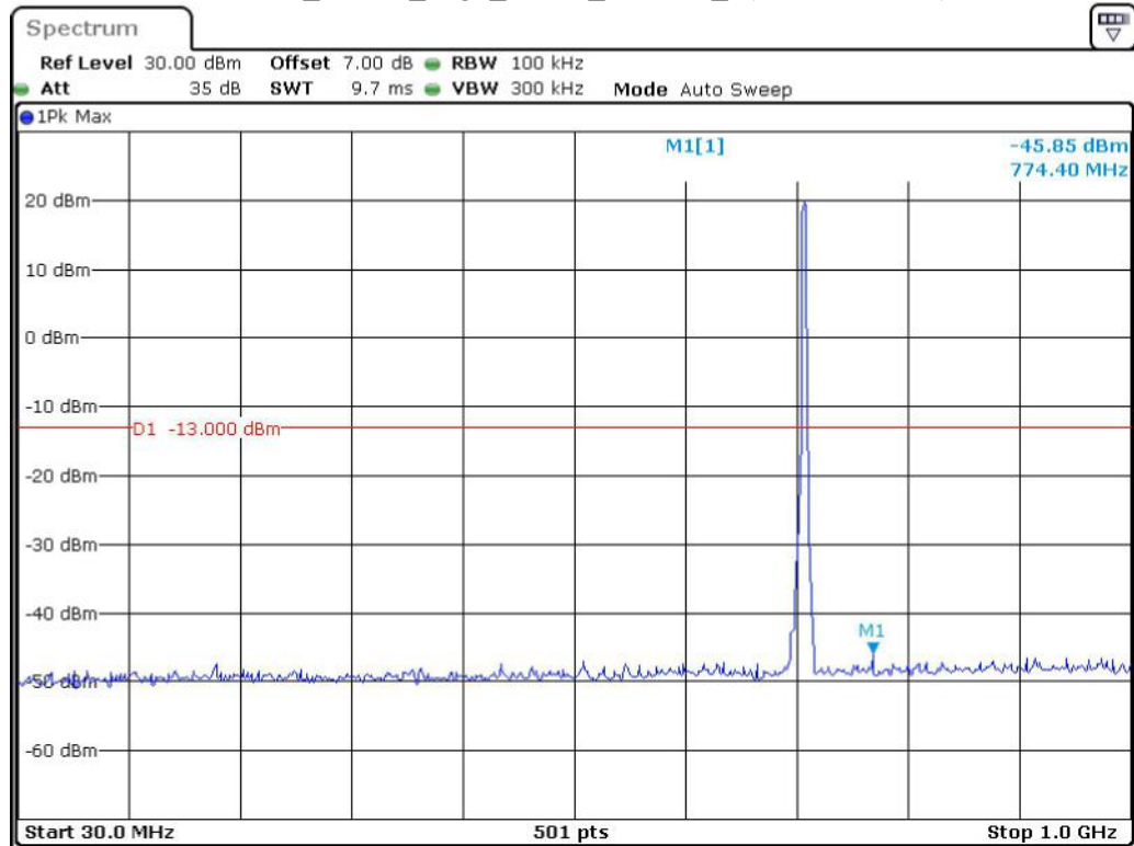
Band 12_3 MHz_High_QPSK_RB15#0_1(30MHz-1GHz)
