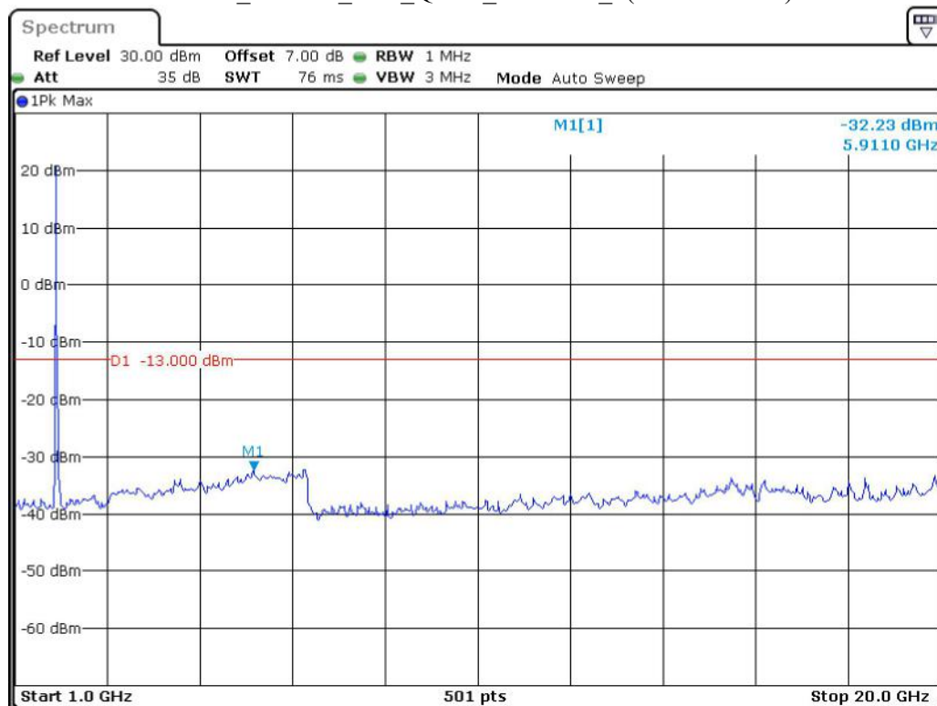
Band 2_20 MHz_Low_QPSK_RB100#0_2(1GHz-20GHz)
