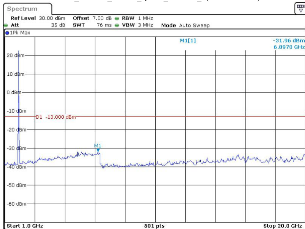
Band 2_15 MHz_Middle_QPSK_RB75#0_2(1GHz-20GHz)
