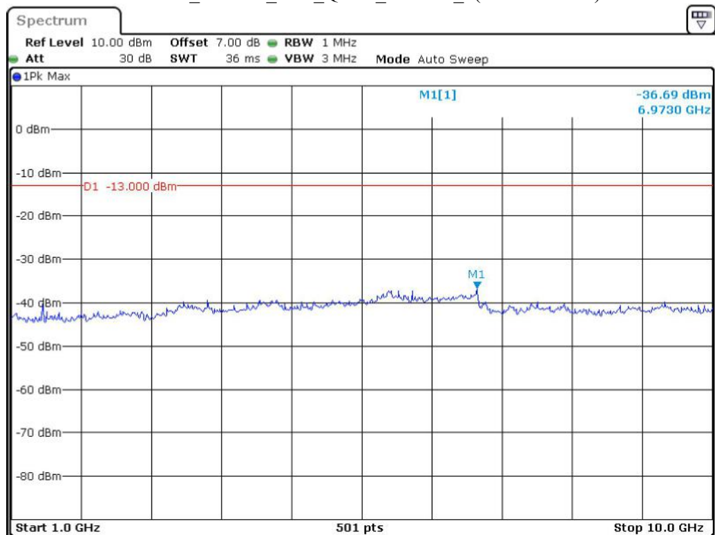
Band 12_10 MHz_Low_QPSK_RB50#0_2(1GHz-10GHz)
