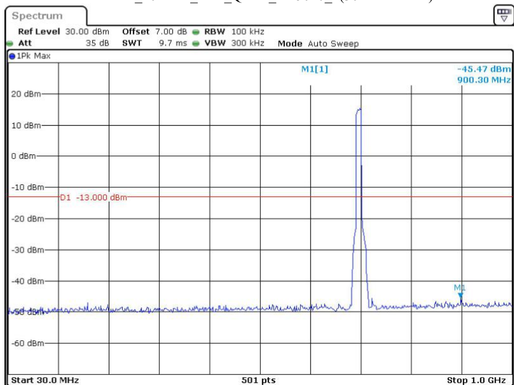
Band 12_10 MHz_Low_QPSK_RB50#0_1(30MHz-1GHz)
