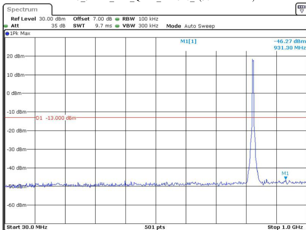
Band 5_5 MHz_Low_QPSK_RB25#0_1(30MHz-1GHz)
