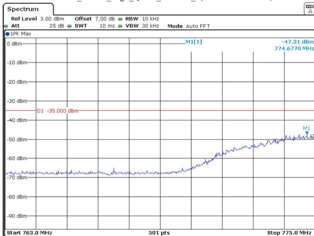
Band 13_5 MHz_High_QPSK_RB25#0_2(763MHz-775MHz)
