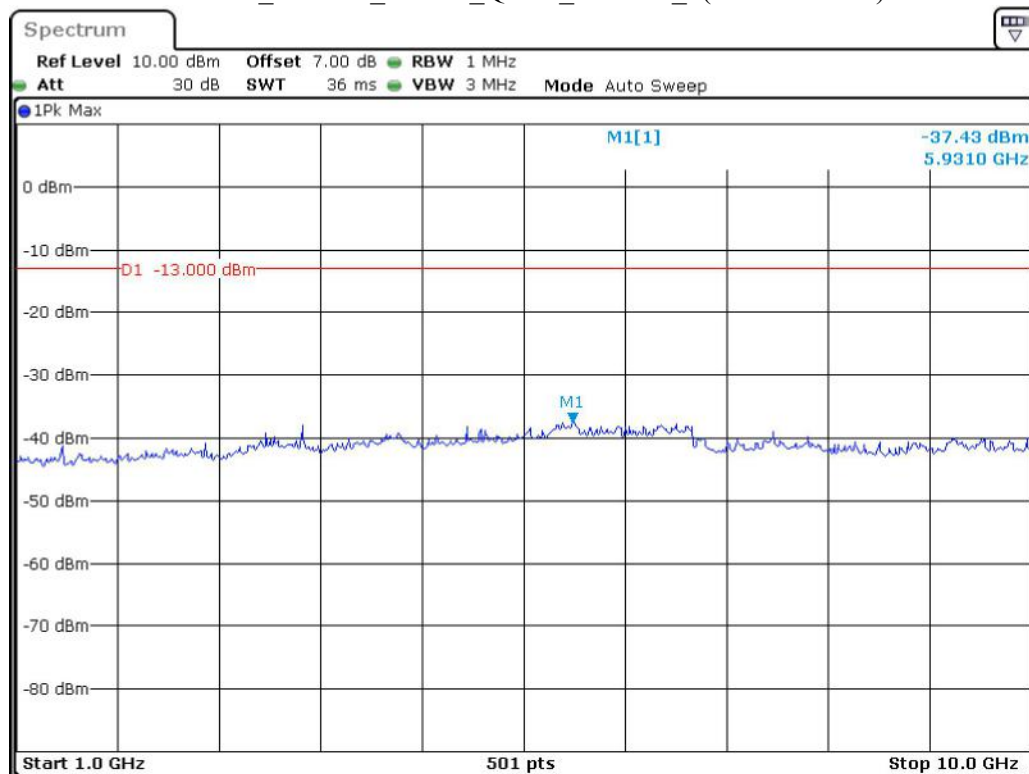
Band 12_10 MHz_Middle_QPSK_RB50#0_2(1GHz-10GHz)
