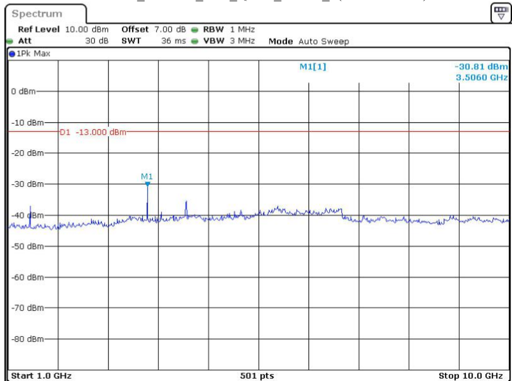
Band 12_1.4 MHz_Low_QPSK_RB6#0_2(1GHz-10GHz)
