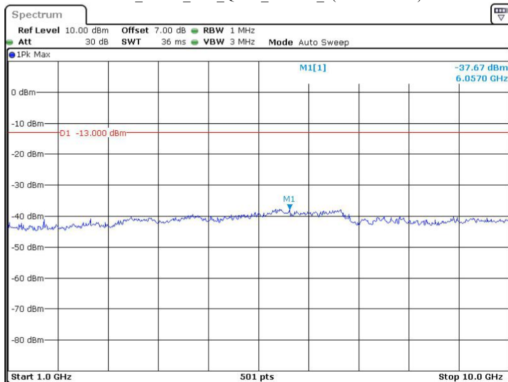
Band 5_5 MHz_Low_QPSK_RB25#0_2(1GHz-10GHz)
