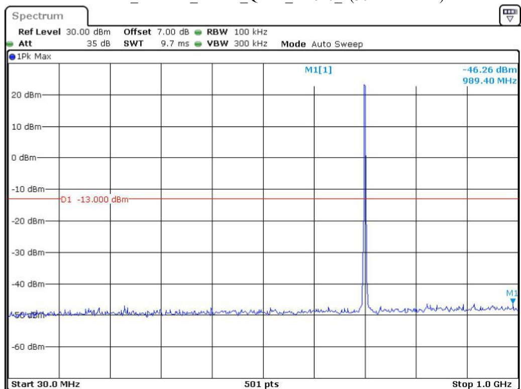
Band 12_1.4 MHz_Middle_QPSK_RB6#0_1(30MHz-1GHz)
