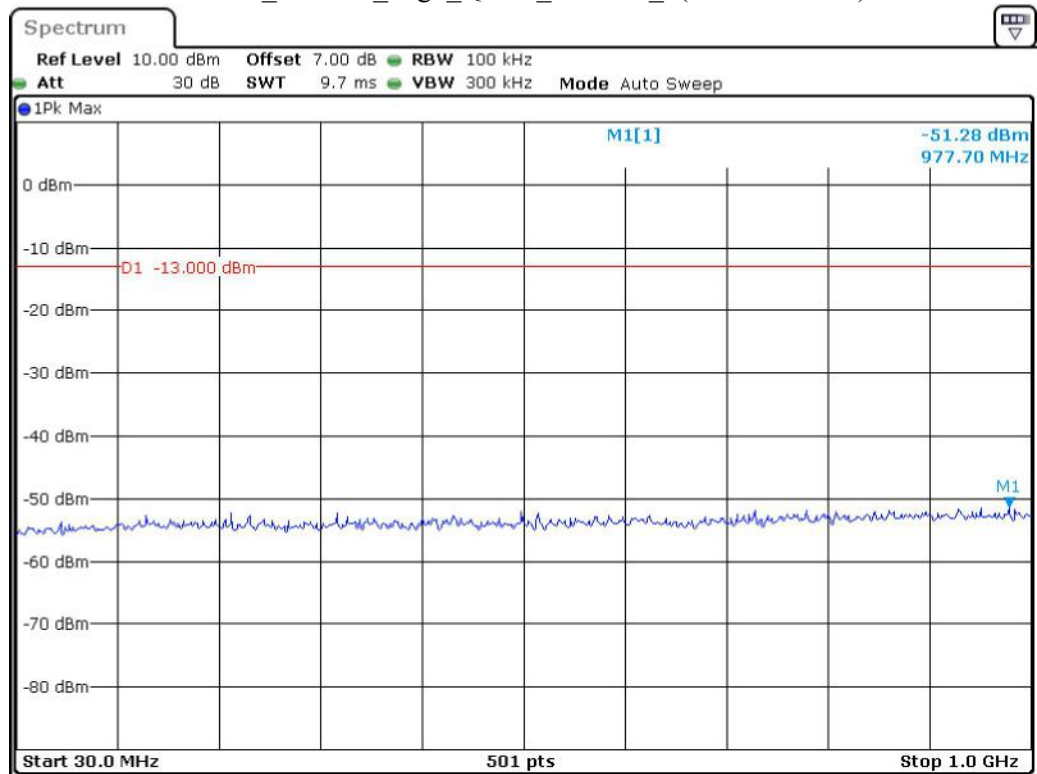
Band 2_15 MHz_High_QPSK_RB75#0_1(30MHz-1GHz)
