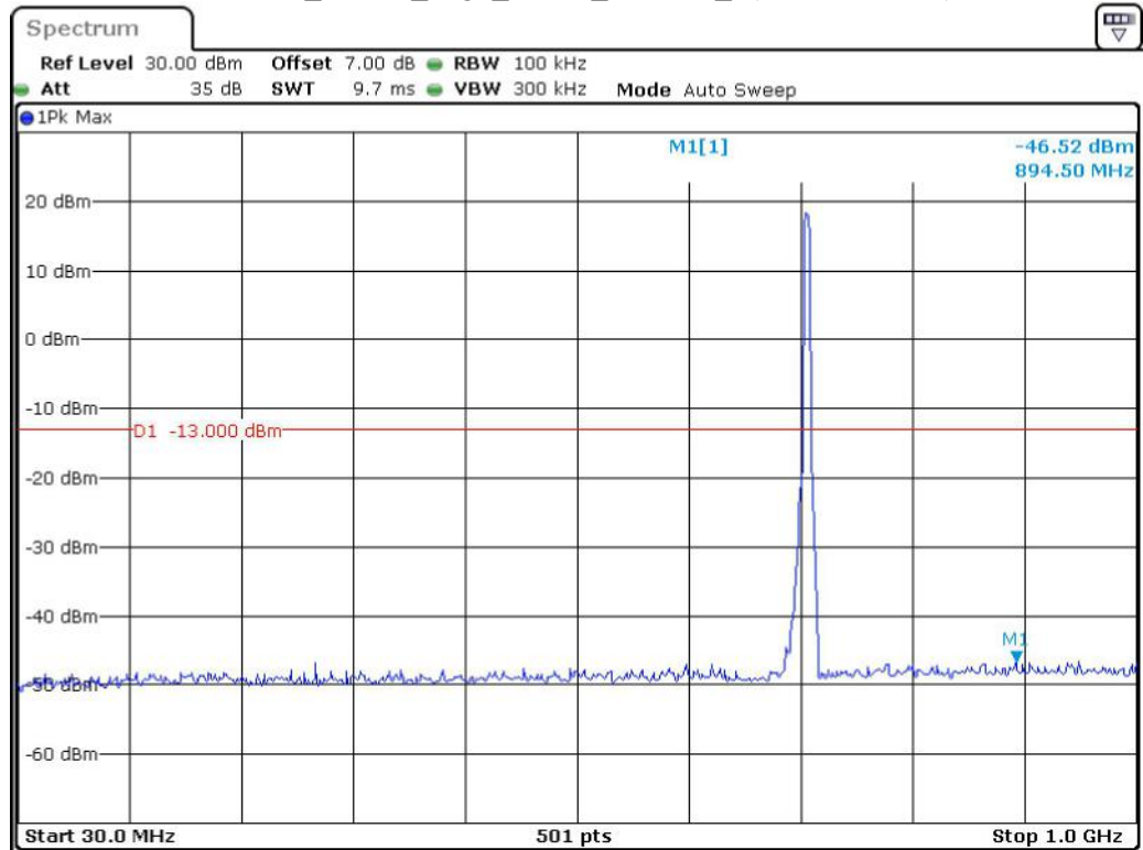
Band 12_5 MHz_High_QPSK_RB25#0_1(30MHz-1GHz)
