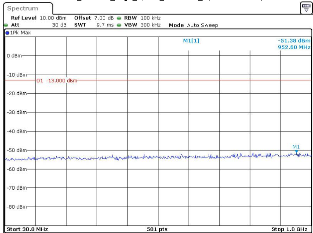
Band 2_20 MHz_High_QPSK_RB100#0_1(30MHz-1GHz)
