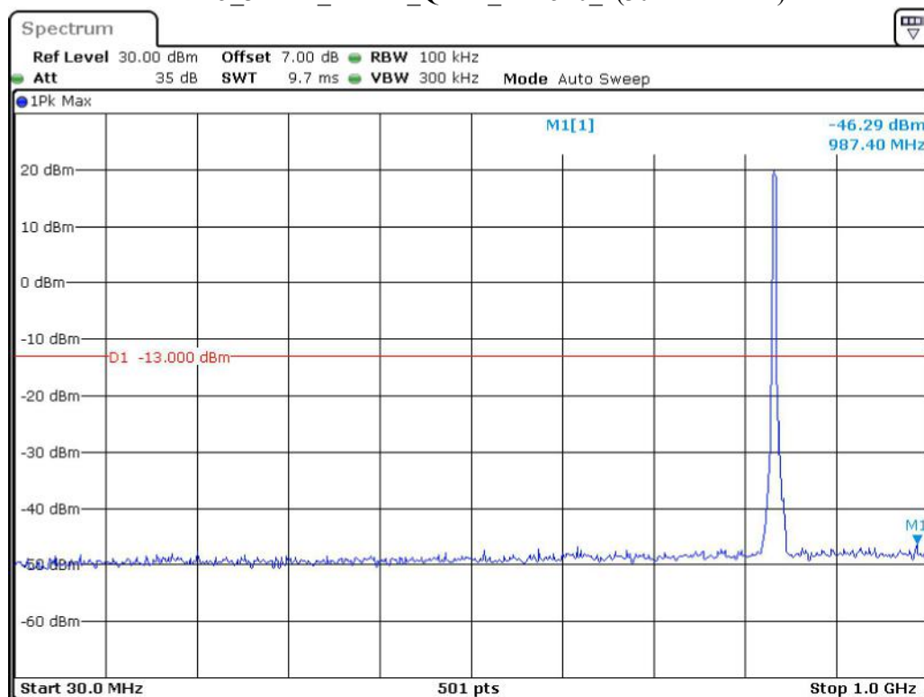
Band 5_3 MHz_Middle_QPSK_RB15#0_1(30MHz-1GHz)
