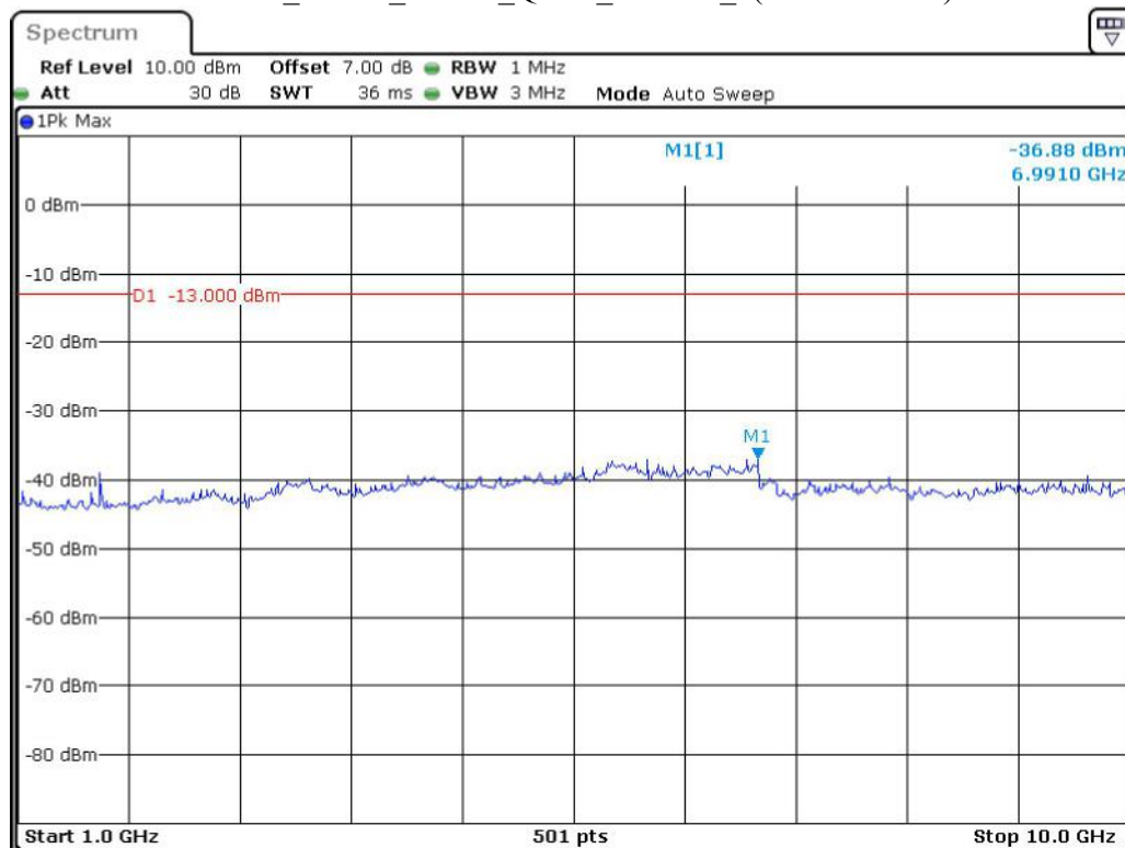
Band 5_3 MHz_Middle_QPSK_RB15#0_2(1GHz-10GHz)
