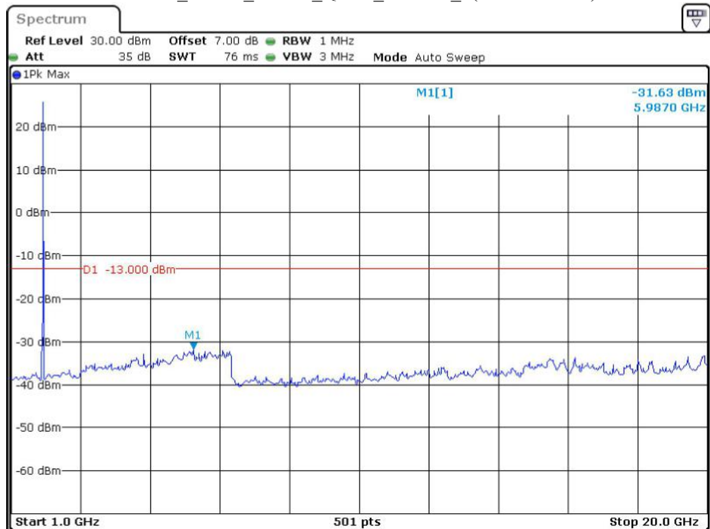
Band 2_3 MHz_Middle_QPSK_RB15#0_2(1GHz-20GHz)
