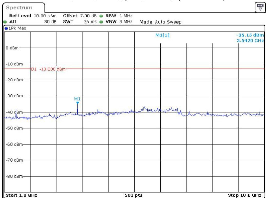
Band 12_3 MHz_Middle_QPSK_RB15#0_2(1GHz-10GHz)
