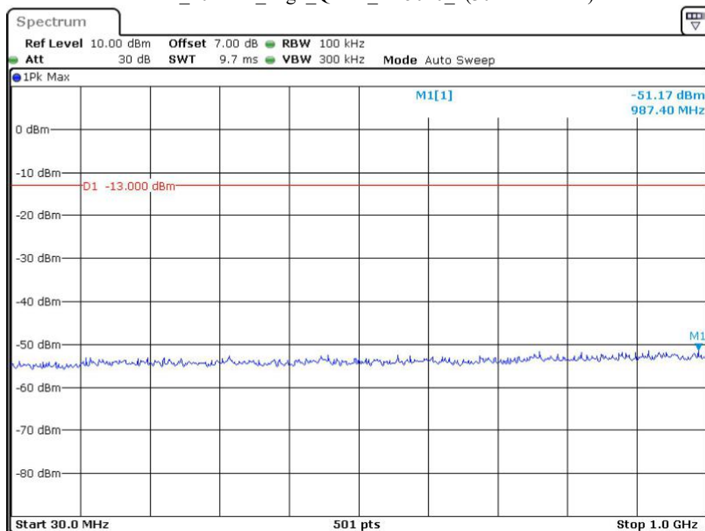
Band 2_10 MHz_High_QPSK_RB50#0_1(30MHz-1GHz)
