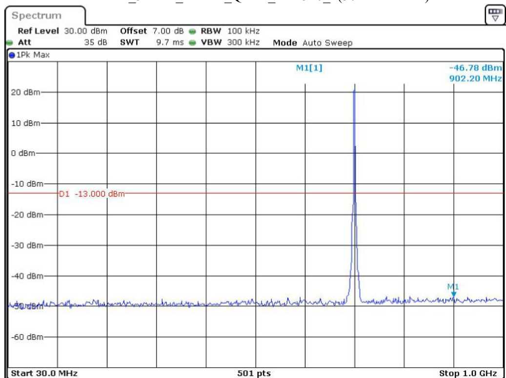
Band 12_3 MHz_Middle_QPSK_RB15#0_1(30MHz-1GHz)
