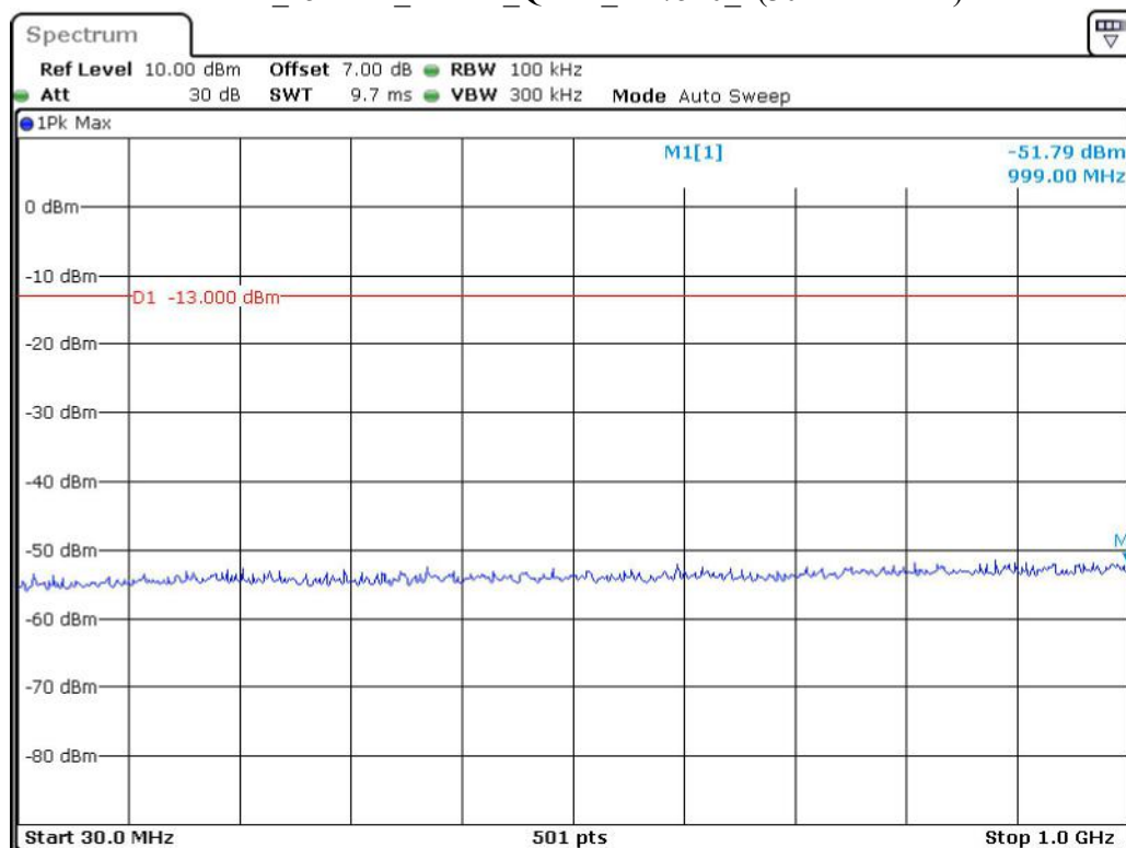
Band 2_15 MHz_Middle_QPSK_RB75#0_1(30MHz-1GHz)
