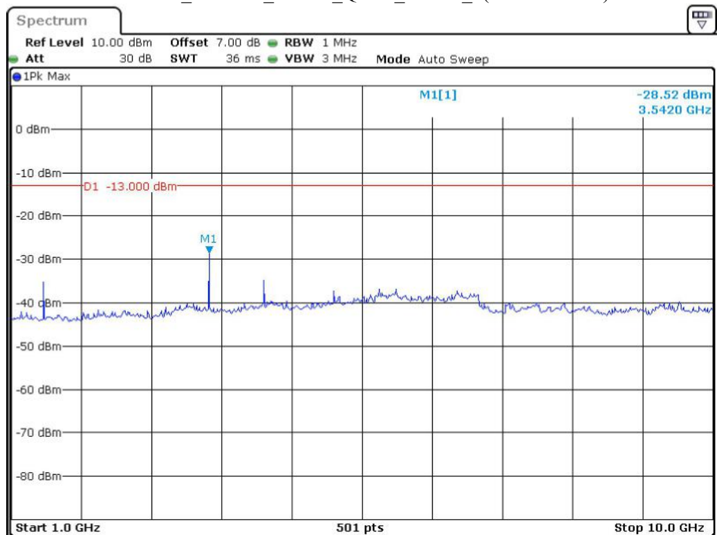
Band 12_1.4 MHz_Middle_QPSK_RB6#0_2(1GHz-10GHz)
