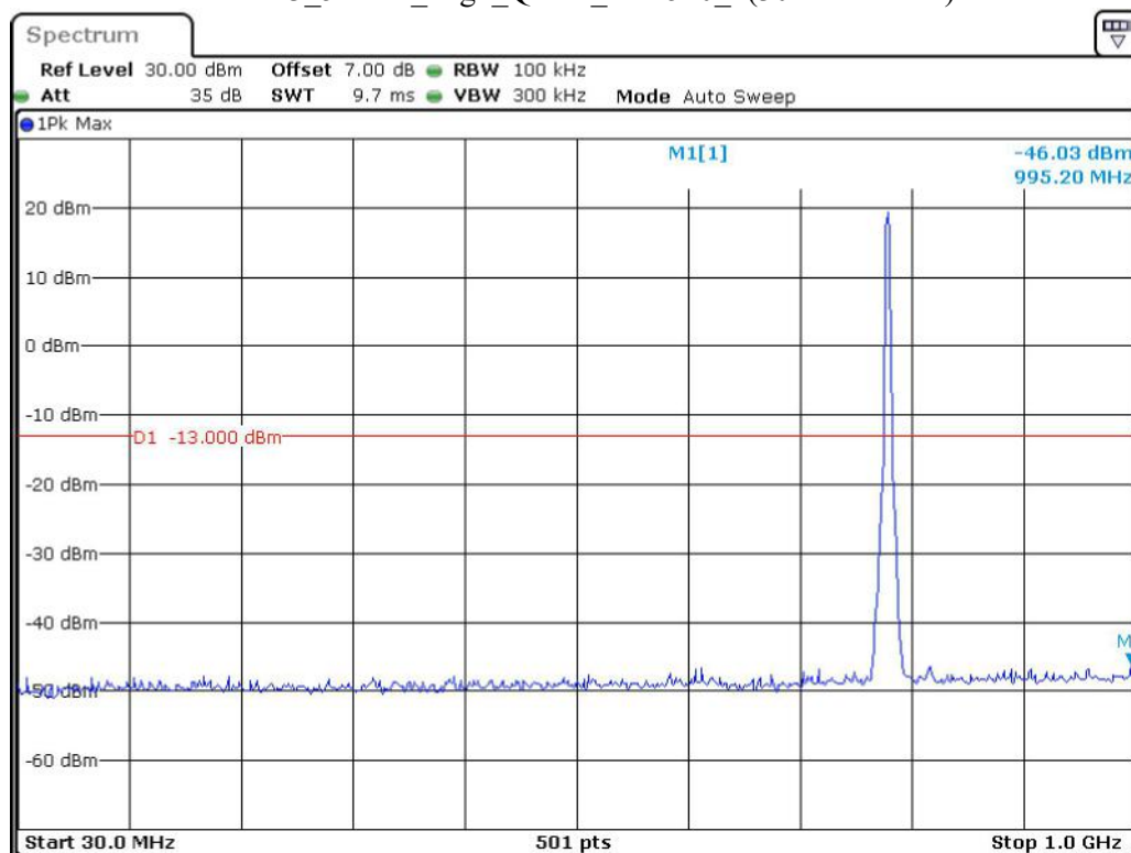
Band 13_5 MHz_High_QPSK_RB25#0_1(30MHz-1GHz)
