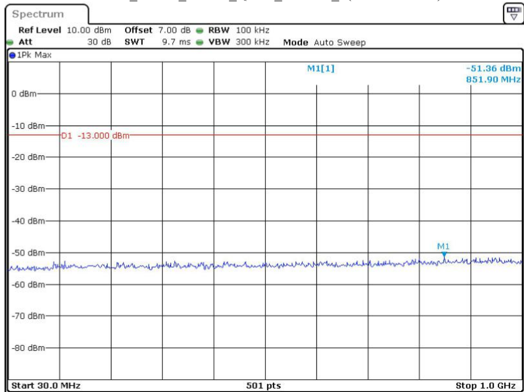
Band 2_3 MHz_Middle_QPSK_RB15#0_1(30MHz-1GHz)
