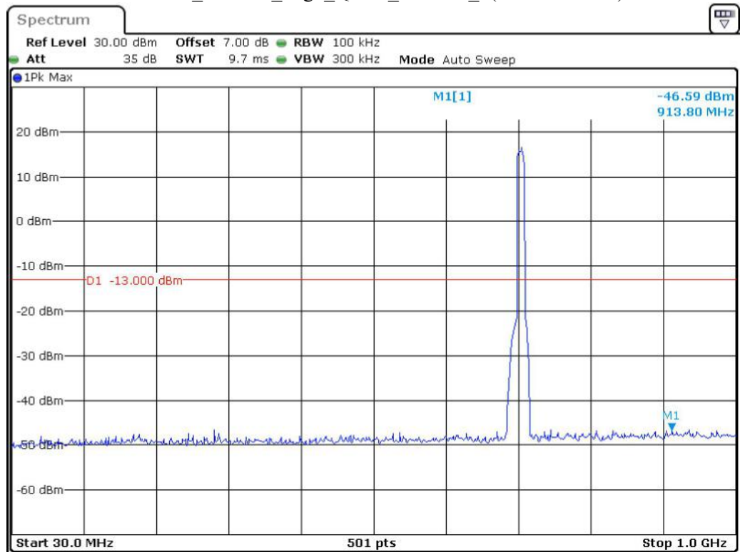
Band 12_10 MHz_High_QPSK_RB50#0_1(30MHz-1GHz)
