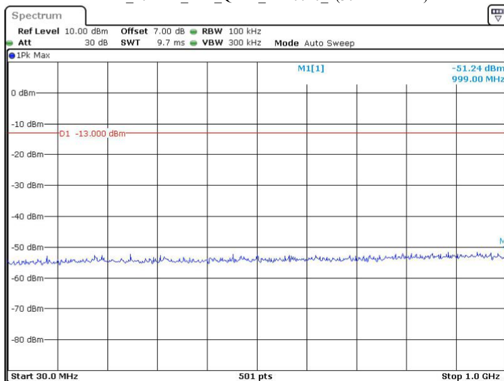
Band 2_20 MHz_Low_QPSK_RB100#0_1(30MHz-1GHz)
