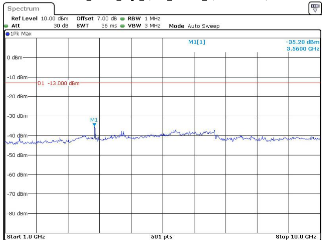
Band 12_5 MHz_High_QPSK_RB25#0_2(1GHz-10GHz)
