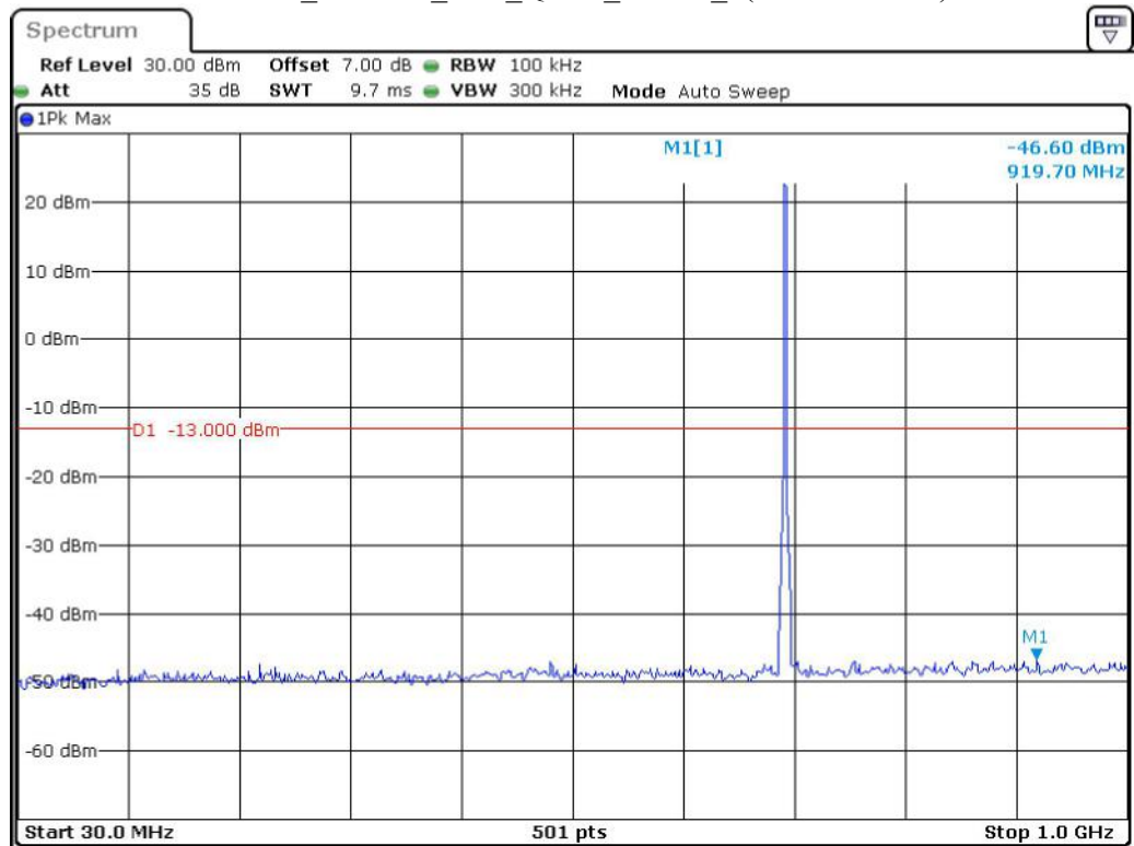
Band 12_1.4 MHz_Low_QPSK_RB6#0_1(30MHz-1GHz)
