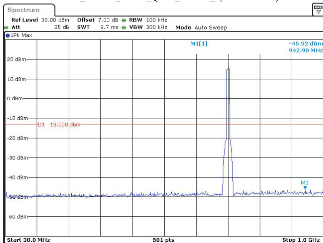
Band 12_10 MHz_Middle_QPSK_RB50#0_1(30MHz-1GHz)
