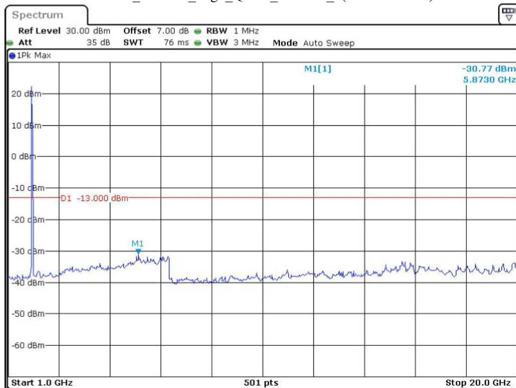
Band 2_10 MHz_High_QPSK_RB50#0_2(1GHz-20GHz)
