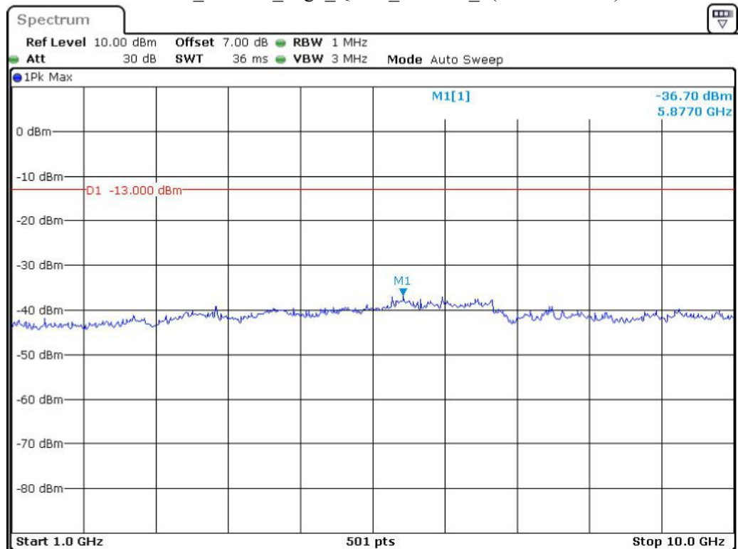
Band 12_10 MHz_High_QPSK_RB50#0_2(1GHz-10GHz)
