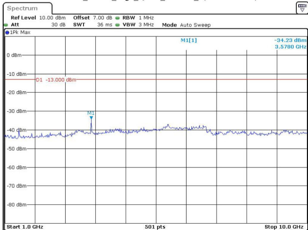
Band 12_3 MHz_High_QPSK_RB15#0_2(1GHz-10GHz)
