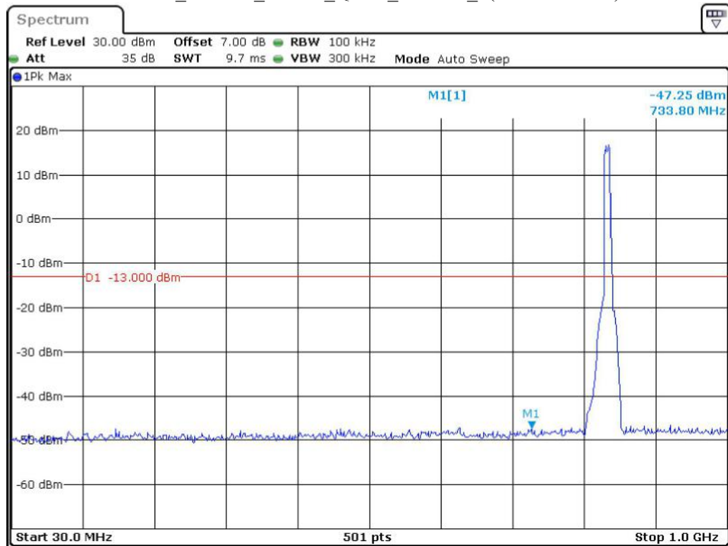
Band 5_10 MHz_Middle_QPSK_RB50#0_1(30MHz-1GHz)
