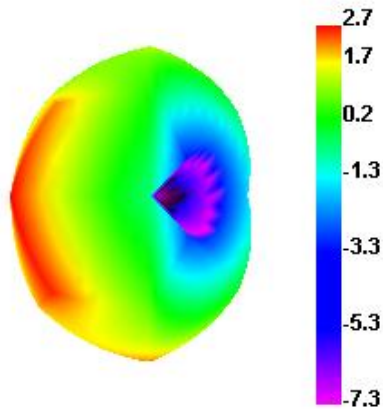
Bluetooth 78 TRP
