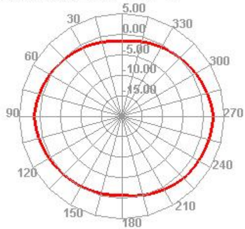
Bluetooth 78 TRP H
