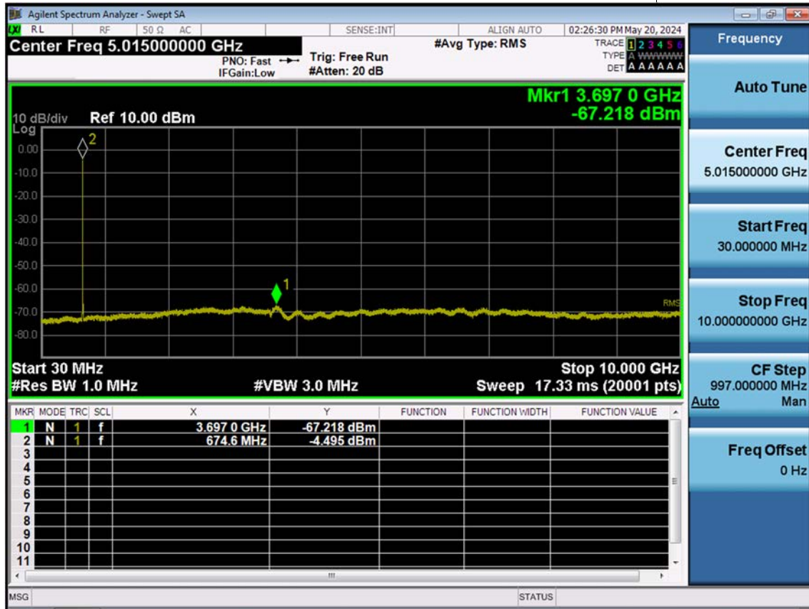
LTE B71_15 M_Conducted Spurious(30 M-10 G)_Mid_QPSK_1RB
