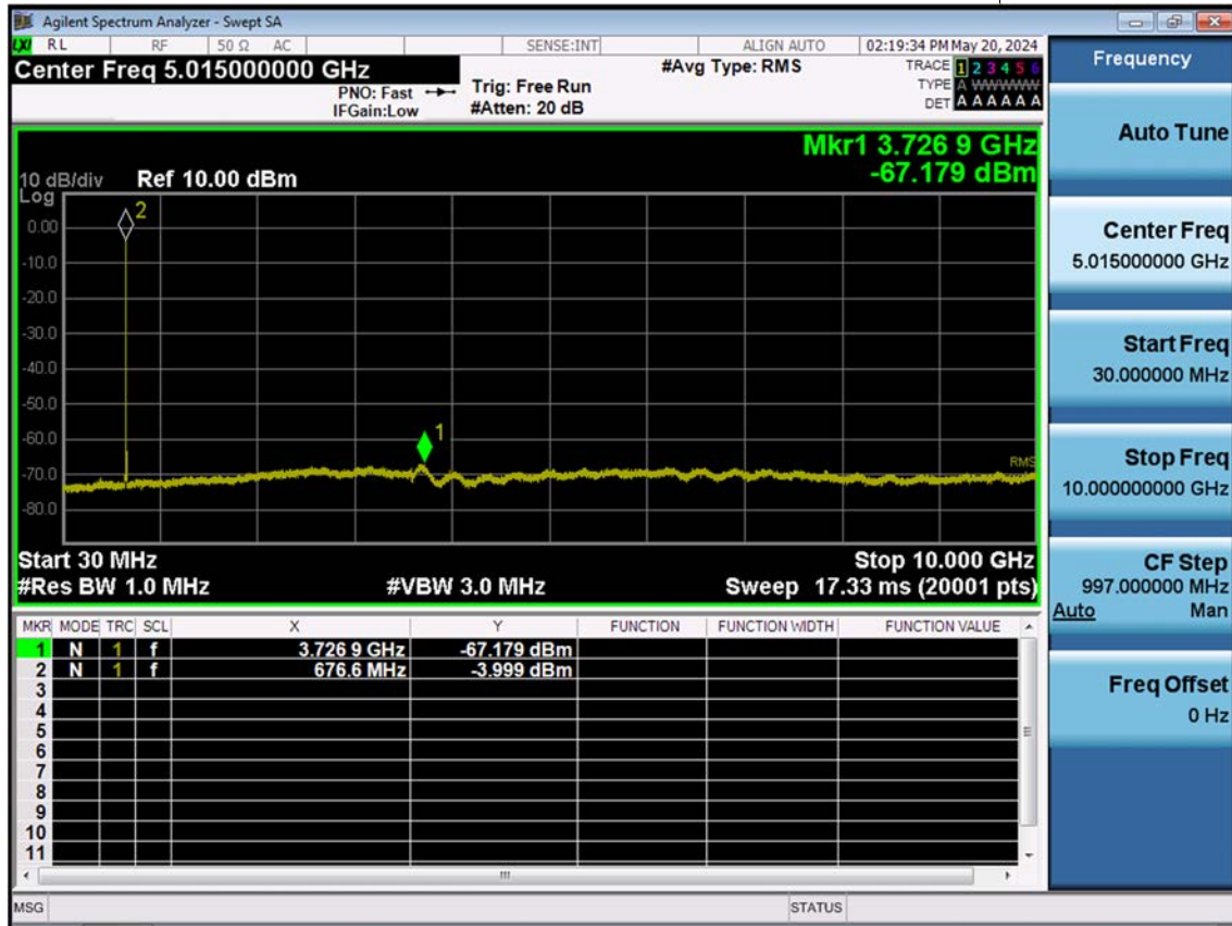
LTE B71_10 M_Conducted Spurious(30 M-10 G)_Mid_QPSK_1RB
