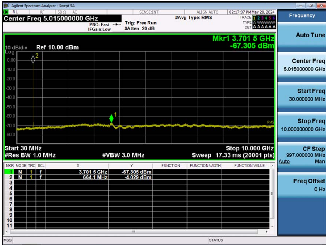
LTE B71_10 M_Conducted Spurious(30 M-10 G)_Low_QPSK_1RB
