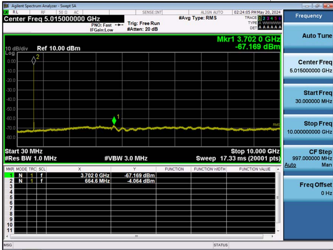
LTE B71_15 M_Conducted Spurious(30 M-10 G)_Low_QPSK_1RB
