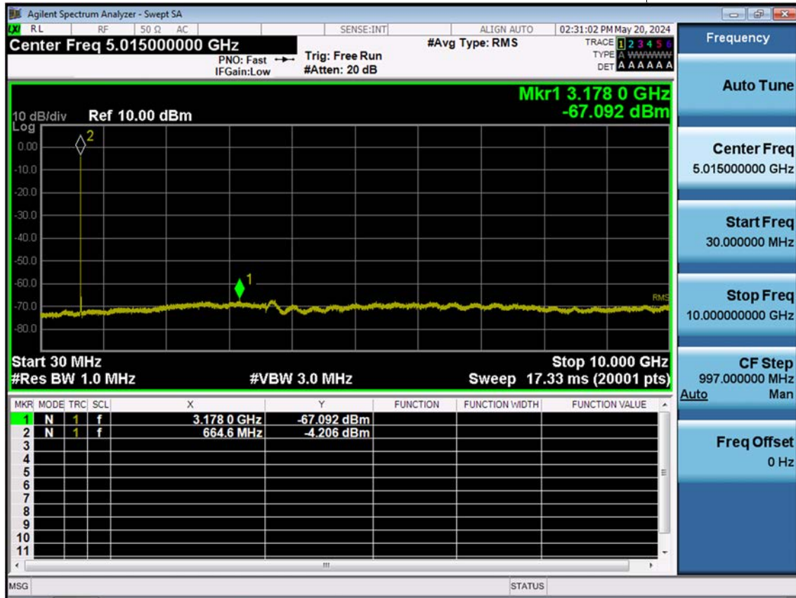
LTE B71_20 M_Conducted Spurious(30 M-10 G)_Low_QPSK_1RB
