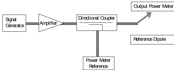
Figure 12 Setup for Desired Output Power to Dipole
