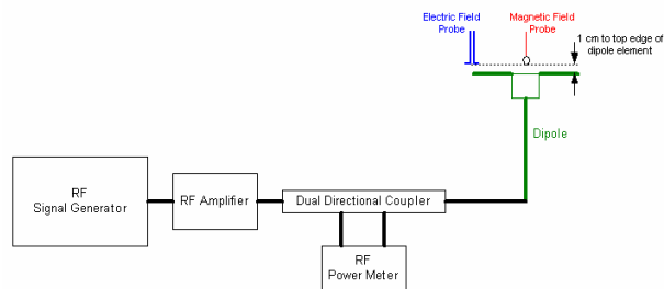
Figure 16 System Check Setup
