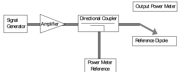
Figure 13 Setup to Dipole
