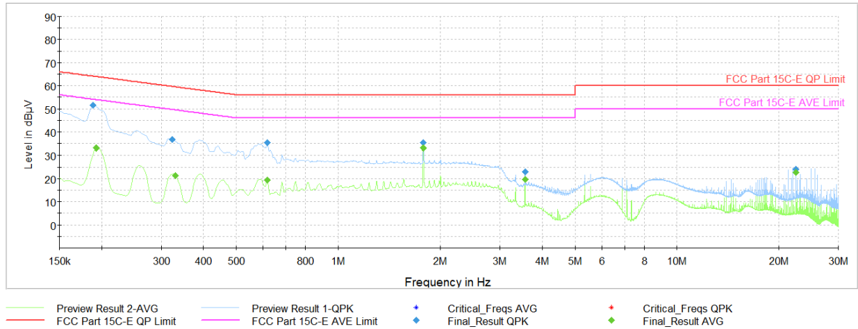
Plot 6-14. AC Line Conducted Plot (N - Mode 1, with Magnetic Charger & Laptop)
