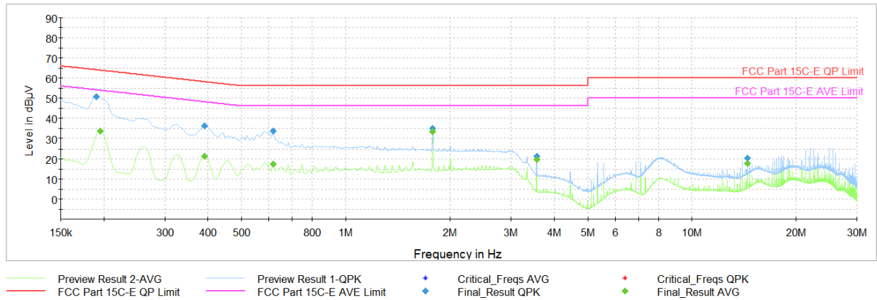
Plot 6-13. AC Line Conducted Plot (L1 - Mode 1, with Magnetic Charger & Laptop)
