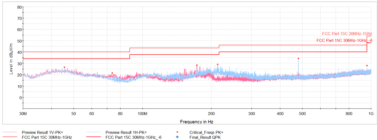
Plot 6-12. Radiated Spurious Emissions 30MHz – 1GHz (Mode 1, with Magnetic Charger & Laptop)
