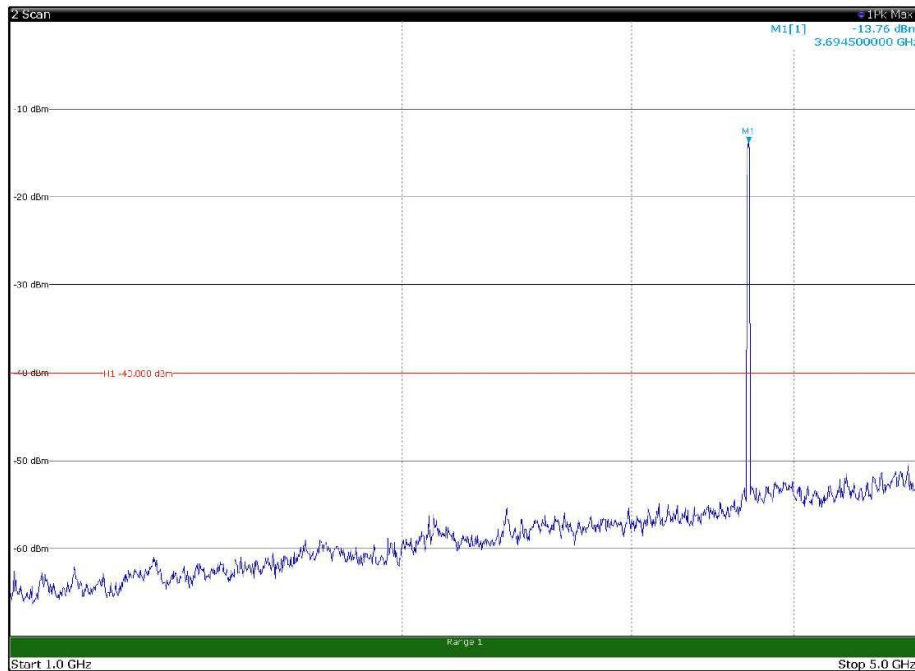
Channel: TOP, Modulation: 256QAM, BW=20MHz, Range: 1GHz - 5GHz, Polarization: Vertical
