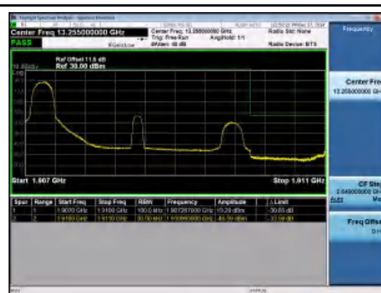
Band2-3MHz-16QAM-19185-1RB#0-PASS
