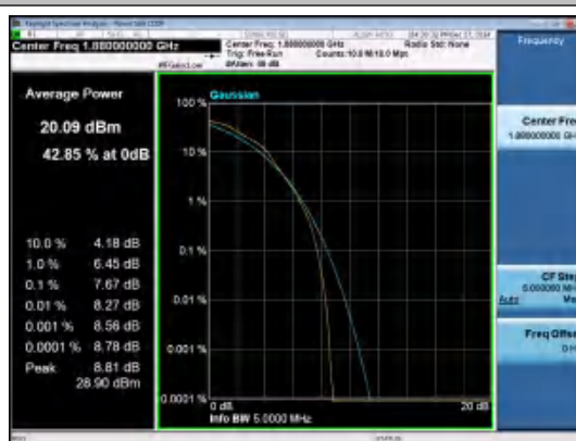
Band2-5MHz-16QAM-18900-25RB#0-PASS
