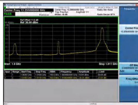
Band2-10MHz-QPSK-19150-1RB#49-PASS
