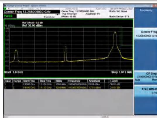
Band2-10MHz-16QAM-19150-1RB#49-PASS
