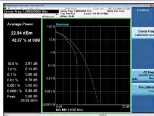
Band2-3MHz-16QAM-18900-1RB#0-PASS
