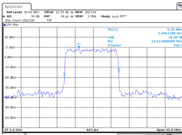
n77_1_15MHz_30kHz_3500MHz_DFT-s-OFDM \pi/2 BPSK_RB36@0 26 dB Emission Bandwidth
