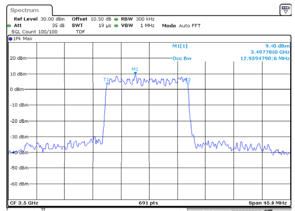
n77_1_15MHz_30kHz_3500MHz_DFT-s-OFDM QPSK_RB36@0 Occupied Bandwidth
