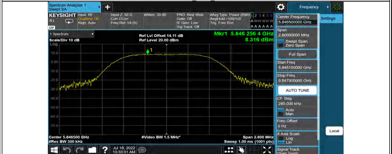
1.4M-MIMO Ant2 5846.5
