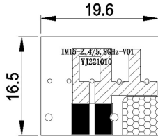
Wifi antenna
