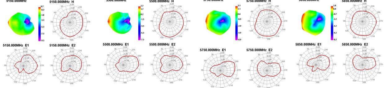
Wifi antenna
