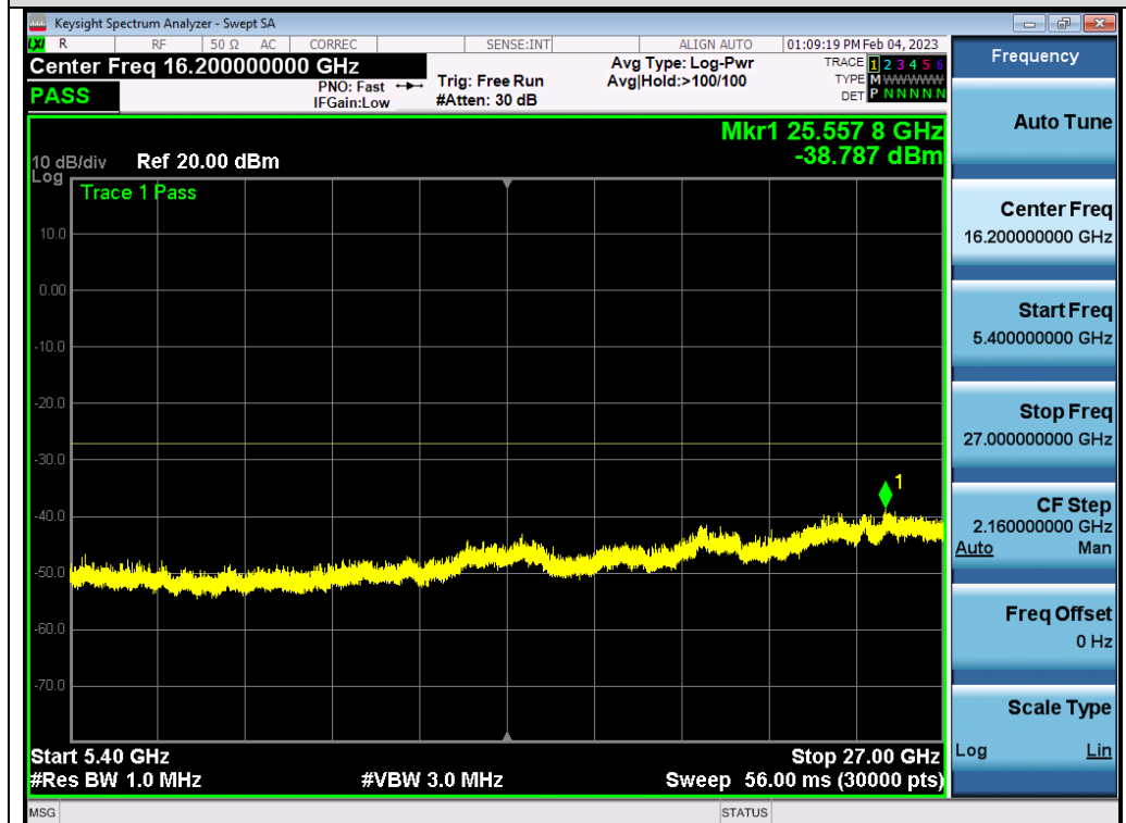
Test_Graph_802.11n40_ANT2_5190_MCS0_Frequency Band 4
