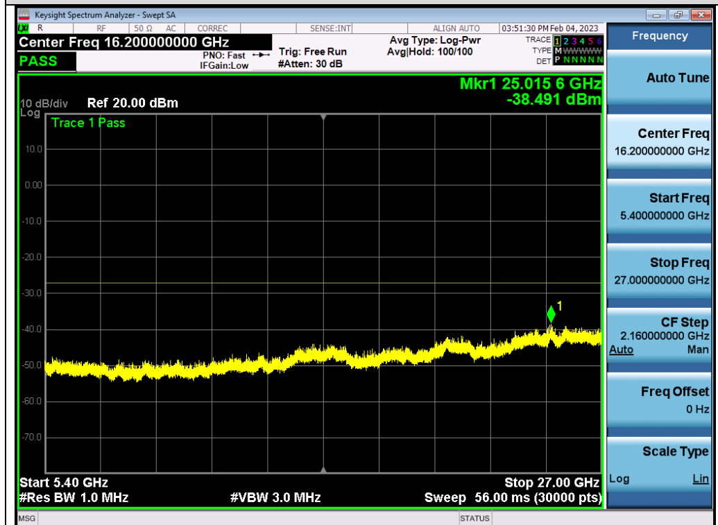
Test_Graph_802.11ax80_ANT2_5290_MCS0_Frequency Band 4
