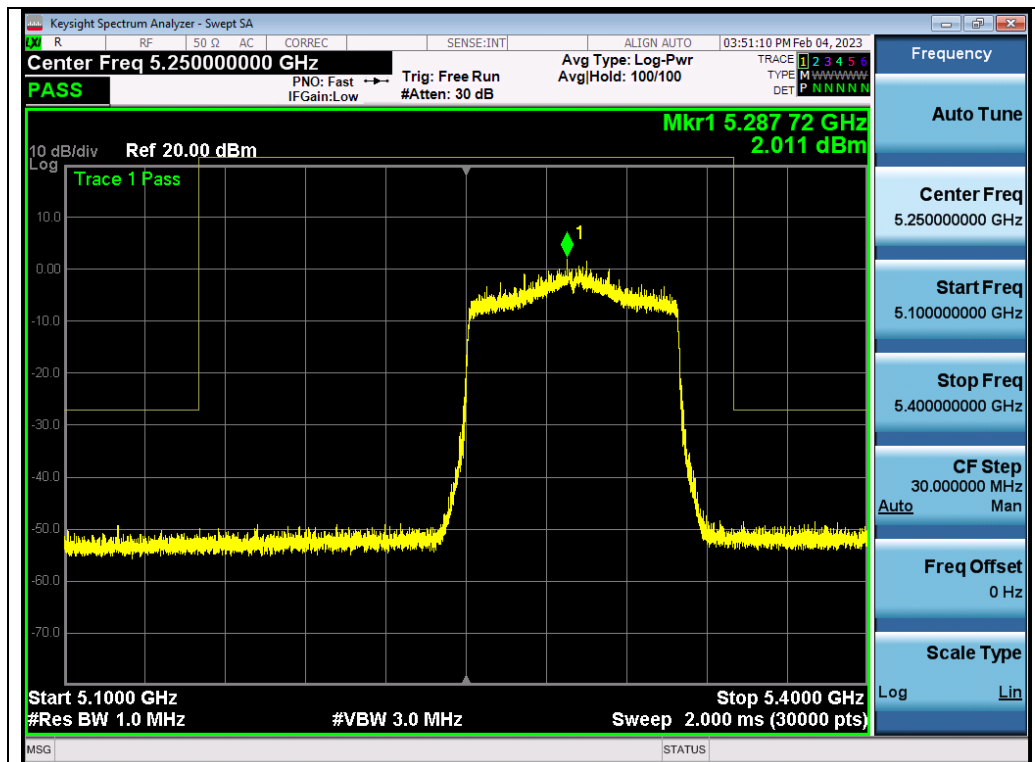
Test_Graph_802.11ax80_ANT2_5290_MCS0_Frequency Band 3
