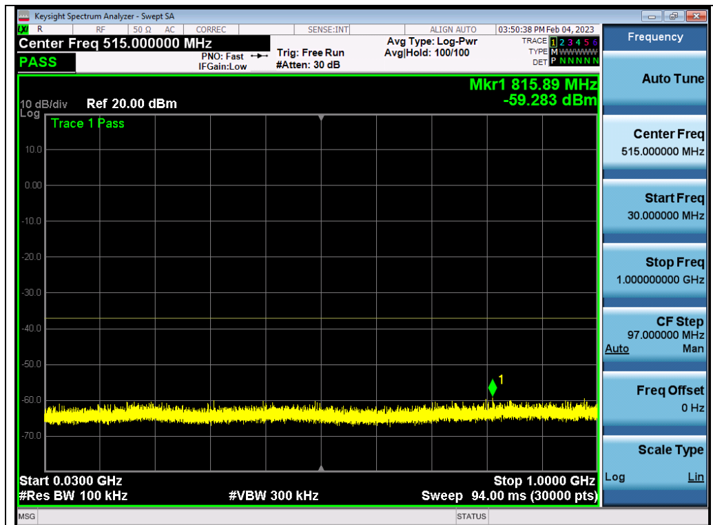
Test_Graph_802.11ax80_ANT2_5290_MCS0_Frequency Band 1
