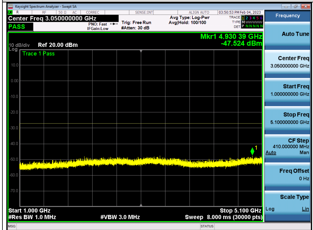
Test_Graph_802.11ax80_ANT2_5290_MCS0_Frequency Band 2
