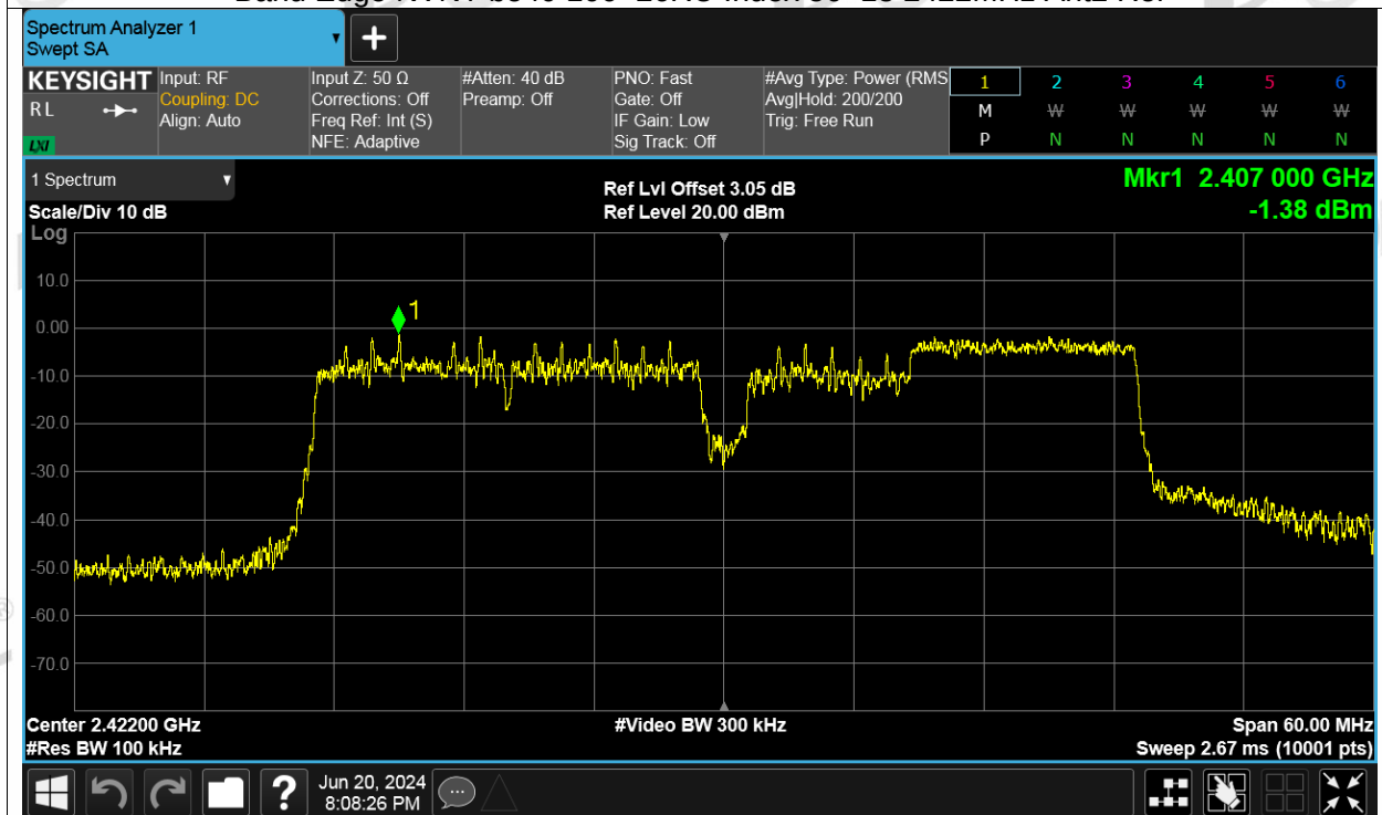
Band Edge NVNT be40 106+26RU Index 56+13 2422MHz Ant2 Emission
