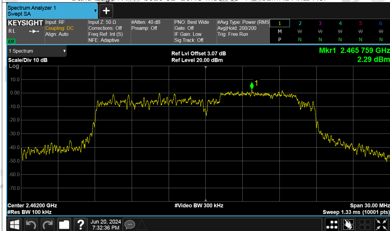
Band Edge NVNT be20 52+26RU Index 39+7 2462MHz Ant2 Emission
