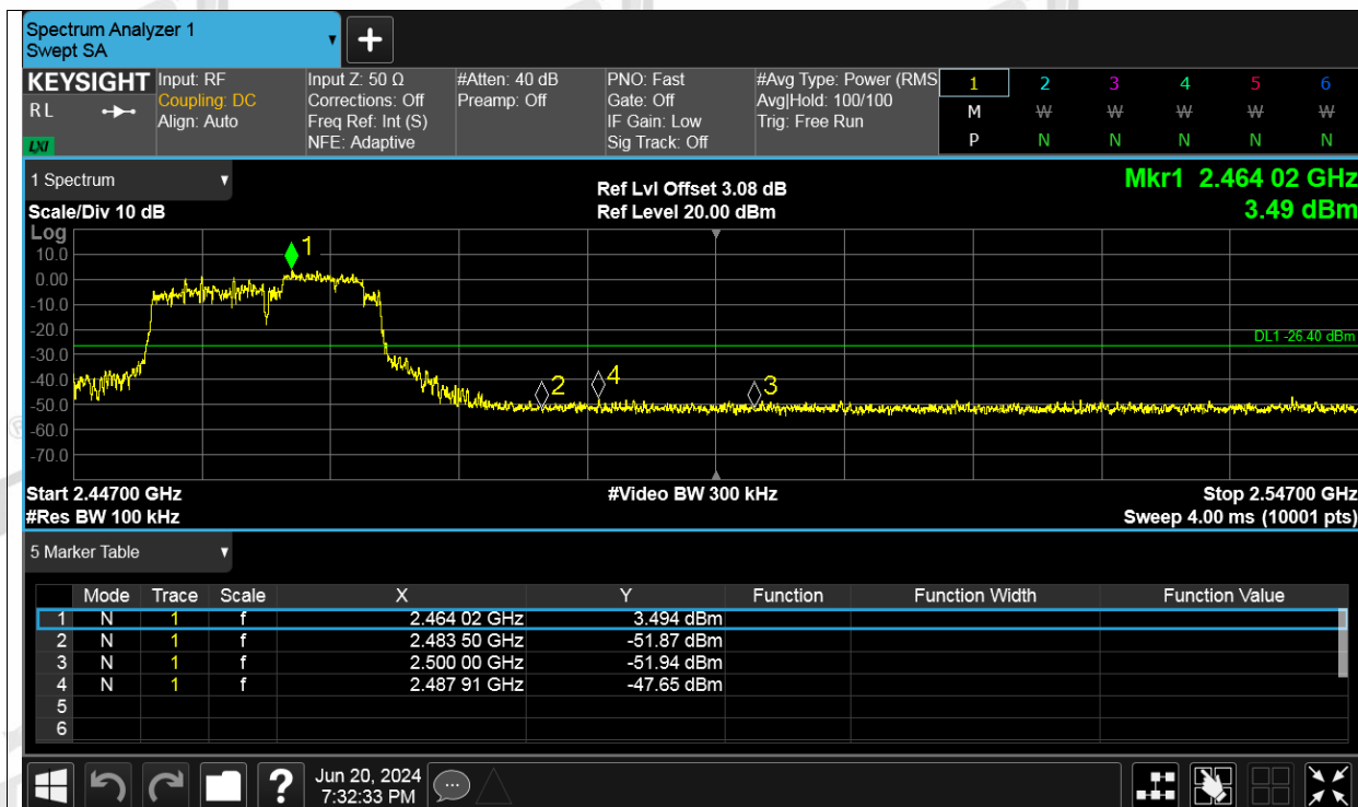
Band Edge NVNT be20 52+26RU Index 39+7 2462MHz Ant2 Ref
