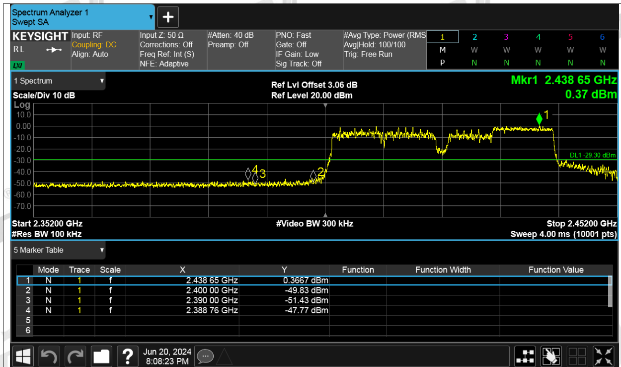
Band Edge NVNT be40 106+26RU Index 56+13 2422MHz Ant2 Ref
