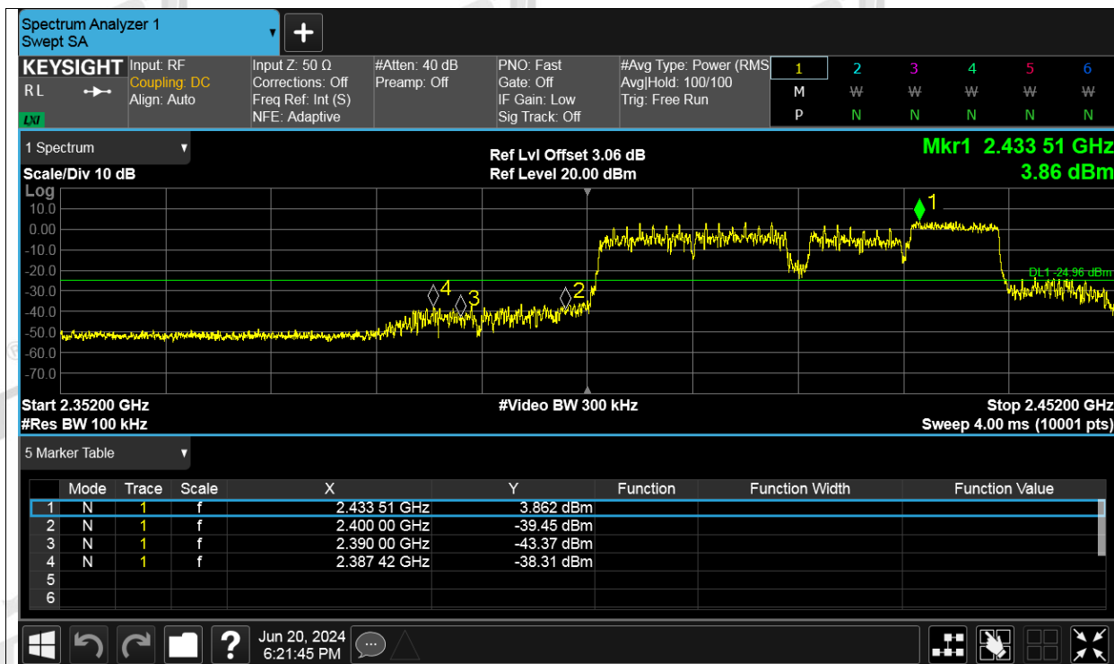
Band Edge NVNT ax40 106RU Index 56 2422MHz Ant2 Ref
