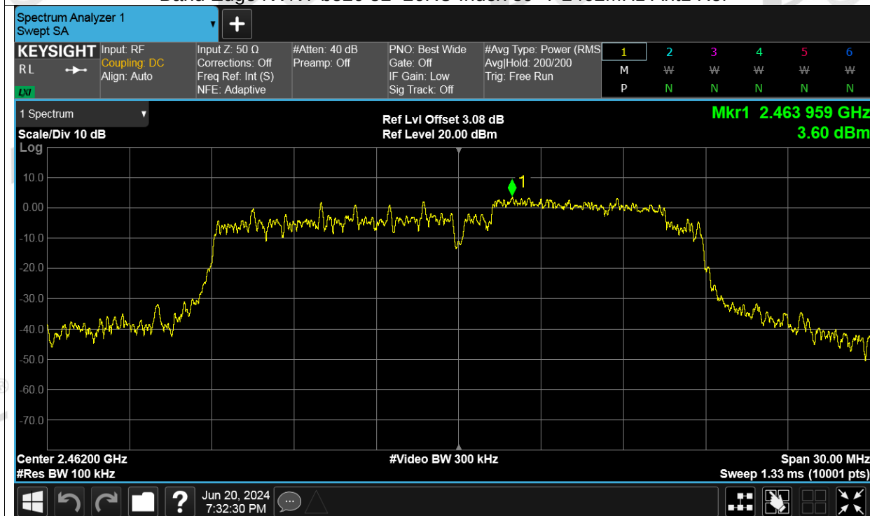
Band Edge NVNT be20 52+26RU Index 39+7 2462MHz Ant1 Emission
