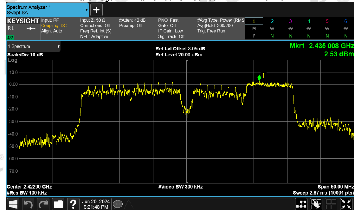
Band Edge NVNT ax40 106RU Index 56 2422MHz Ant2 Emission
