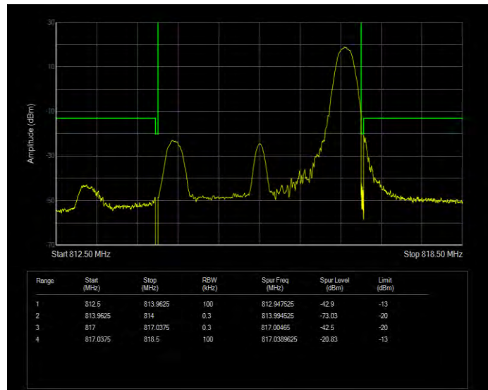
Band26(814-824) 16QAM BW=3MHz Channel=26705 RB Size=1 Position=#0 Normal
