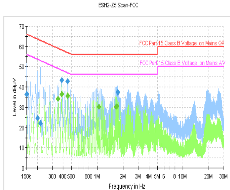
Fig. 32 AC Power line Conducted Emission (Idle, AE2)
