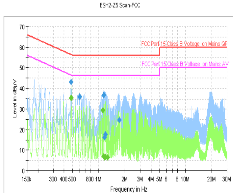
Fig. 34 AC Power line Conducted Emission (Idle, AE3)
