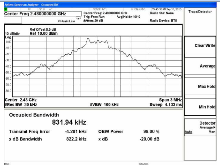
20dB Bandwidth GFSK-High channel
