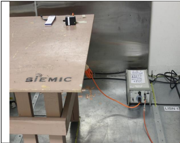
AC conducted emissions – Front View
