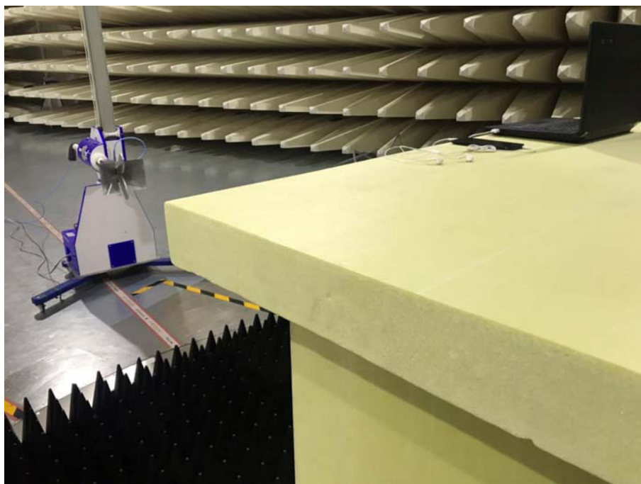
Above 1GHz Radiated Emissions Test Setup (with laptop)
