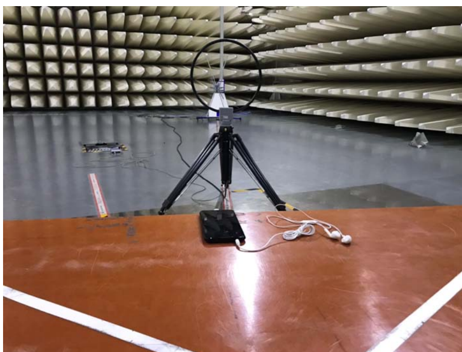
Radiated Emissions Test Setup below 30MHz
