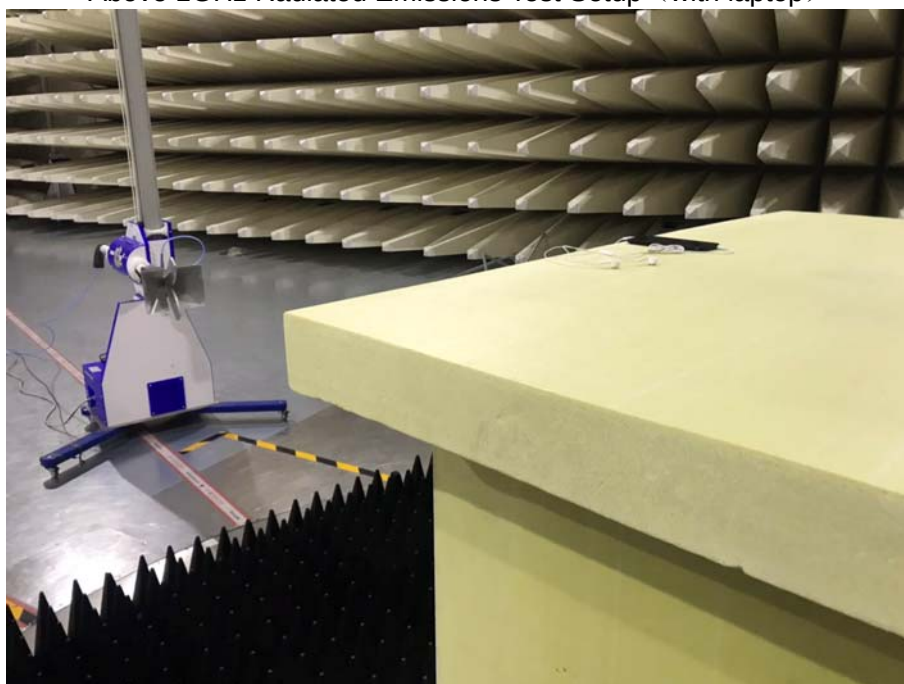
Above 1GHz Radiated Emissions Test Setup (with charger)
