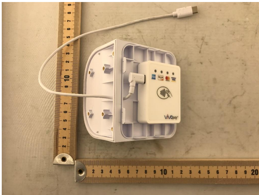
Photograph 8: Front View of DUT With Front Cover Off
