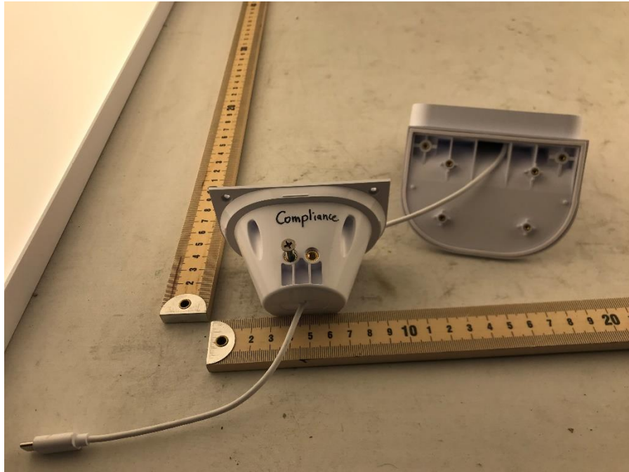
Photograph 7: Bottom View of DUT With Bottom Cover Off
