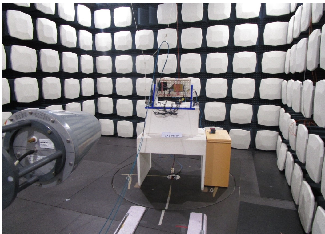
Figure 2: EUT setup in fully anechoic room (overall view)
