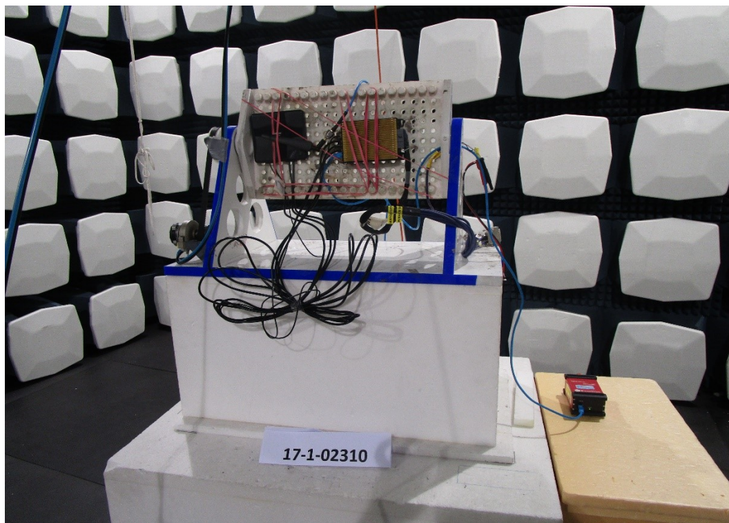
Figure 1: EUT setup in fully anechoic room (close view)
