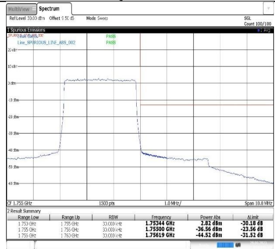
Band4-3MHz-QPSK-20385-15RB#0
