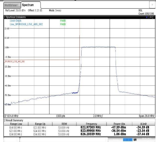
Band5-5MHz-16QAM-20425-25RB#0
