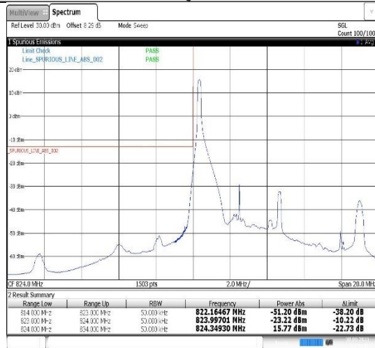
Band5-5MHz-16QAM-20425-1RB#0
