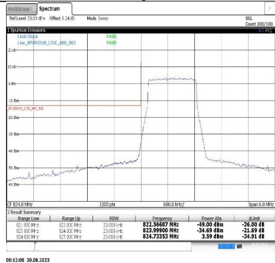
Band5-1.4MHz-16QAM-20643-6RB#0
