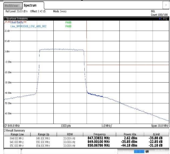
Band5-3MHz-16QAM-20635-15RB#0
