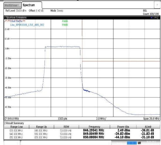
Band5-5MHz-16QAM-20625-25RB#0
