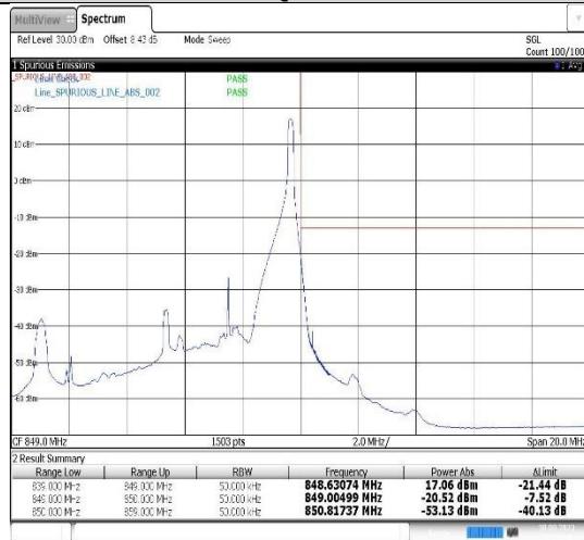
Band5-5MHz-16QAM-20625-1RB#24
