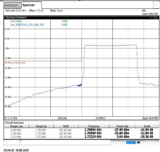
Band4-15MHz-16QAM-20325-75RB#0
