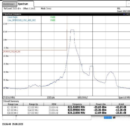
Band5-1.4MHz-QPSK-20643-1RB#5
