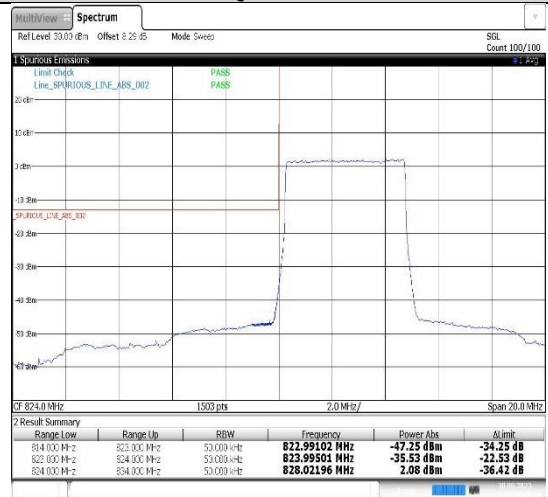
Band5-5MHz-QPSK-20425-25RB#0
