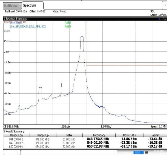
Band5-3MHz-16QAM-20635-1RB#14
