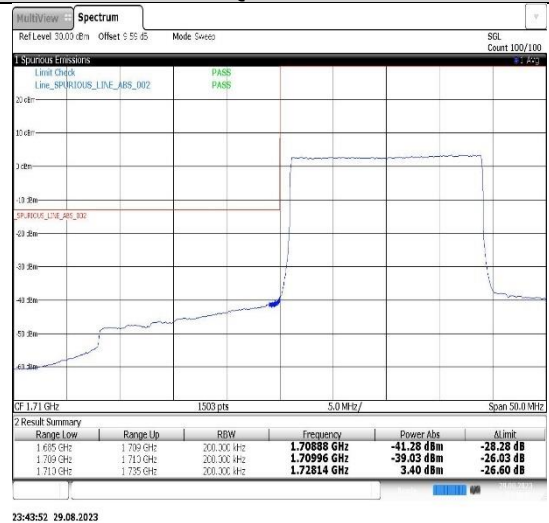
Band4-20MHz-16QAM-20050-100RB#0
