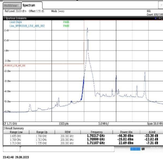
Band4-20MHz-16QAM-20050-1RB#0
