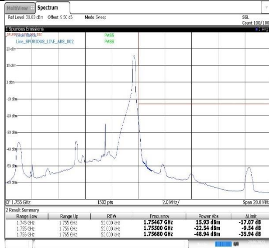
Band4-5MHz-16QAM-20375-1RB#24
