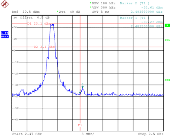
2.4G(ANT 1): Band edge-right side
