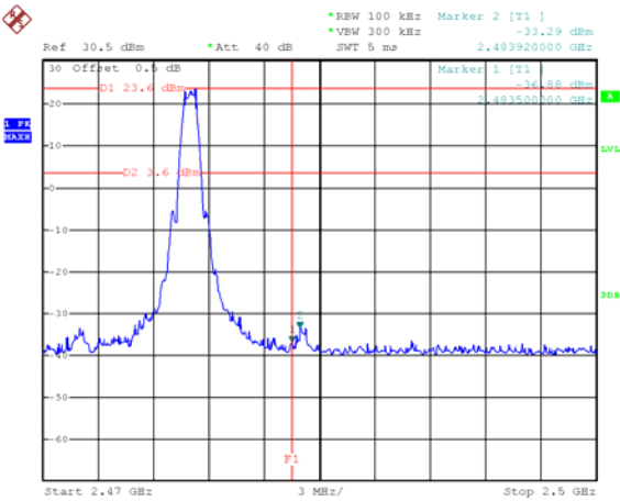
2.4G(ANT 2): Band edge-right side
