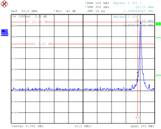
2.4G(ANT 1): Band edge-left side
