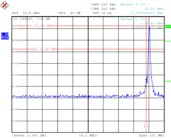
2.4G(ANT 2): Band edge-left side
