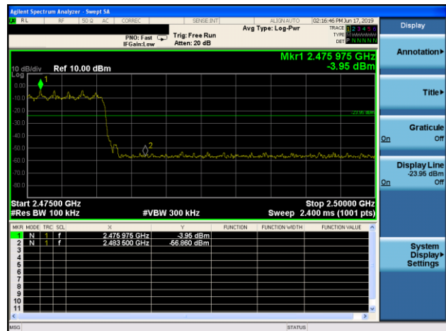
\pi/4 -DQPSK: Band Edge-High Channel
