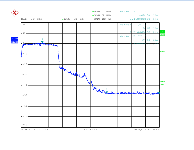
Channel 42 / 5210 MHz – Peak
