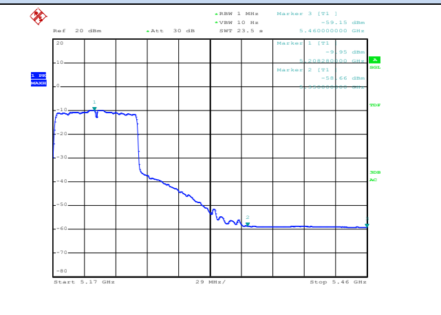
Channel 42 / 5210 MHz – Average
