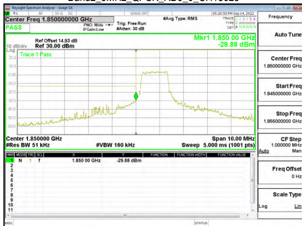
Band2_5MHz_QPSK_RB6_0_CH18625
