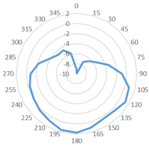
2.44GHz
