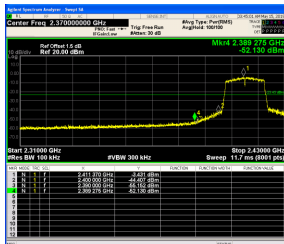
Left bandedge
