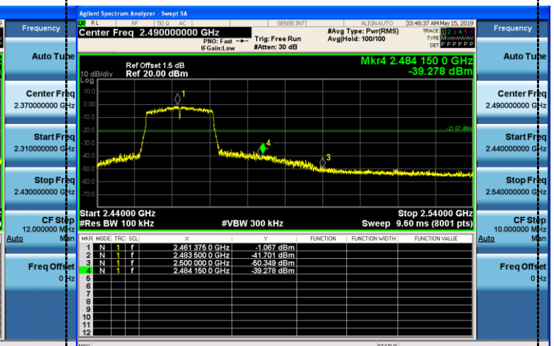
Right bandedge
