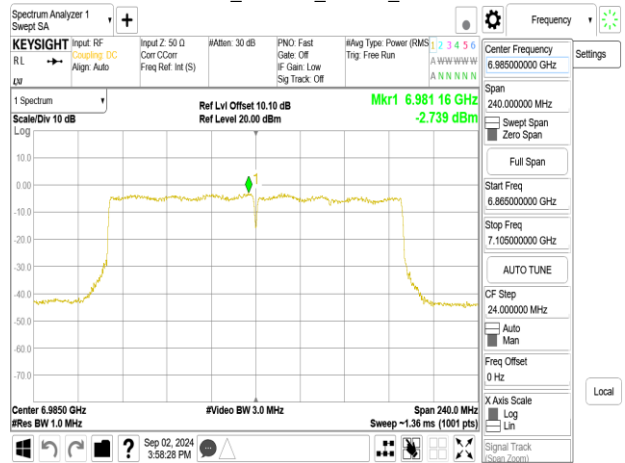
802.11be_160MHz_Chain1_6985MHz_996+484+242_MR2
