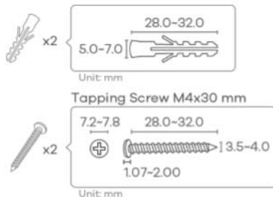
Figure 4 Screw Specifications
