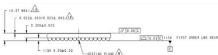
Figure 4-2 QCA9377 package mechanical dimensions height and seating plane
