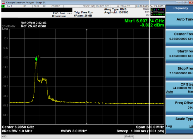
Plot 7-505. LPI Power Spectral Density Plot SDM Antenna WF8 (160MHz 802.11ax RU26 (UNII Band 8) – Ch. 207)
