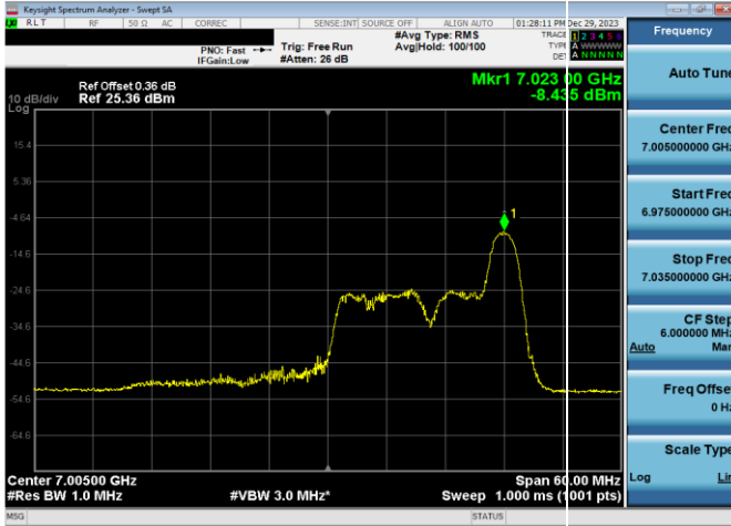
Plot 7-493. LPI Power Spectral Density Plot SDM Antenna WF8 (40MHz 802.11ax RU26 (UNII Band 8) – Ch. 211)
