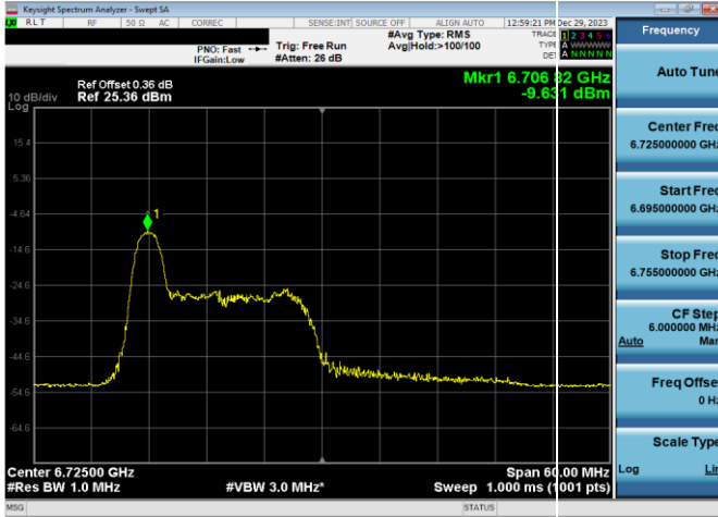
Plot 7-457. LPI Power Spectral Density Plot SDM Antenna WF8 (40MHz 802.11ax RU26 (UNII Band 7) – Ch. 155)
