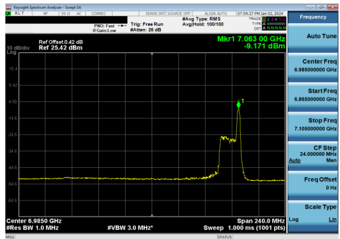
Plot 7-510. LPI Power Spectral Density Plot SDM Antenna WF7a (160MHz 802.11ax RU26 (UNII Band 8) – Ch. 207)
