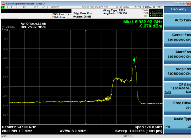
Plot 7-501. LPI Power Spectral Density Plot SDM Antenna WF8 (80MHz 802.11ax RU26 (UNII Band 8) – Ch. 199)
