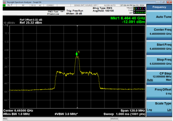
Plot 7-436. LPI Power Spectral Density Plot SDM Antenna WF7a (80MHz 802.11ax RU26 (UNII Band 6) – Ch. 103)
