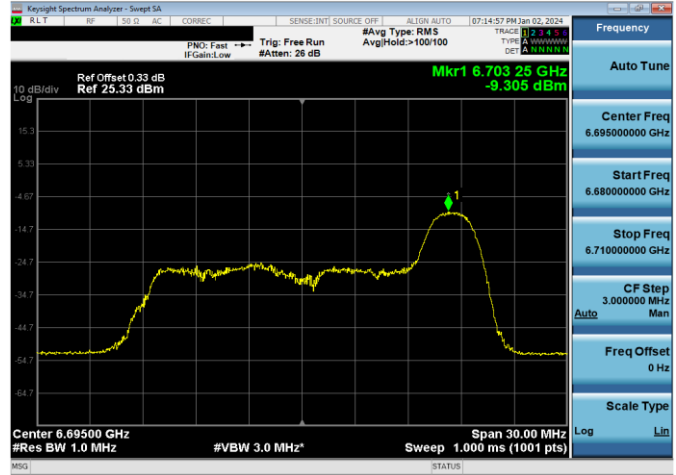
Plot 7-454. LPI Power Spectral Density Plot SDM Antenna WF7a (20MHz 802.11ax RU26 (UNII Band 7) – Ch. 149)
