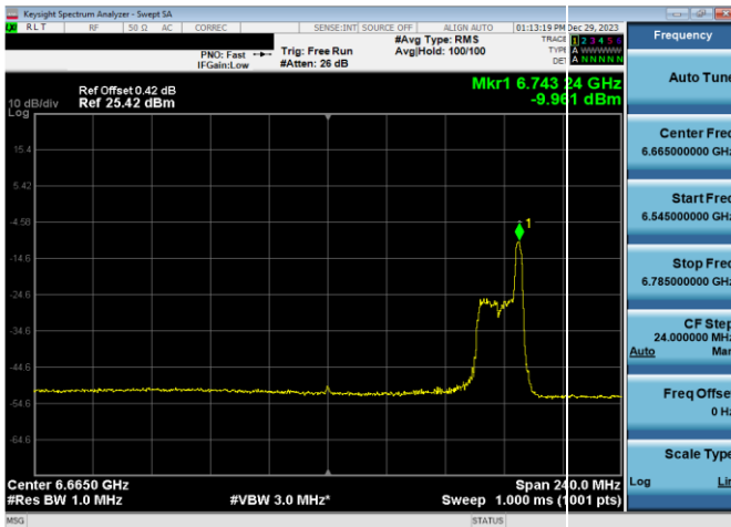
Plot 7-477. LPI Power Spectral Density Plot SDM Antenna WF8 (160MHz 802.11ax RU26 (UNII Band 7) – Ch. 143)
