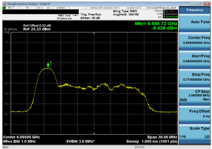
Plot 7-450. LPI Power Spectral Density Plot SDM Antenna WF7a (20MHz 802.11ax RU26 (UNII Band 7) – Ch. 149)
