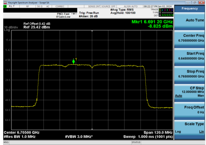
Plot 7-472. LPI Power Spectral Density Plot SDM Antenna WF7a (80MHz 802.11ax RU996 (UNII Band 7) – Ch. 151)
