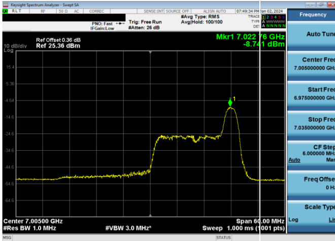
Plot 7-494. LPI Power Spectral Density Plot SDM Antenna WF7a (40MHz 802.11ax RU26 (UNII Band 8) – Ch. 211)
