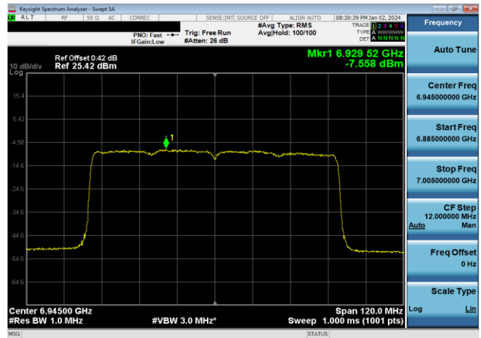
Plot 7-504. LPI Power Spectral Density Plot SDM Antenna WF7a (80MHz 802.11ax RU996 (UNII Band 8) – Ch. 199)
