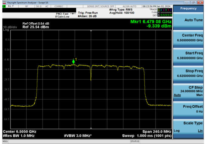
Plot 7-448. LPI Power Spectral Density Plot SDM Antenna WF7a (160MHz 802.11ax RU996x2 (UNII Band 6) – Ch. 111)
