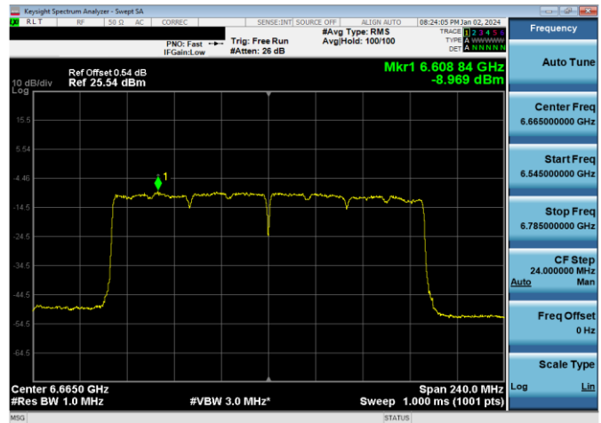
Plot 7-480. LPI Power Spectral Density Plot SDM Antenna WF7a (160MHz 802.11ax RU996x2 (UNII Band 7) – Ch. 143)
