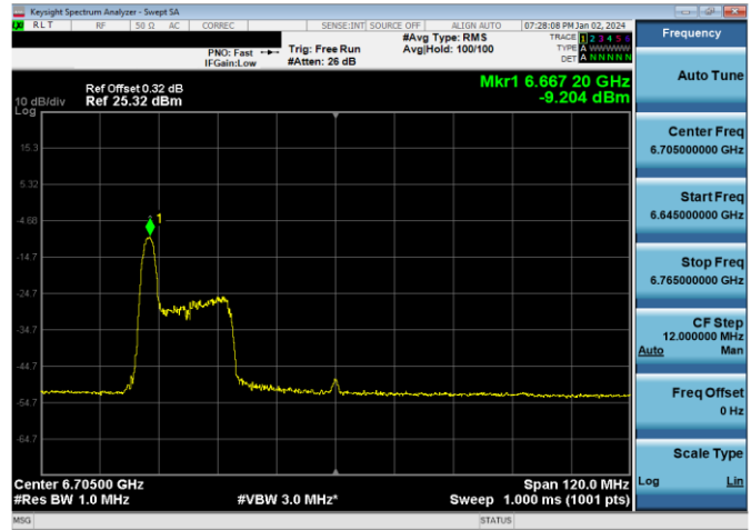
Plot 7-466. LPI Power Spectral Density Plot SDM Antenna WF7a (80MHz 802.11ax RU26 (UNII Band 7) – Ch. 151)
