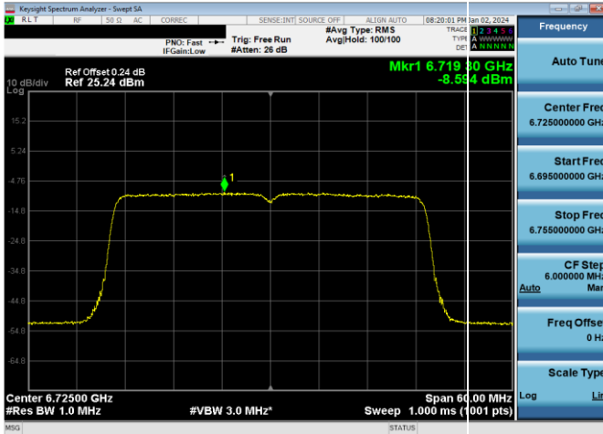
Plot 7-464. LPI Power Spectral Density Plot SDM Antenna WF7a (40MHz 802.11ax RU484 (UNII Band 7) – Ch. 155)
