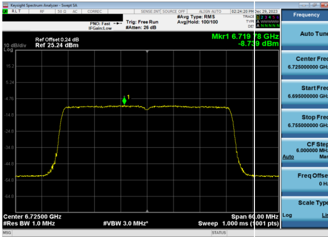
Plot 7-463. LPI Power Spectral Density Plot SDM Antenna WF8 (40MHz 802.11ax RU484 (UNII Band 7) – Ch. 155)
