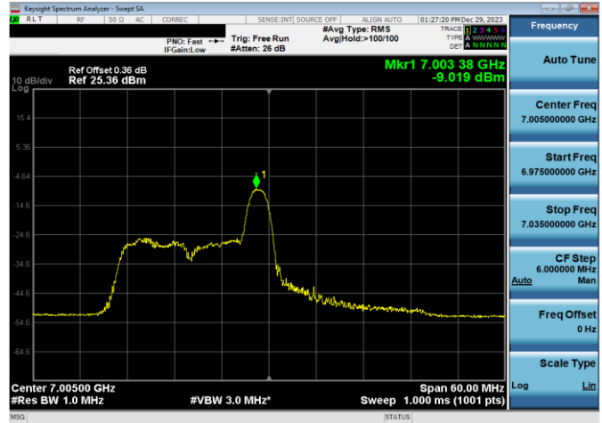
Plot 7-491. LPI Power Spectral Density Plot SDM Antenna WF8 (40MHz 802.11ax RU26 (UNII Band 8) – Ch. 211)
