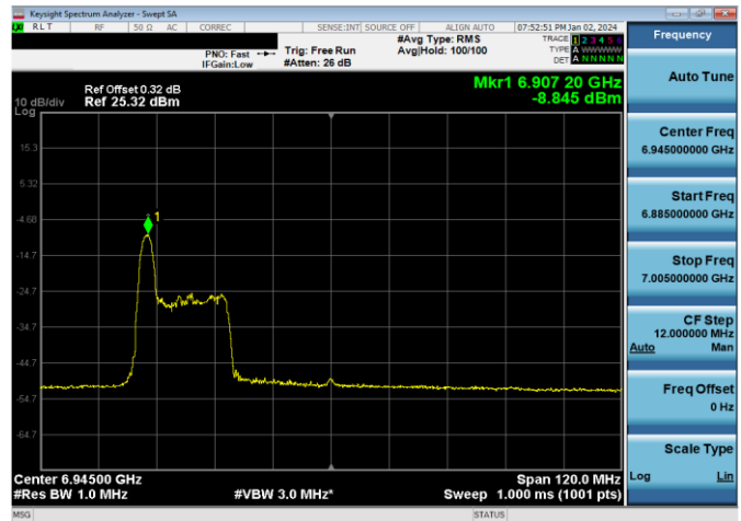
Plot 7-498. LPI Power Spectral Density Plot SDM Antenna WF7a (80MHz 802.11ax RU26 (UNII Band 8) – Ch. 199)
