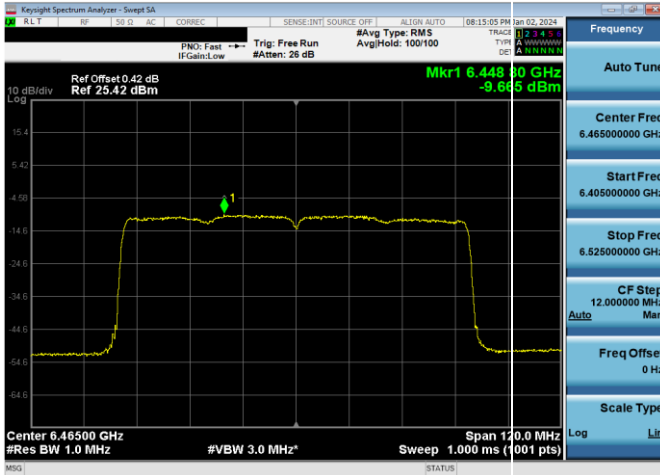
Plot 7-440. LPI Power Spectral Density Plot SDM Antenna WF7a (80MHz 802.11ax RU996 (UNII Band 6) – Ch. 103)
