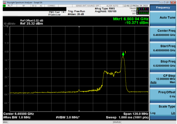
Plot 7-437. LPI Power Spectral Density Plot SDM Antenna WF8 (80MHz 802.11ax RU26 (UNII Band 6) – Ch. 103)
