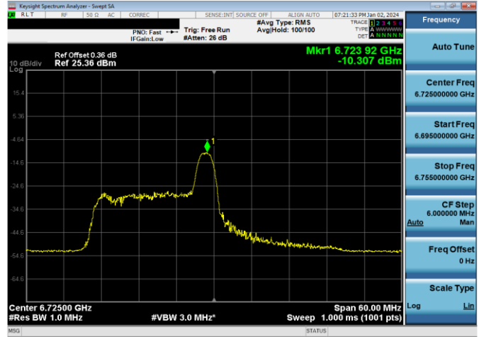
Plot 7-460. LPI Power Spectral Density Plot SDM Antenna WF7a (40MHz 802.11ax RU26 (UNII Band 7) – Ch. 155)
