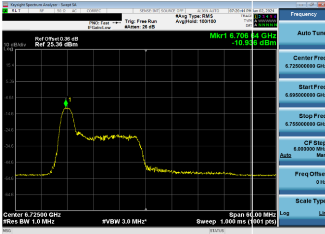
Plot 7-458. LPI Power Spectral Density Plot SDM Antenna WF7a (40MHz 802.11ax RU26 (UNII Band 7) – Ch. 155)
