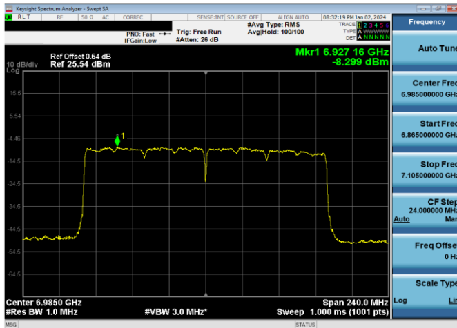
Plot 7-512. LPI Power Spectral Density Plot SDM Antenna WF7a (160MHz 802.11ax RU996x2 (UNII Band 8) – Ch. 207)
