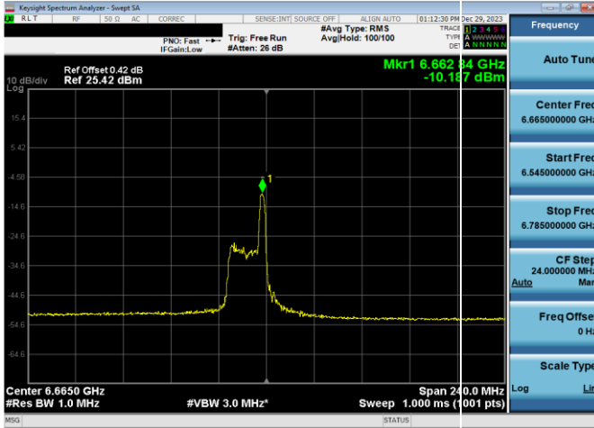
Plot 7-475. LPI Power Spectral Density Plot SDM Antenna WF8 (160MHz 802.11ax RU26 (UNII Band 7) – Ch. 143)
