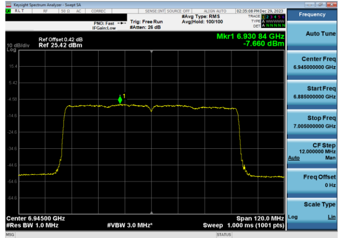
Plot 7-503. LPI Power Spectral Density Plot SDM Antenna WF8 (80MHz 802.11ax RU996 (UNII Band 8) – Ch. 199)
