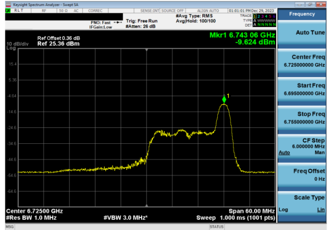
Plot 7-461. LPI Power Spectral Density Plot SDM Antenna WF8 (40MHz 802.11ax RU26 (UNII Band 7) – Ch. 155)
