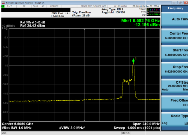
Plot 7-446. LPI Power Spectral Density Plot SDM Antenna WF7a (160MHz 802.11ax RU26 (UNII Band 6) – Ch. 111)
