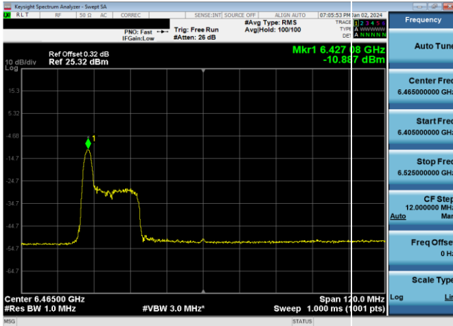
Plot 7-434. LPI Power Spectral Density Plot SDM Antenna WF7a (80MHz 802.11ax RU26 (UNII Band 6) – Ch. 103)
