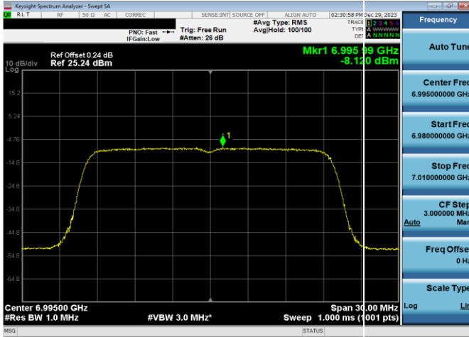
Plot 7-487. LPI Power Spectral Density Plot SDM Antenna WF8 (20MHz 802.11ax RU242 (UNII Band 8) – Ch. 209)
