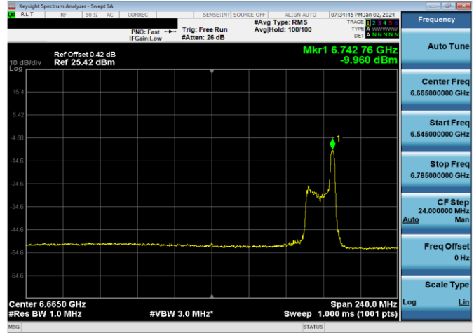
Plot 7-478. LPI Power Spectral Density Plot SDM Antenna WF7a (160MHz 802.11ax RU26 (UNII Band 7) – Ch. 143)
