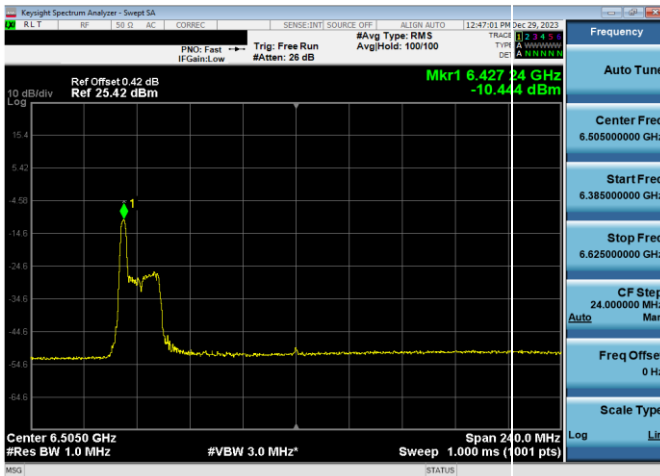
Plot 7-441. LPI Power Spectral Density Plot SDM Antenna WF8 (160MHz 802.11ax RU26 (UNII Band 6) – Ch. 111)
