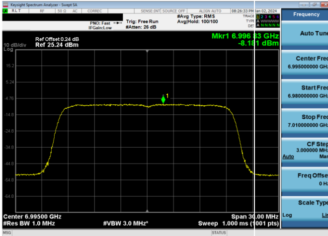
Plot 7-488. LPI Power Spectral Density Plot SDM Antenna WF7a (20MHz 802.11ax RU242 (UNII Band 8) – Ch. 209)
