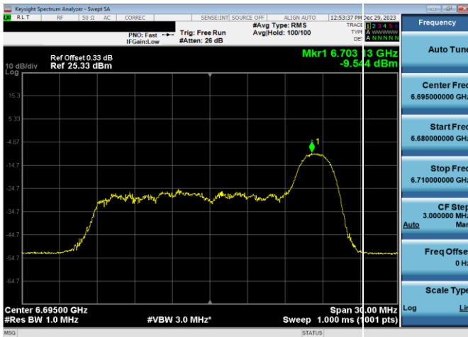
Plot 7-453. LPI Power Spectral Density Plot SDM Antenna WF8 (20MHz 802.11ax RU26 (UNII Band 7) – Ch. 149)
