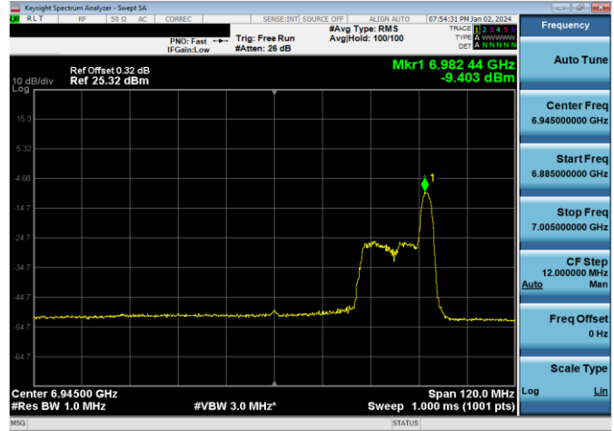
Plot 7-502. LPI Power Spectral Density Plot SDM Antenna WF7a (80MHz 802.11ax RU26 (UNII Band 8) – Ch. 199)
