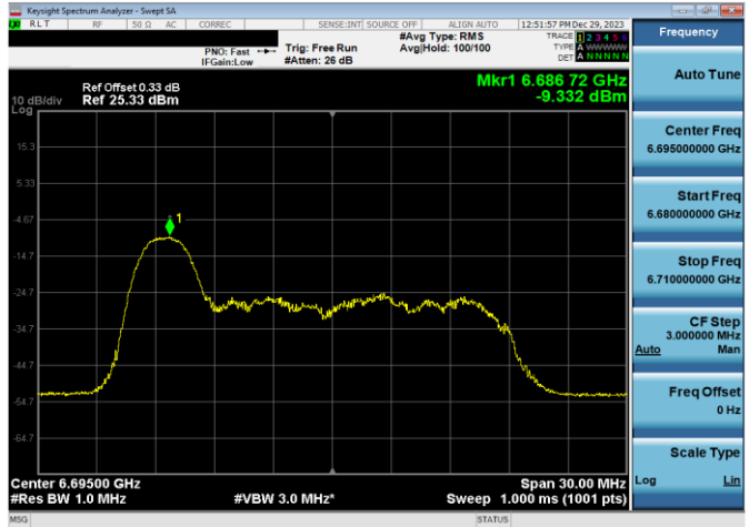
Plot 7-449. LPI Power Spectral Density Plot SDM Antenna WF8 (20MHz 802.11ax RU26 (UNII Band 7) – Ch. 149)
