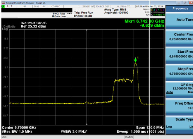
Plot 7-470. LPI Power Spectral Density Plot SDM Antenna WF7a (80MHz 802.11ax RU26 (UNII Band 7) – Ch. 151)
