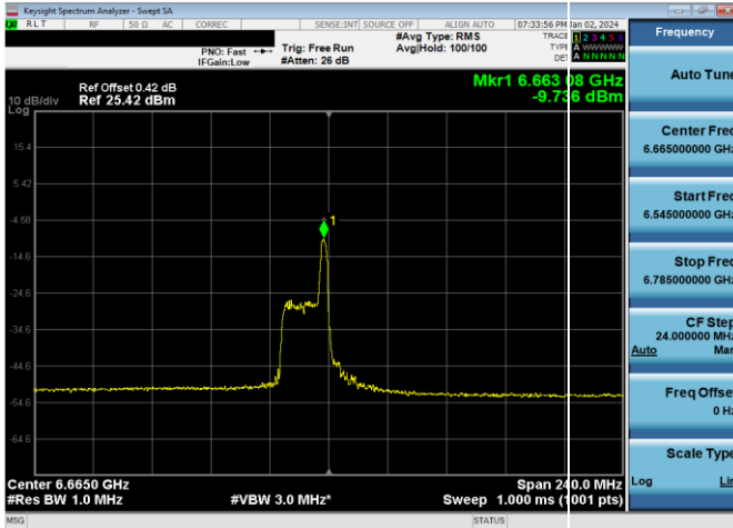
Plot 7-476. LPI Power Spectral Density Plot SDM Antenna WF7a (160MHz 802.11ax RU26 (UNII Band 7) – Ch. 143)
