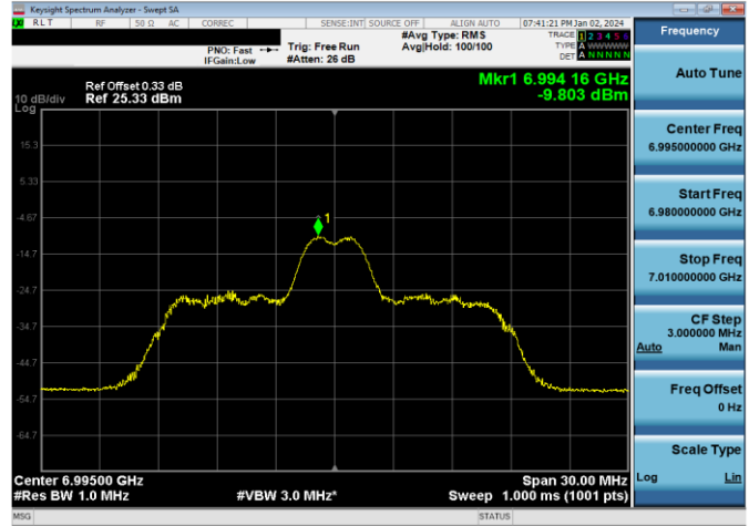
Plot 7-484. LPI Power Spectral Density Plot SDM Antenna WF7a (20MHz 802.11ax RU26 (UNII Band 8) – Ch. 209)
