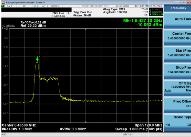
Plot 7-433. LPI Power Spectral Density Plot SDM Antenna WF8 (80MHz 802.11ax RU26 (UNII Band 6) – Ch. 103)
