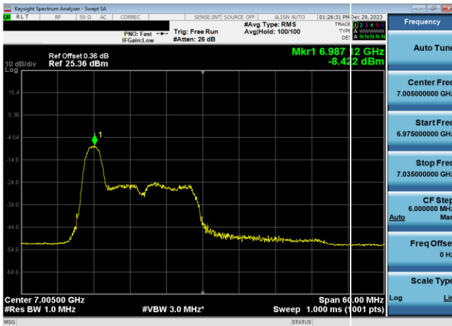
Plot 7-489. LPI Power Spectral Density Plot SDM Antenna WF8 (40MHz 802.11ax RU26 (UNII Band 8) – Ch. 211)
