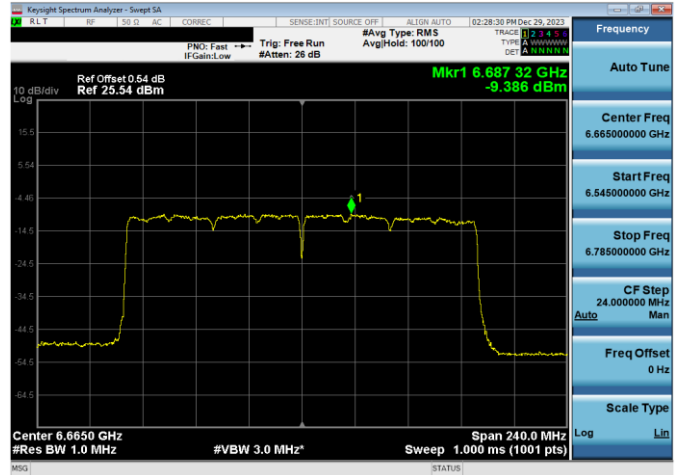
Plot 7-479. LPI Power Spectral Density Plot SDM Antenna WF8 (160MHz 802.11ax RU996x2 (UNII Band 7) – Ch. 143)
