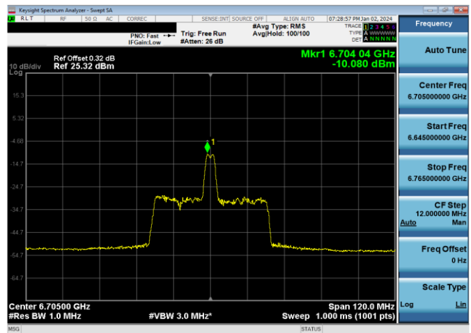
Plot 7-468. LPI Power Spectral Density Plot SDM Antenna WF7a (80MHz 802.11ax RU26 (UNII Band 7) – Ch. 151)
