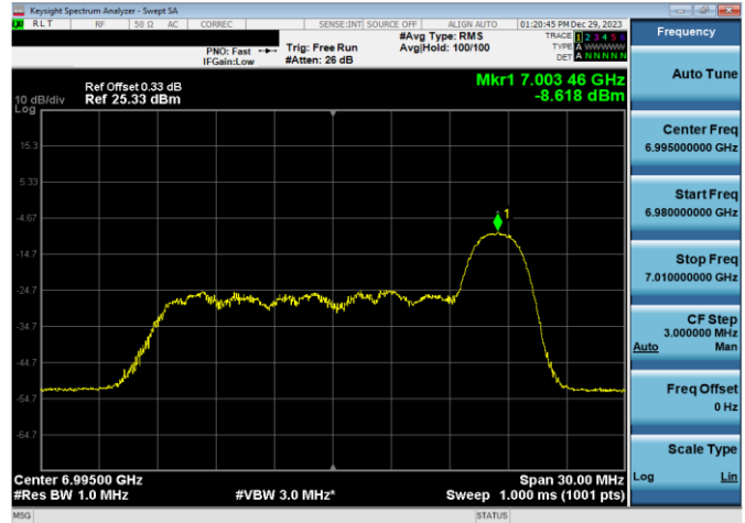
Plot 7-485. LPI Power Spectral Density Plot SDM Antenna WF8 (20MHz 802.11ax RU26 (UNII Band 8) – Ch. 209)
