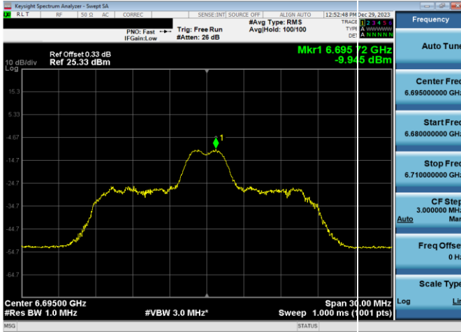
Plot 7-451. LPI Power Spectral Density Plot SDM Antenna WF8 (20MHz 802.11ax RU26 (UNII Band 7) – Ch. 149)
