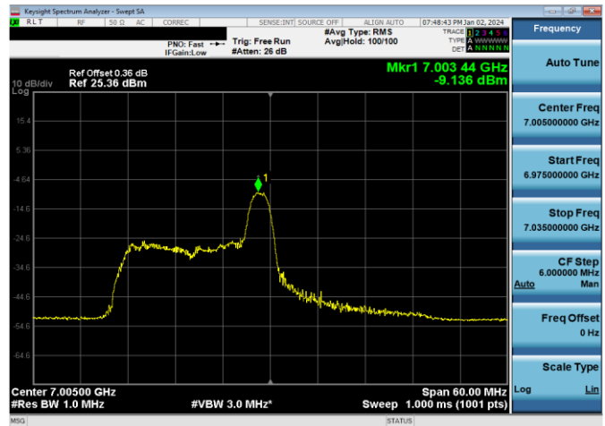
Plot 7-492. LPI Power Spectral Density Plot SDM Antenna WF7a (40MHz 802.11ax RU26 (UNII Band 8) – Ch. 211)
