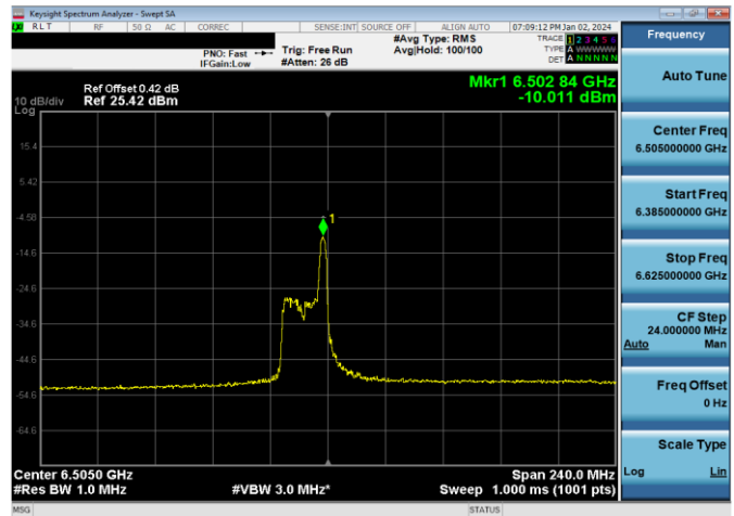
Plot 7-444. LPI Power Spectral Density Plot SDM Antenna WF7a (160MHz 802.11ax RU26 (UNII Band 6) – Ch. 111)
