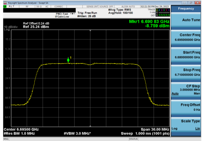
Plot 7-455. LPI Power Spectral Density Plot SDM Antenna WF8 (20MHz 802.11ax RU242 (UNII Band 7) – Ch. 149)
