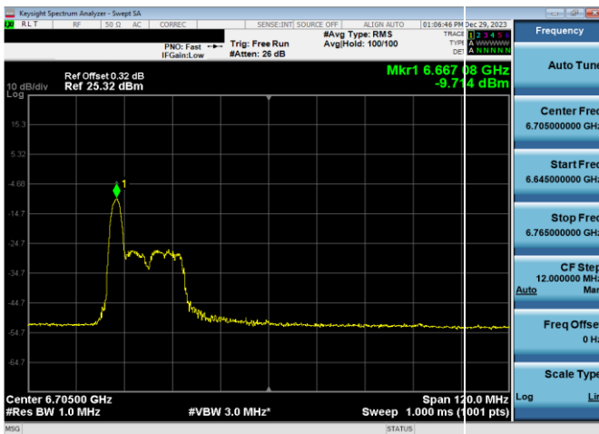
Plot 7-465. LPI Power Spectral Density Plot SDM Antenna WF8 (80MHz 802.11ax RU26 (UNII Band 7) – Ch. 151)
