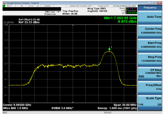
Plot 7-486. LPI Power Spectral Density Plot SDM Antenna WF7a (20MHz 802.11ax RU26 (UNII Band 8) – Ch. 209)
