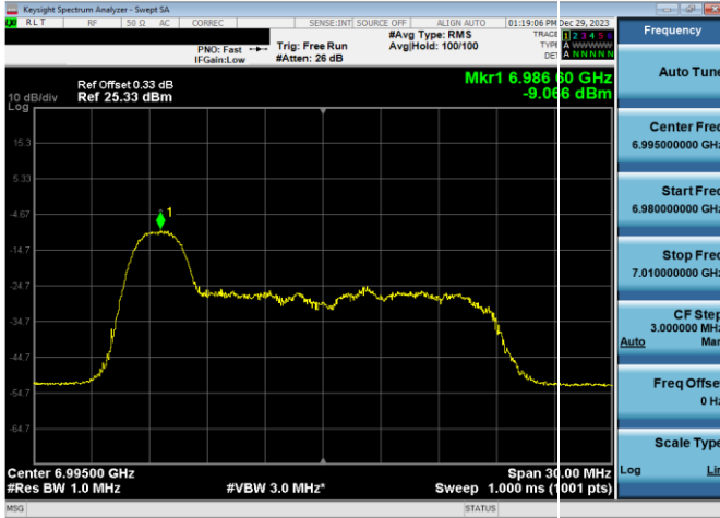
Plot 7-481. LPI Power Spectral Density Plot SDM Antenna WF8 (20MHz 802.11ax RU26 (UNII Band 8) – Ch. 209)
