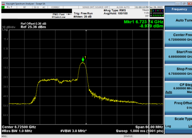
Plot 7-459. LPI Power Spectral Density Plot SDM Antenna WF8 (40MHz 802.11ax RU26 (UNII Band 7) – Ch. 155)
