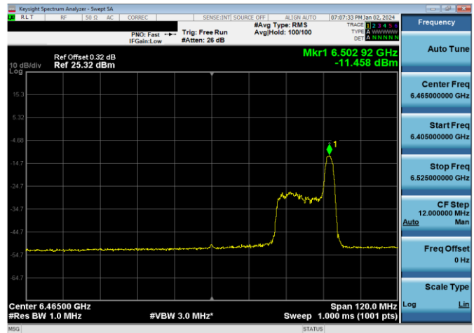
Plot 7-438. LPI Power Spectral Density Plot SDM Antenna WF7a (80MHz 802.11ax RU26 (UNII Band 6) – Ch. 103)
