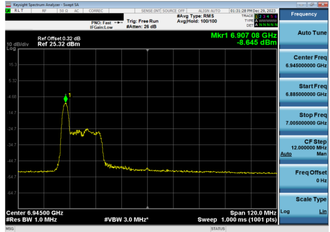
Plot 7-497. LPI Power Spectral Density Plot SDM Antenna WF8 (80MHz 802.11ax RU26 (UNII Band 8) – Ch. 199)
