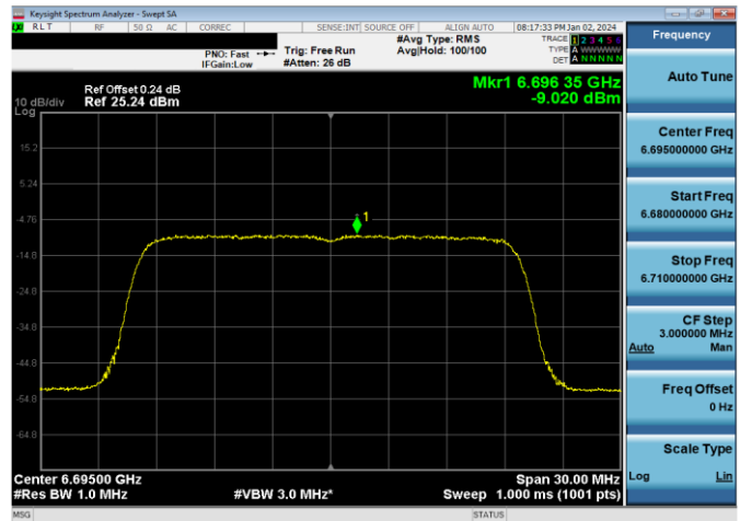
Plot 7-456. LPI Power Spectral Density Plot SDM Antenna WF7a (20MHz 802.11ax RU242 (UNII Band 7) – Ch. 149)
