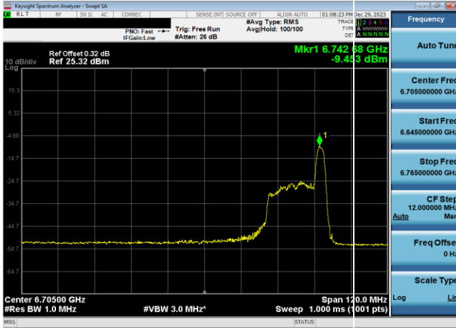
Plot 7-469. LPI Power Spectral Density Plot SDM Antenna WF8 (80MHz 802.11ax RU26 (UNII Band 7) – Ch. 151)
