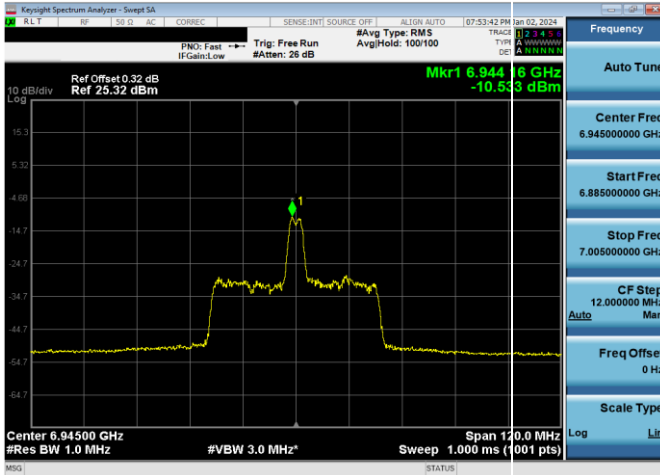
Plot 7-500. LPI Power Spectral Density Plot SDM Antenna WF7a (80MHz 802.11ax RU26 (UNII Band 8) – Ch. 199)
