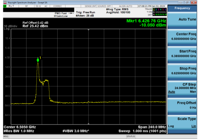
Plot 7-442. LPI Power Spectral Density Plot SDM Antenna WF7a (160MHz 802.11ax RU26 (UNII Band 6) – Ch. 111)
