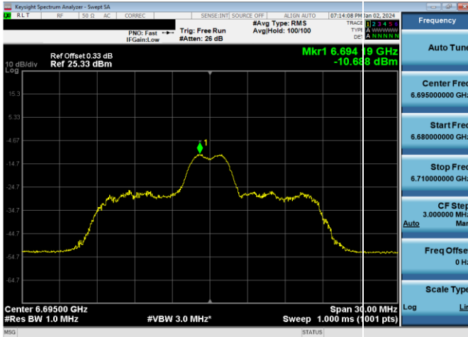
Plot 7-452. LPI Power Spectral Density Plot SDM Antenna WF7a (20MHz 802.11ax RU26 (UNII Band 7) – Ch. 149)
