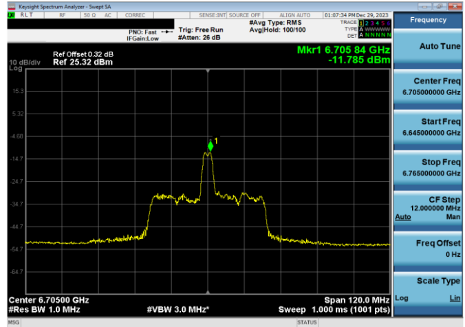
Plot 7-467. LPI Power Spectral Density Plot SDM Antenna WF8 (80MHz 802.11ax RU26 (UNII Band 7) – Ch. 151)
