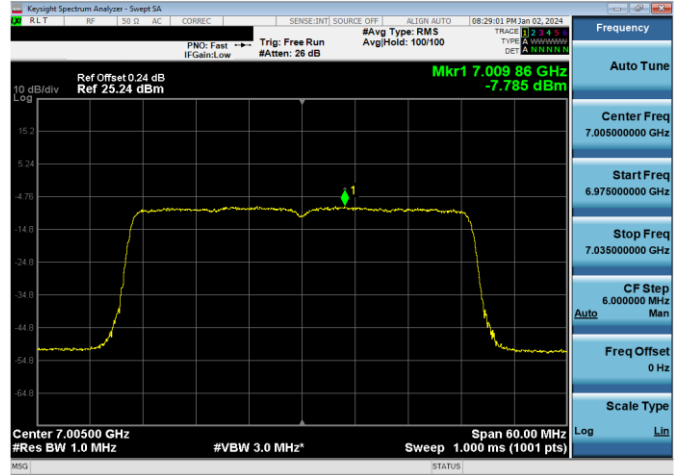
Plot 7-496. LPI Power Spectral Density Plot SDM Antenna WF7a (40MHz 802.11ax RU484 (UNII Band 8) – Ch. 211)
