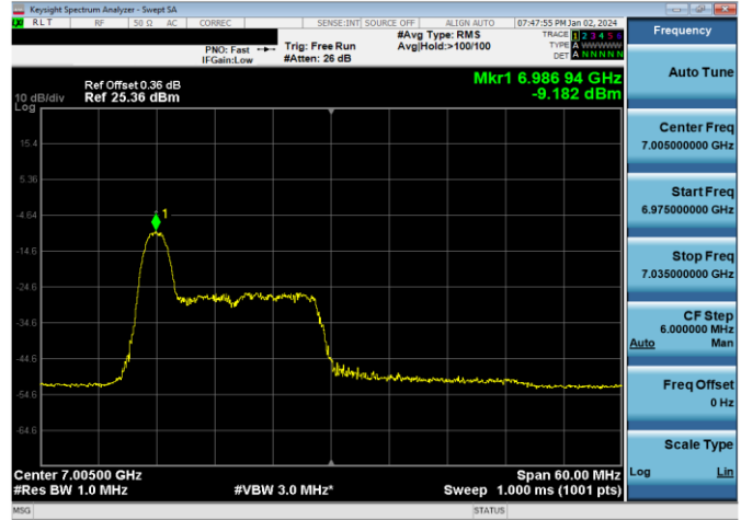
Plot 7-490. LPI Power Spectral Density Plot SDM Antenna WF7a (40MHz 802.11ax RU26 (UNII Band 8) – Ch. 211)
