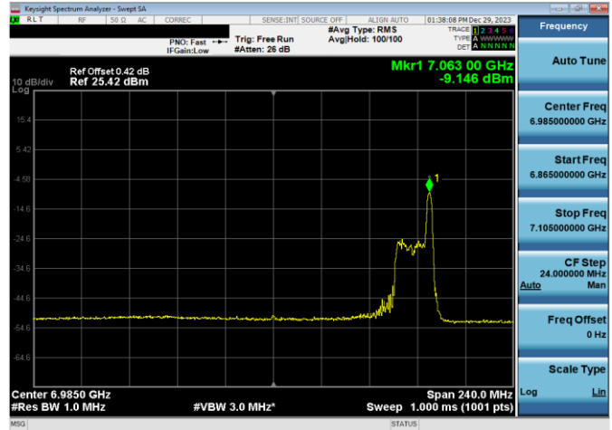
Plot 7-509. LPI Power Spectral Density Plot SDM Antenna WF8 (160MHz 802.11ax RU26 (UNII Band 8) – Ch. 207)
