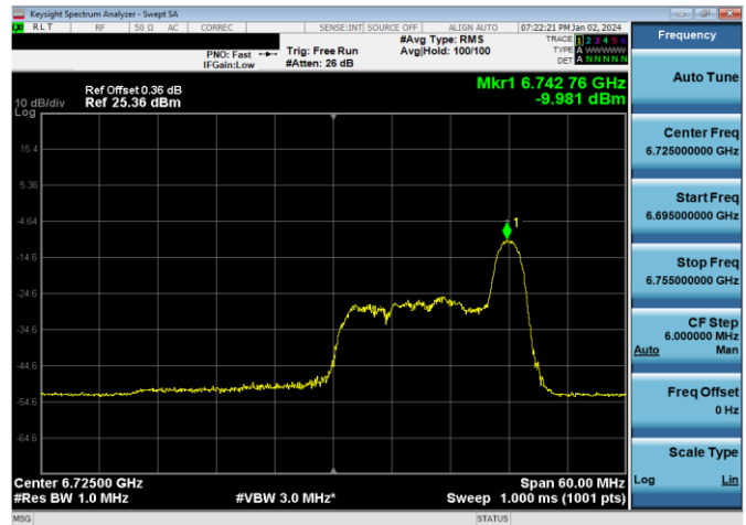
Plot 7-462. LPI Power Spectral Density Plot SDM Antenna WF7a (40MHz 802.11ax RU26 (UNII Band 7) – Ch. 155)
