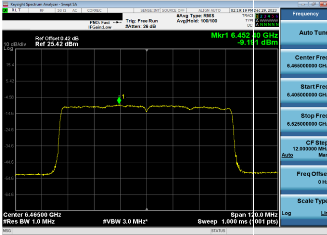
Plot 7-439. LPI Power Spectral Density Plot SDM Antenna WF8 (80MHz 802.11ax RU996 (UNII Band 6) – Ch. 103)
