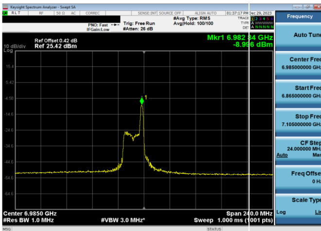
Plot 7-507. LPI Power Spectral Density Plot SDM Antenna WF8 (160MHz 802.11ax RU26 (UNII Band 8) – Ch. 207)
