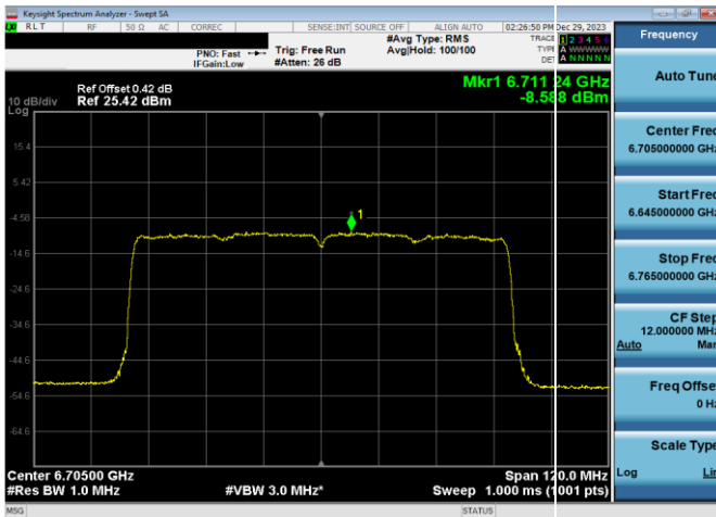
Plot 7-471. LPI Power Spectral Density Plot SDM Antenna WF8 (80MHz 802.11ax RU996 (UNII Band 7) – Ch. 151)
