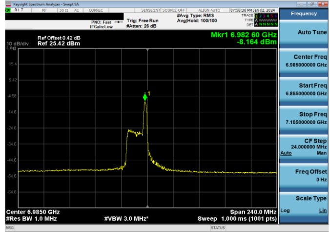
Plot 7-508. LPI Power Spectral Density Plot SDM Antenna WF7a (160MHz 802.11ax RU26 (UNII Band 8) – Ch. 207)
