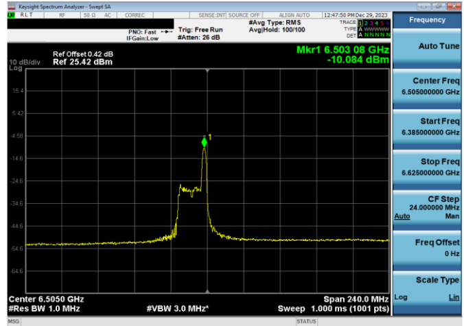
Plot 7-443. LPI Power Spectral Density Plot SDM Antenna WF8 (160MHz 802.11ax RU26 (UNII Band 6) – Ch. 111)
