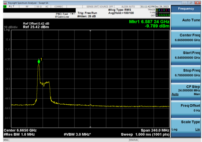
Plot 7-473. LPI Power Spectral Density Plot SDM Antenna WF8 (160MHz 802.11ax RU26 (UNII Band 7) – Ch. 143)
