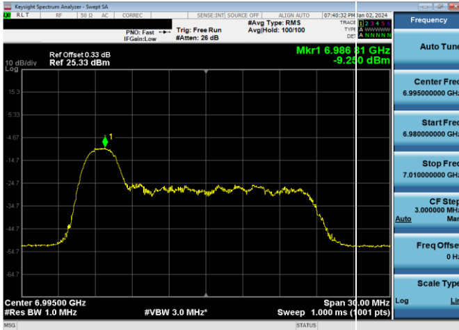
Plot 7-482. LPI Power Spectral Density Plot SDM Antenna WF7a (20MHz 802.11ax RU26 (UNII Band 8) – Ch. 209)
