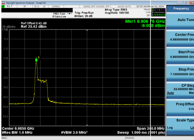
Plot 7-506. LPI Power Spectral Density Plot SDM Antenna WF7a (160MHz 802.11ax RU26 (UNII Band 8) – Ch. 207)
