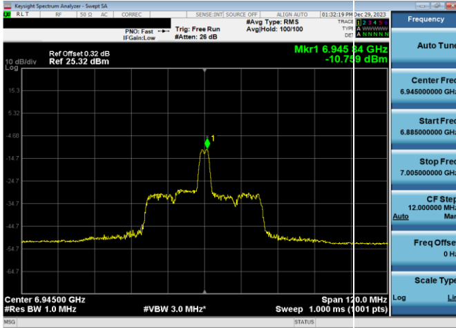
Plot 7-499. LPI Power Spectral Density Plot SDM Antenna WF8 (80MHz 802.11ax RU26 (UNII Band 8) – Ch. 199)
