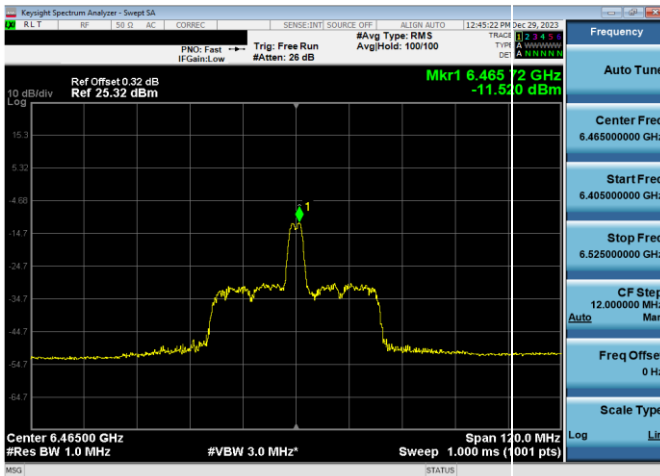
Plot 7-435. LPI Power Spectral Density Plot SDM Antenna WF8 (80MHz 802.11ax RU26 (UNII Band 6) – Ch. 103)
