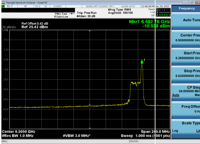
Plot 7-445. LPI Power Spectral Density Plot SDM Antenna WF8 (160MHz 802.11ax RU26 (UNII Band 6) – Ch. 111)
