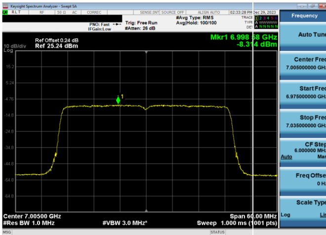
Plot 7-495. LPI Power Spectral Density Plot SDM Antenna WF8 (40MHz 802.11ax RU484 (UNII Band 8) – Ch. 211)
