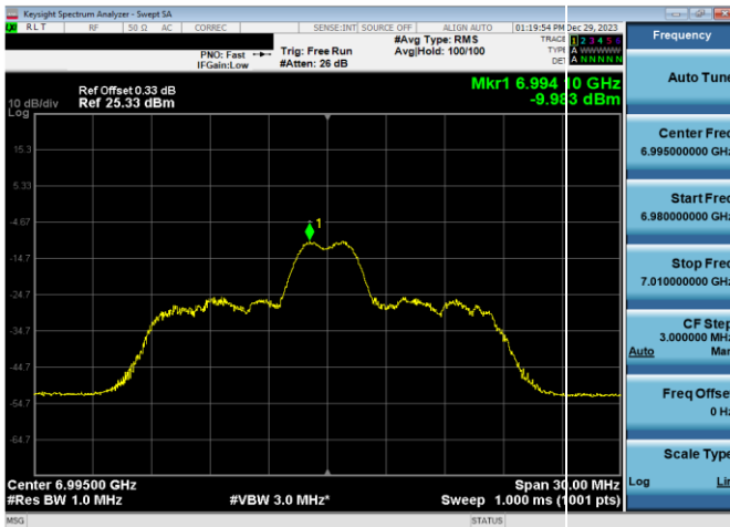
Plot 7-483. LPI Power Spectral Density Plot SDM Antenna WF8 (20MHz 802.11ax RU26 (UNII Band 8) – Ch. 209)
