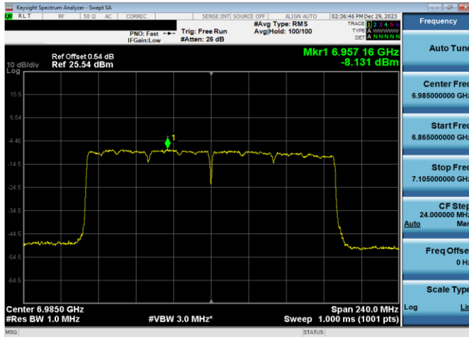
Plot 7-511. LPI Power Spectral Density Plot SDM Antenna WF8 (160MHz 802.11ax RU996x2 (UNII Band 8) – Ch. 207)
