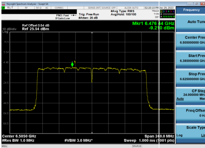
Plot 7-447. LPI Power Spectral Density Plot SDM Antenna WF8 (160MHz 802.11ax RU996x2 (UNII Band 6) – Ch. 111)
