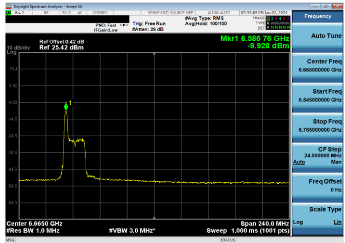
Plot 7-474. LPI Power Spectral Density Plot SDM Antenna WF7a (160MHz 802.11ax RU26 (UNII Band 7) – Ch. 143)
