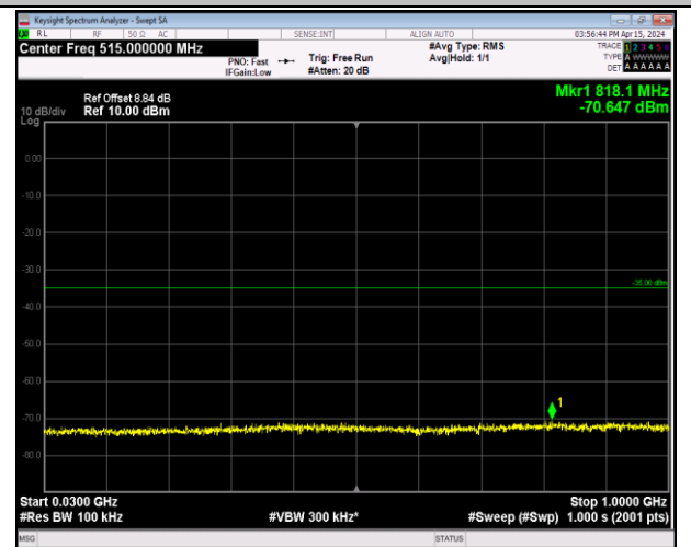
Band7_20MHz_QPSK_21350_1RB#0_30~1000_30~1000
