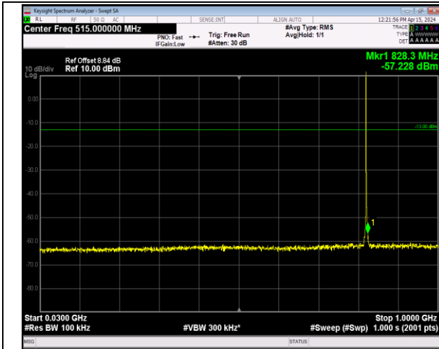
Band5_1.4MHz_64QAM_20407_1RB#0_30~1000_30~1000
