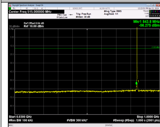
Band5_1.4MHz_16QAM_20643_1RB#0_30~1000_30~10 00
