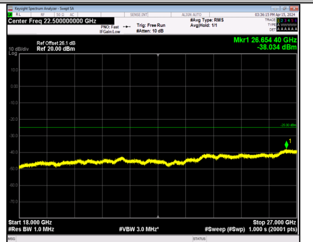
Band7_5MHz_16QAM_21425_1RB#0_18000~27000_18000~27000
