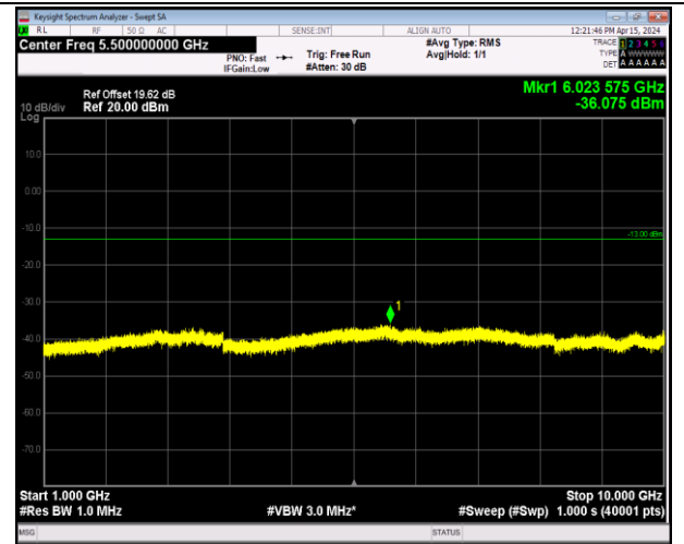
Band5_1.4MHz_16QAM_20407_1RB#0_1000~10000_100 0~10000
