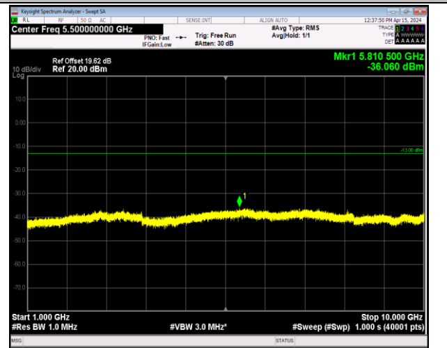
Band5_10MHz_16QAM_20525_1RB#0_1000~10000_100
