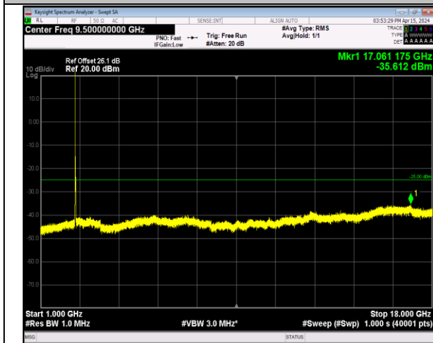
Band7_20MHz_QPSK_20850_1RB#0_1000~18000_1000~18000
