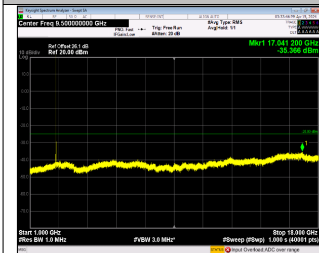
Band7_5MHz_QPSK_21100_1RB#0_1000~18000_1000~18000
