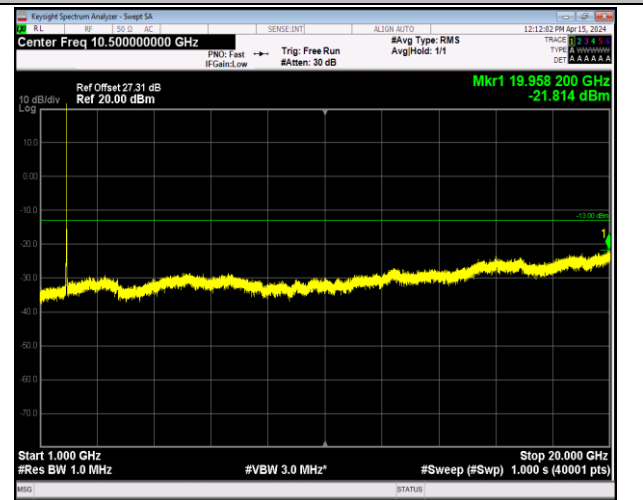
Band2_20MHz_QPSK_18900_1RB#0_1000~20000_1000~20000
