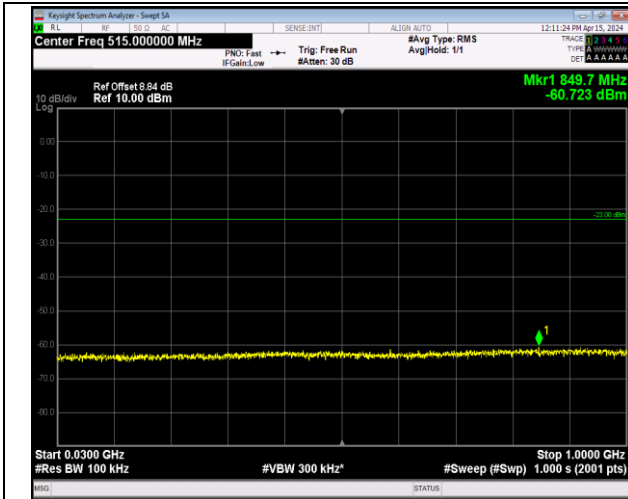
Band2_20MHz_64QAM_18700_1RB#0_30~1000_30~100
