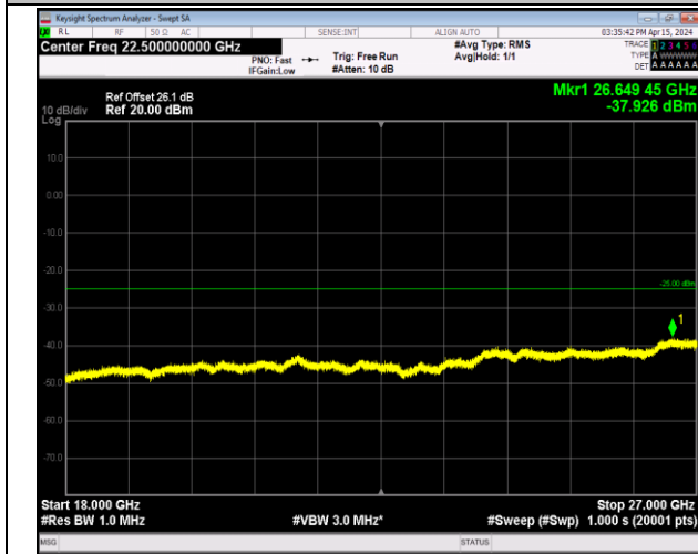
Band7_5MHz_QPSK_21425_1RB#0_18000~27000_18000~27000
