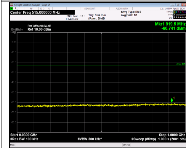
Band2_20MHz_QPSK_18900_1RB#0_30~1000_30~1000
