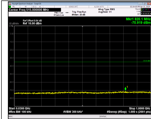
Band7_5MHz_16QAM_21100_1RB#0_30~1000_30~1000
