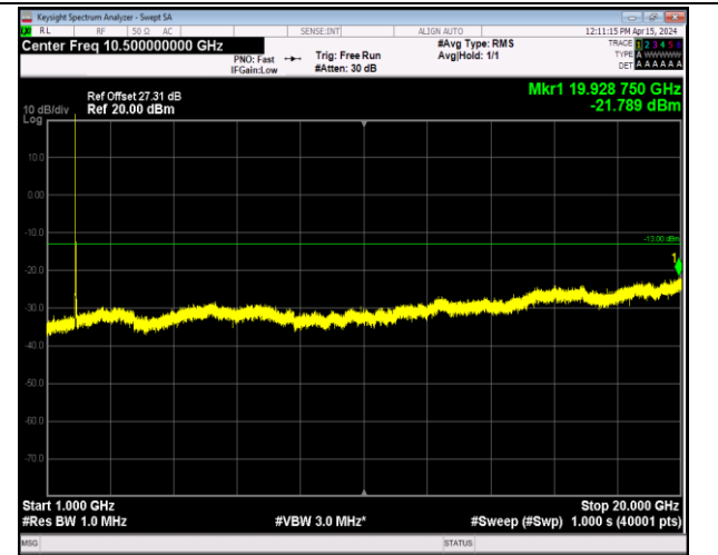
Band2_20MHz_16QAM_18700_1RB#0_1000~20000_100 0~20000
