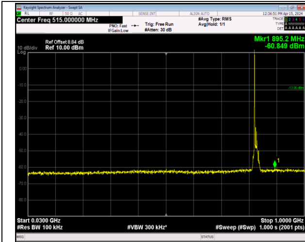
Band5_10MHz_64QAM_20450_1RB#0_30~1000_30~100
