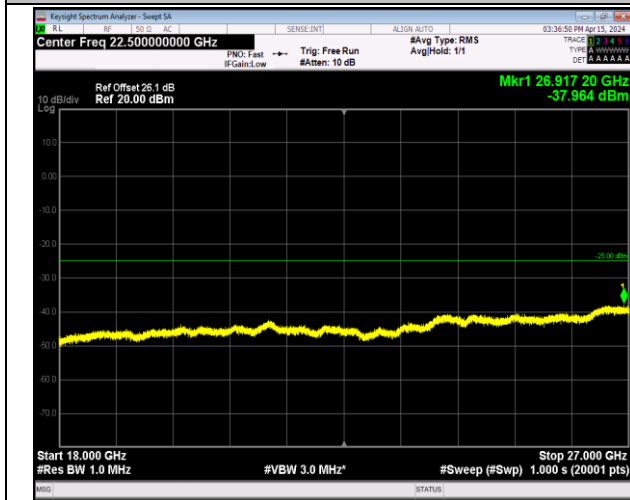
Band7_5MHz_64QAM_21425_1RB#0_18000~27000_18000~27000
