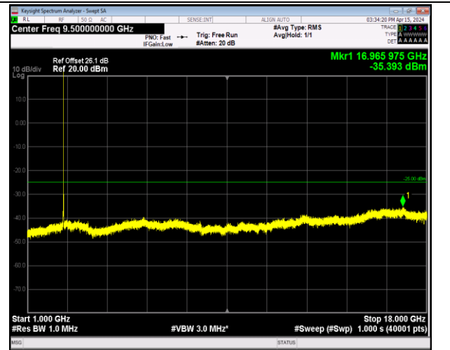
Band7_5MHz_16QAM_21100_1RB#0_1000~18000_1000~18000
