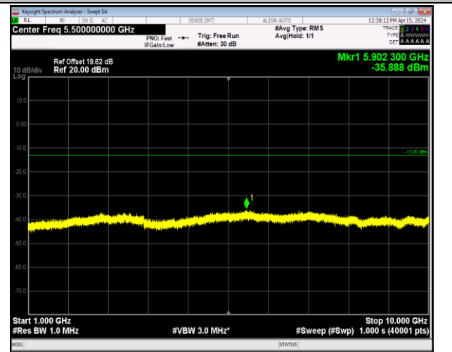
Band5_10MHz_64QAM_20525_1RB#0_1000~10000_100
