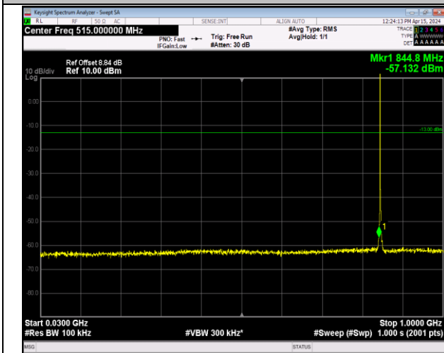
Band5_1.4MHz_64QAM_20643_1RB#0_30~1000_30~1000
