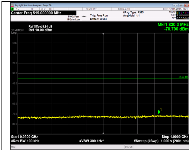
Band7_5MHz_QPSK_20775_1RB#0_30~1000_30~1000
