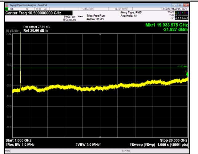
Band2_20MHz_64QAM_18900_1RB#0_1000~20000_100
