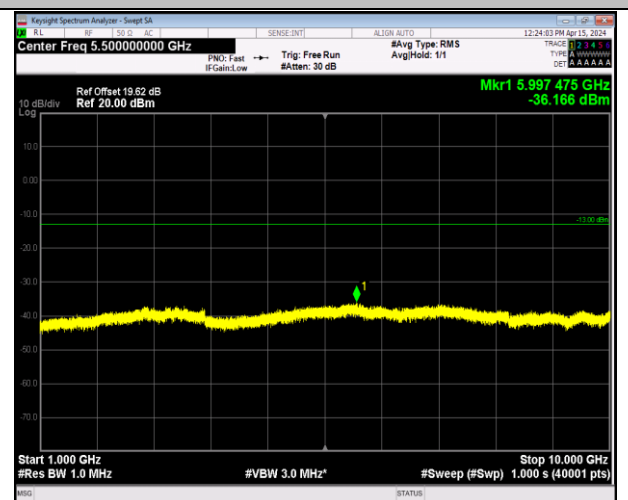
Band5_1.4MHz_16QAM_20643_1RB#0_1000~10000_100 0~10000
