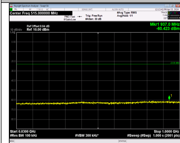
Band2_20MHz_64QAM_19100_1RB#0_30~1000_30~100
