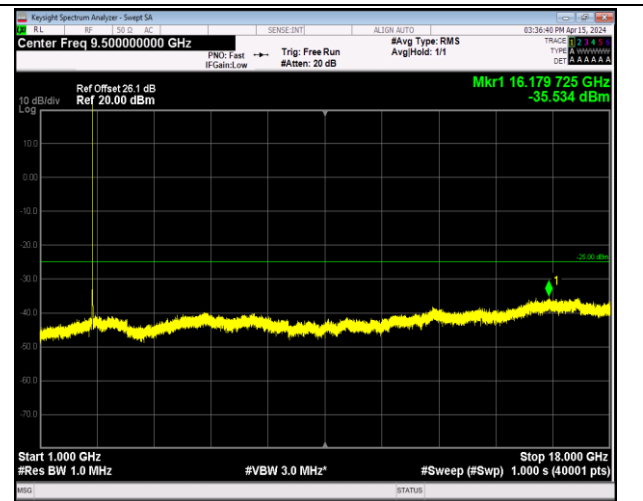
Band7_5MHz_64QAM_21425_1RB#0_1000~18000_1000~18000
