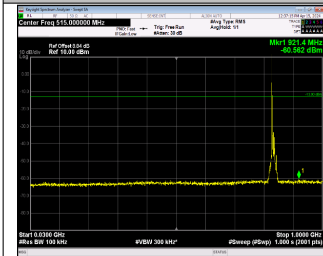
Band5_10MHz_QPSK_20525_1RB#0_30~1000_30~1000
