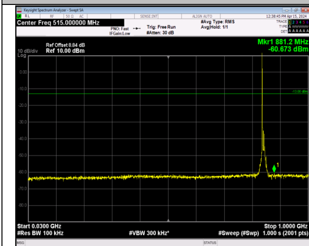
Band5_10MHz_16QAM_20600_1RB#0_30~1000_30~100
