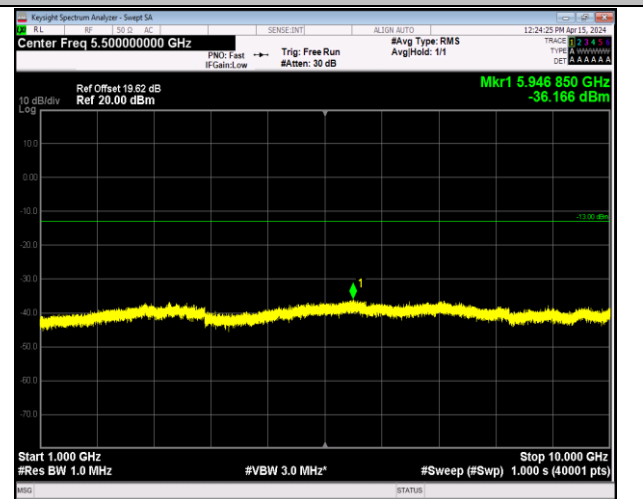
Band5_1.4MHz_64QAM_20643_1RB#0_1000~10000_00~10000
