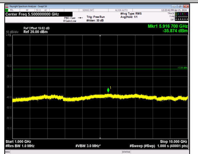
Band5_1.4MHz_QPSK_20643_1RB#0_1000~10000_1000~10000
