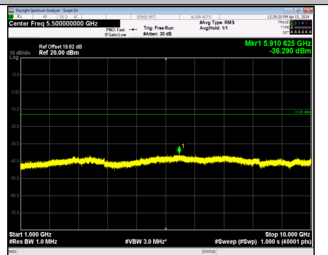
Band5_10MHz_64QAM_20600_1RB#0_1000~10000_100
