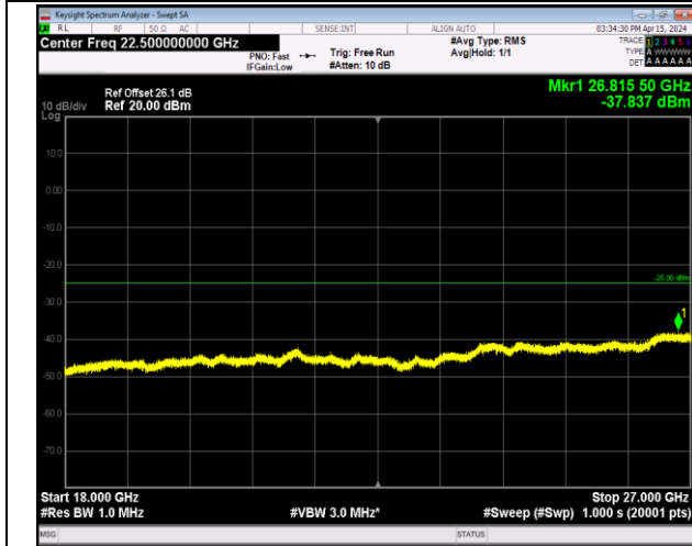
Band7_5MHz_16QAM_21100_1RB#0_18000~27000_18000~27000
