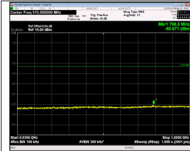
Band2_20MHz_QPSK_18700_1RB#0_30~1000_30~1000
