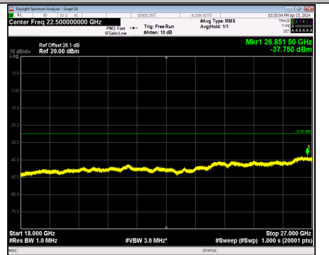
Band7_5MHz_64QAM_21100_1RB#0_18000~27000_18000~27000
