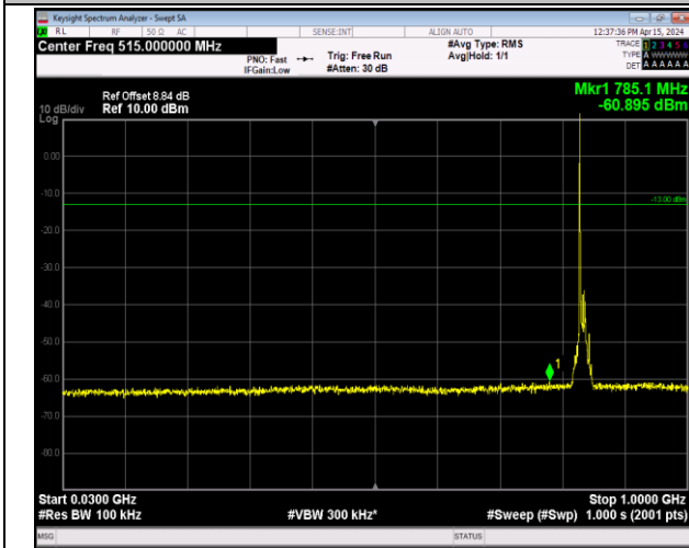
Band5_10MHz_16QAM_20525_1RB#0_30~1000_30~100
