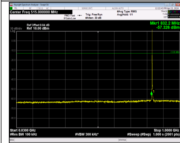
Band5_1.4MHz_16QAM_20525_1RB#0_30~1000_30~10 00
