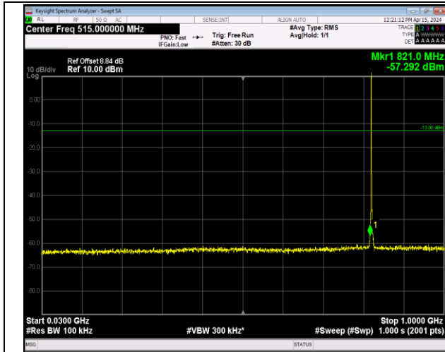
Band5_1.4MHz_QPSK_20407_1RB#0_30~1000_30~1000
