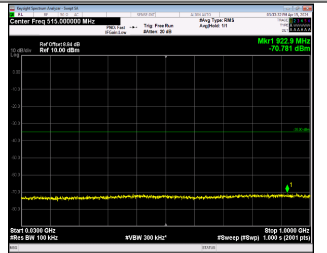
Band7_5MHz_QPSK_21100_1RB#0_30~1000_30~1000
