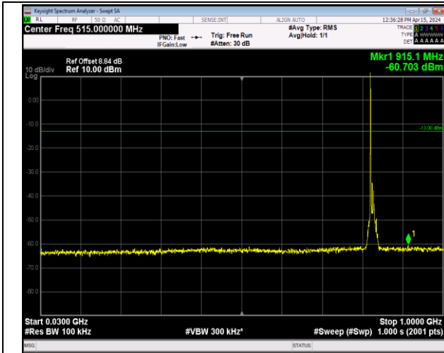
Band5_10MHz_16QAM_20450_1RB#0_30~1000_30~100
