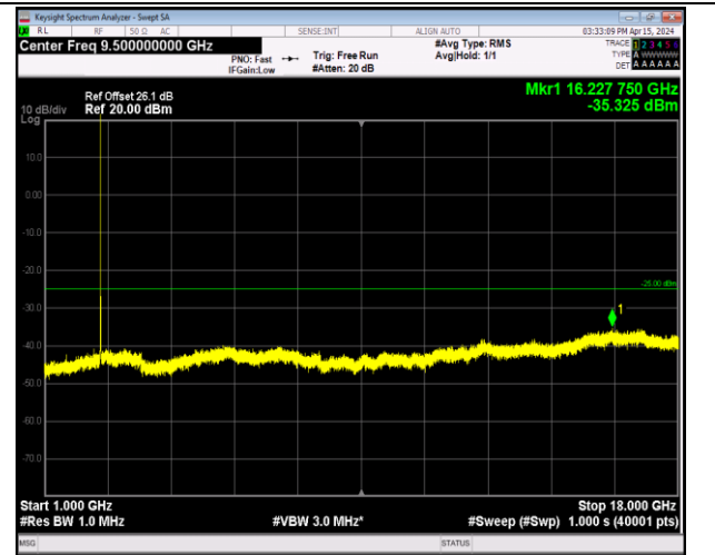
Band7_5MHz_64QAM_20775_1RB#0_1000~18000_1000~18000
