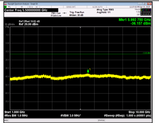
Band5_10MHz_64QAM_20450_1RB#0_1000~10000_100
