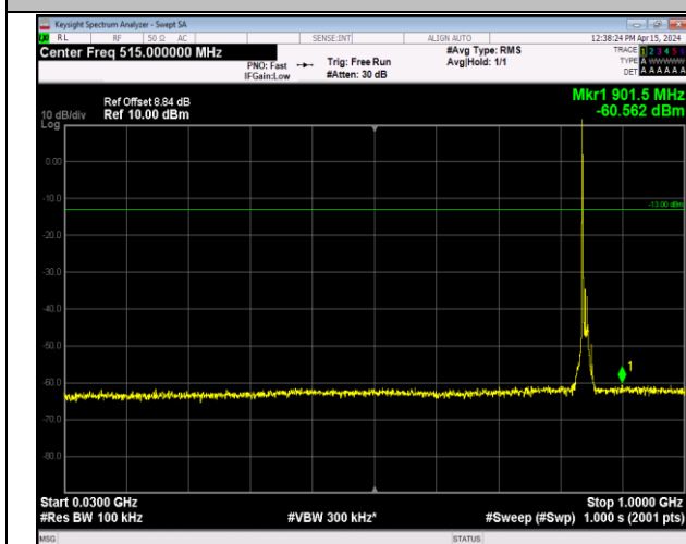
Band5_10MHz_QPSK_20600_1RB#0_30~1000_30~1000
