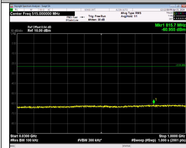
Band2_20MHz_QPSK_19100_1RB#0_30~1000_30~1000
