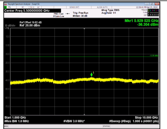
Band5_10MHz_16QAM_20450_1RB#0_1000~10000_100
