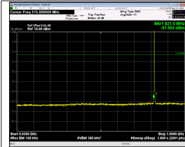
Band5_1.4MHz_16QAM_20407_1RB#0_30~1000_30~10 00
