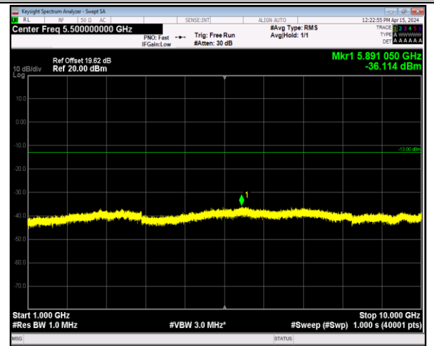
Band5_1.4MHz_16QAM_20525_1RB#0_1000~10000_100 0~10000
