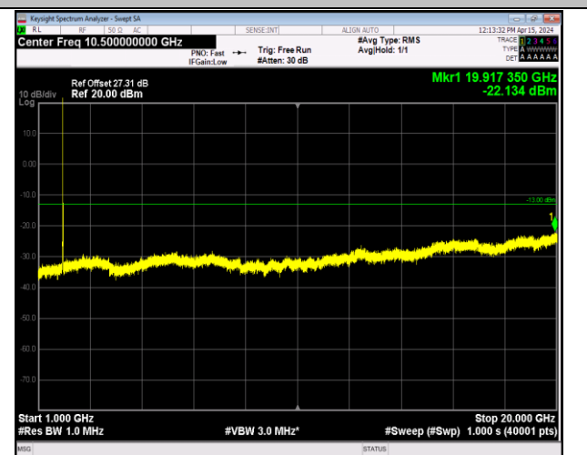
Band2_20MHz_16QAM_19100_1RB#0_1000~20000_100 0~20000
