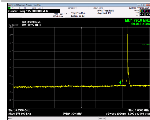
Band5_10MHz_64QAM_20600_1RB#0_30~1000_30~100
