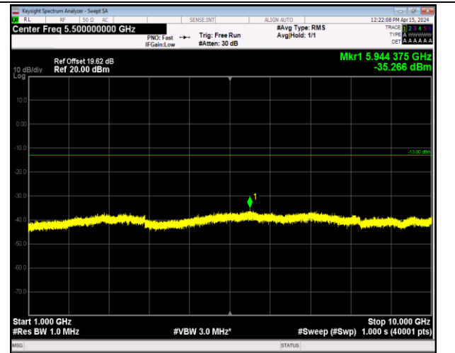
Band5_1.4MHz_64QAM_20407_1RB#0_1000~10000_00~10000
