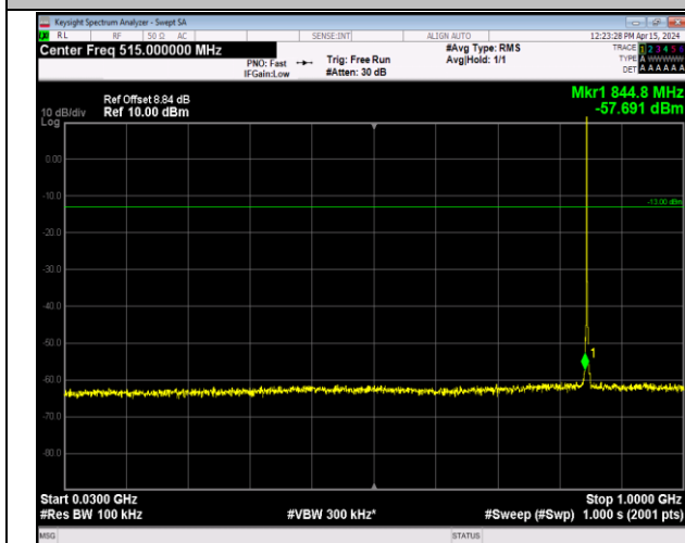
Band5_1.4MHz_QPSK_20643_1RB#0_30~1000_30~1000
