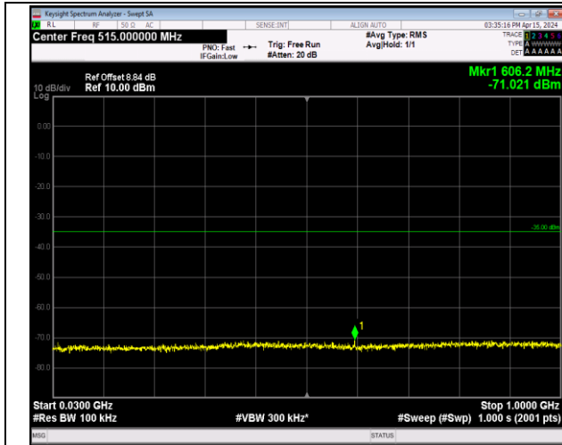
Band7_5MHz_QPSK_21425_1RB#0_30~1000_30~1000
