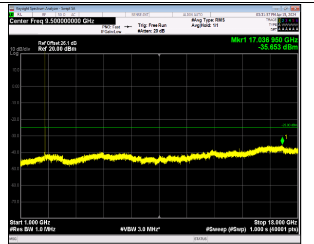
Band7_5MHz_QPSK_20775_1RB#0_1000~18000_1000~18000
