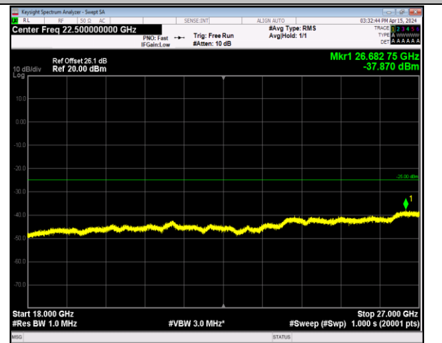
Band7_5MHz_16QAM_20775_1RB#0_18000~27000_18000~27000
