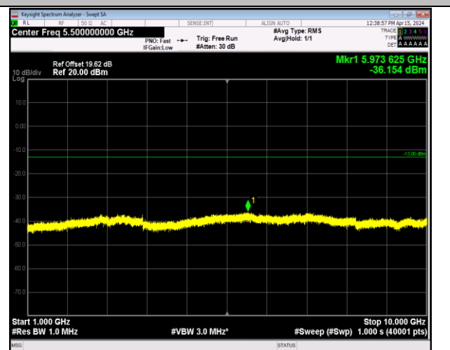
Band5_10MHz_16QAM_20600_1RB#0_1000~10000_100
