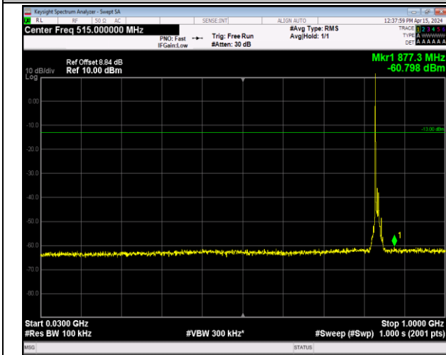
Band5_10MHz_64QAM_20525_1RB#0_30~1000_30~100
