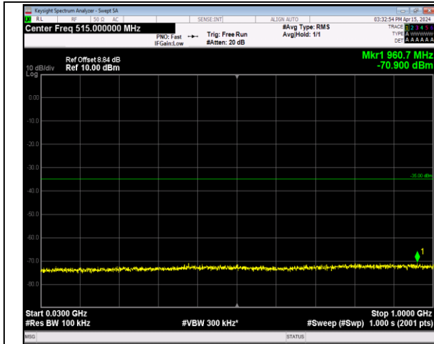
Band7_5MHz_64QAM_20775_1RB#0_30~1000_30~1000
