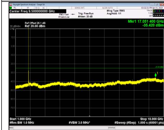
Band7_5MHz_16QAM_20775_1RB#0_1000~18000_1000~18000
