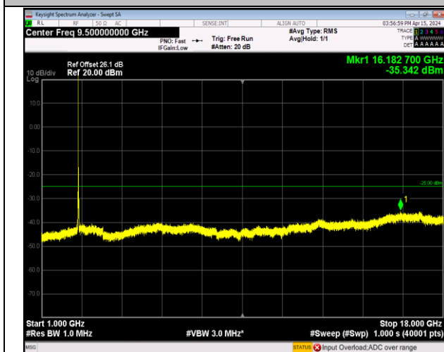
Band7_20MHz_QPSK_21350_1RB#0_1000~18000_1000~18000
