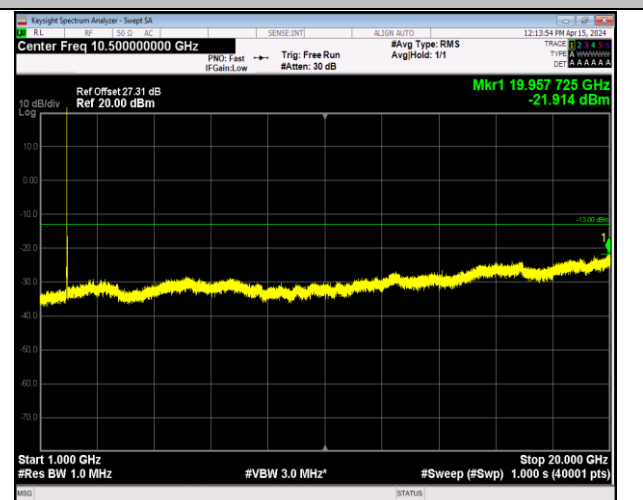
Band2_20MHz_64QAM_19100_1RB#0_1000~20000_100
