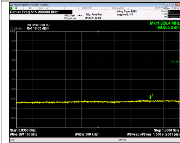
Band2_20MHz_64QAM_18900_1RB#0_30~1000_30~100
