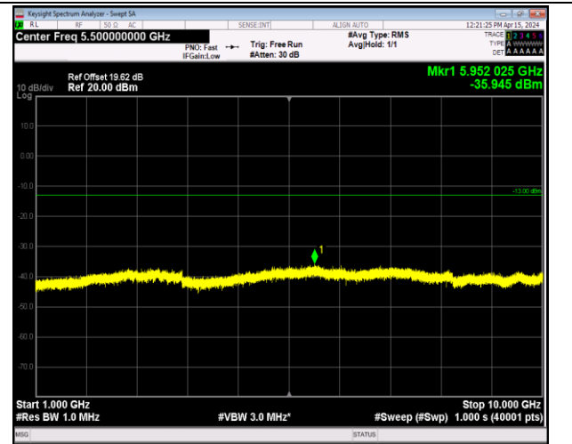
Band5_1.4MHz_QPSK_20407_1RB#0_1000~10000_1000~10000
