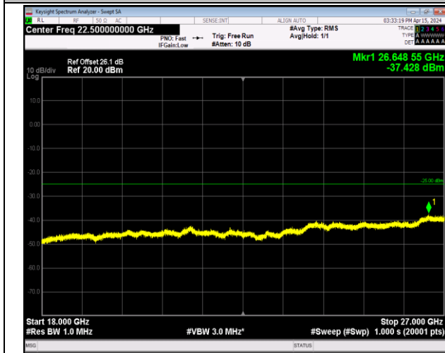
Band7_5MHz_64QAM_20775_1RB#0_18000~27000_18000~27000
