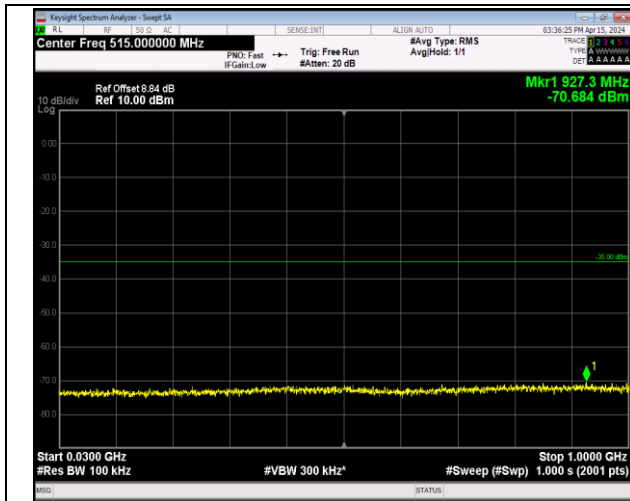
Band7_5MHz_64QAM_21425_1RB#0_30~1000_30~1000
