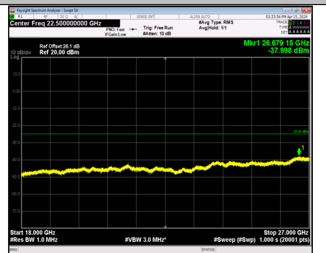
Band7_5MHz_QPSK_21100_1RB#0_18000~27000_18000~27000
