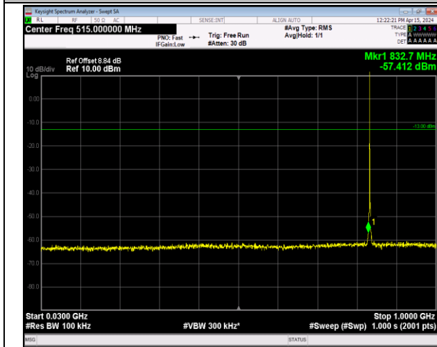
Band5_1.4MHz_QPSK_20525_1RB#0_30~1000_30~1000
