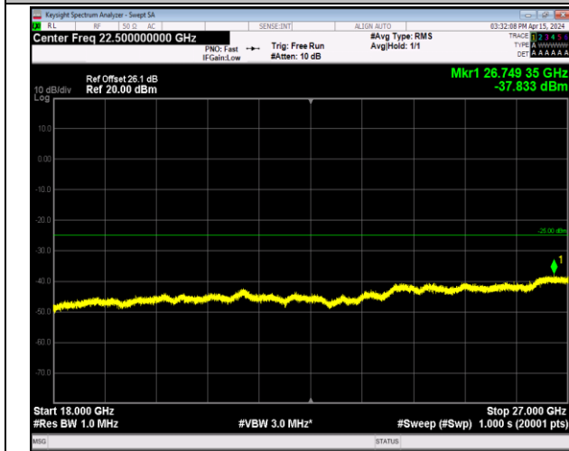
Band7_5MHz_QPSK_20775_1RB#0_18000~27000_18000~27000
