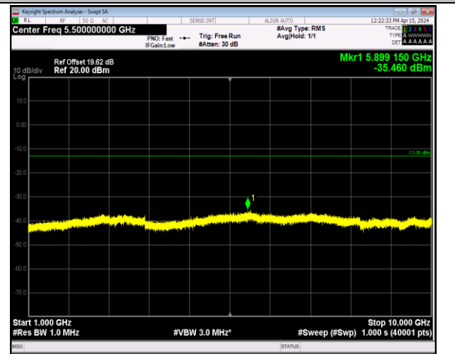
Band5_1.4MHz_QPSK_20525_1RB#0_1000~10000_1000~10000
