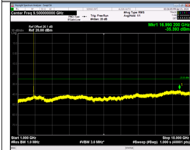
Band7_5MHz_16QAM_21425_1RB#0_1000~18000_1000~18000
