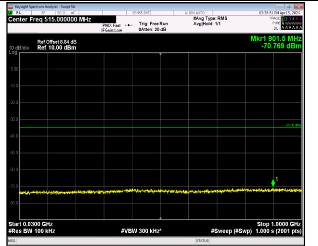
Band7_5MHz_16QAM_21425_1RB#0_30~1000_30~1000
