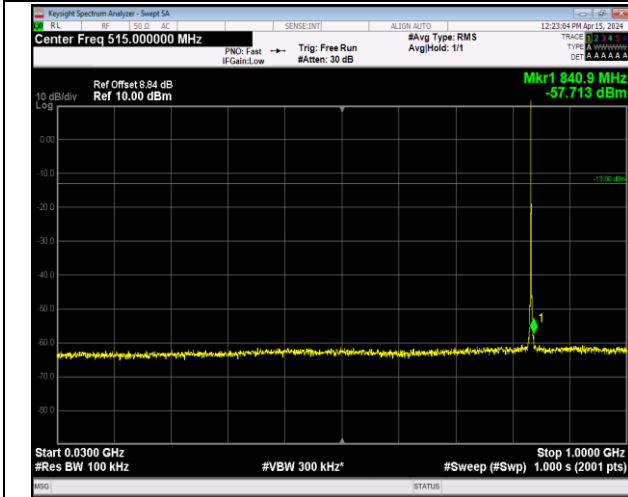
Band5_1.4MHz_64QAM_20525_1RB#0_30~1000_30~1000
