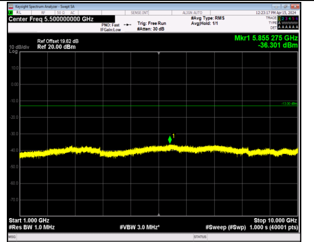
Band5_1.4MHz_64QAM_20525_1RB#0_1000~10000_00~10000
