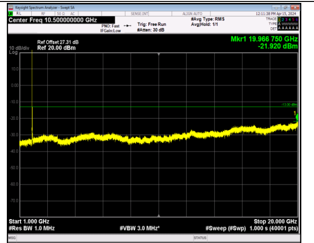
Band2_20MHz_64QAM_18700_1RB#0_1000~20000_100
