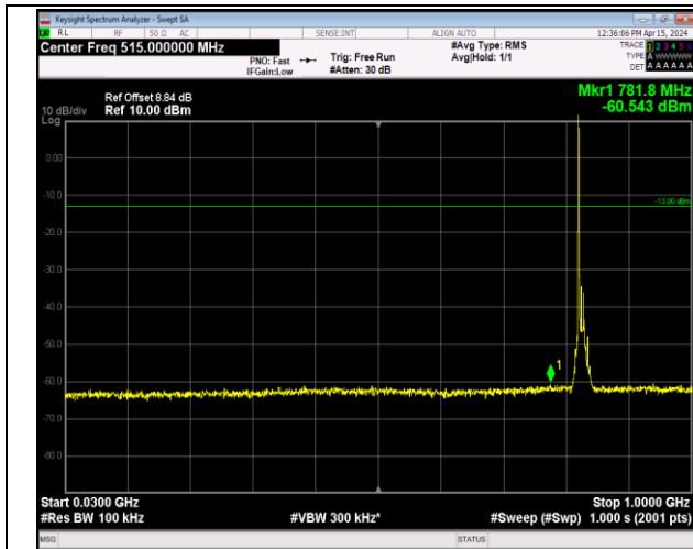
Band5_10MHz_QPSK_20450_1RB#0_30~1000_30~1000
