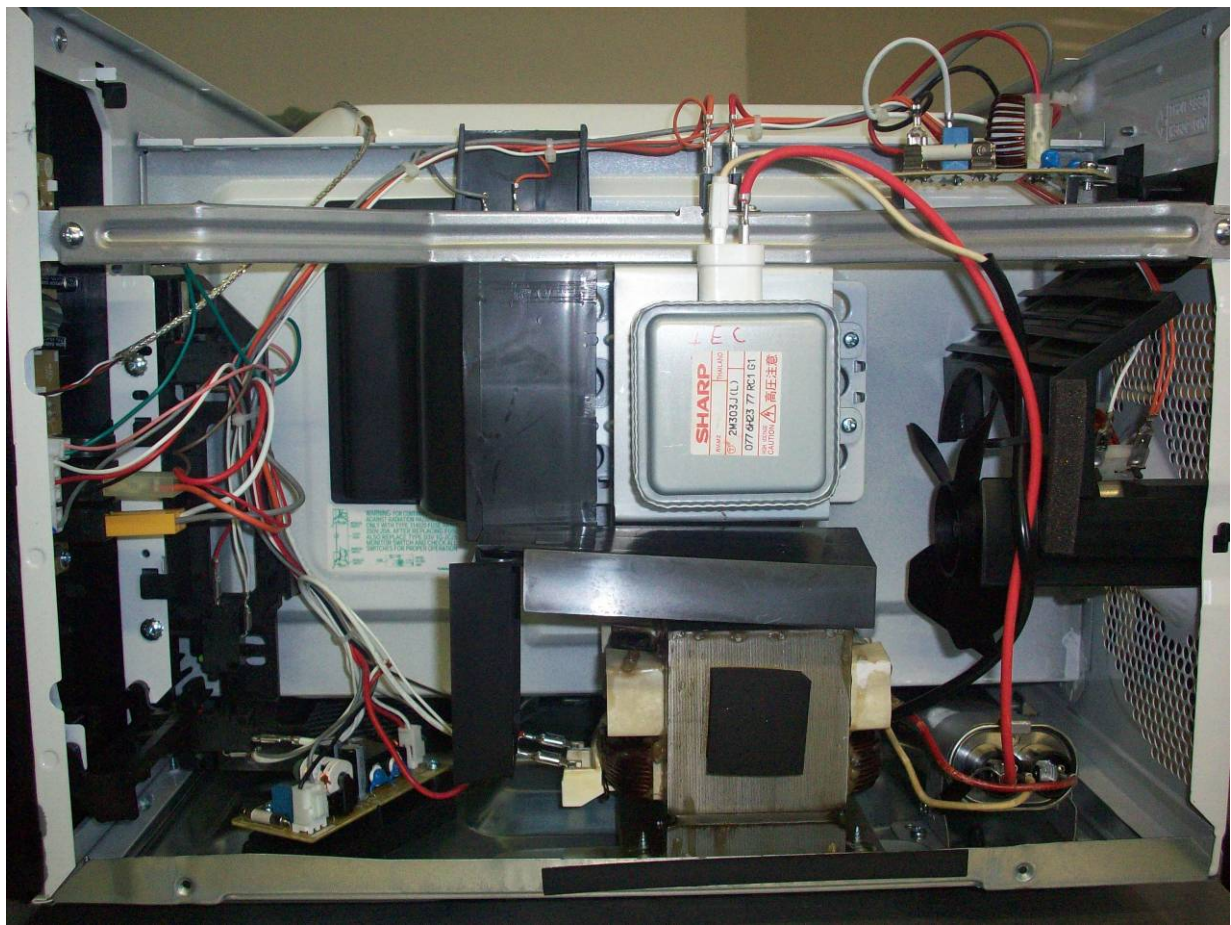
Figure 2. Magnetron Location
