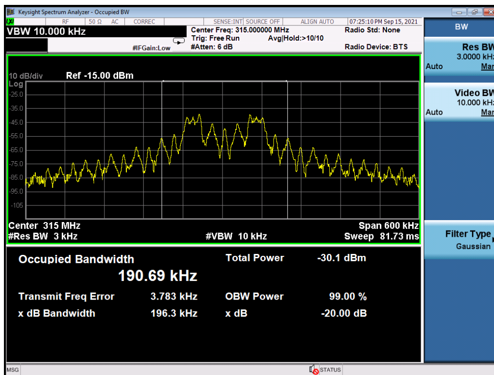
Figure 1: 20dB Bandwidth
