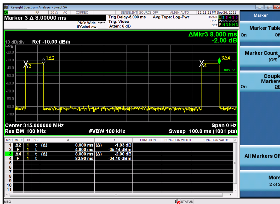
Figure 3: Duty Cycle
