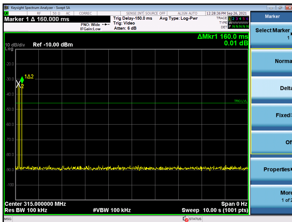
Figure 2: Deactivation Time
