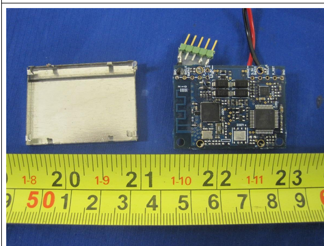
EUT – Top View without Shielding
