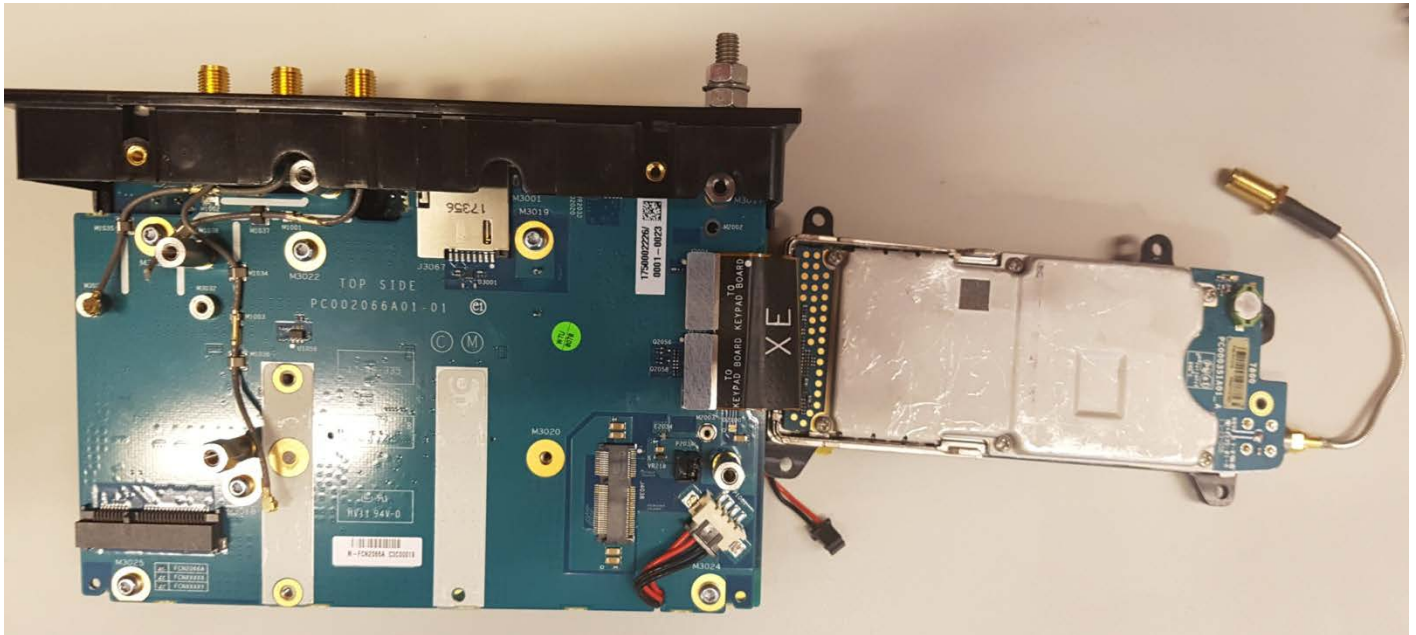
MC-EDGE Piggy Board Top View With Front Panel (APX4000 7/800 Flipped Over)
