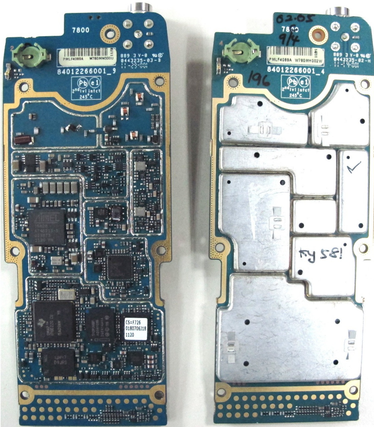
APX4000 7/800 Board Without and With Shields (Top)
