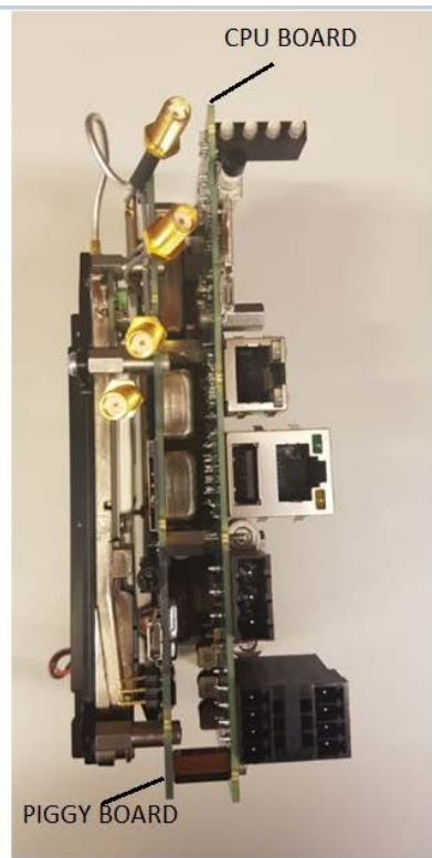
INTERNAL CPU & PIGGY BOARD (APX4000 7/800 INSTALLED WITH LoRA & LTE)
