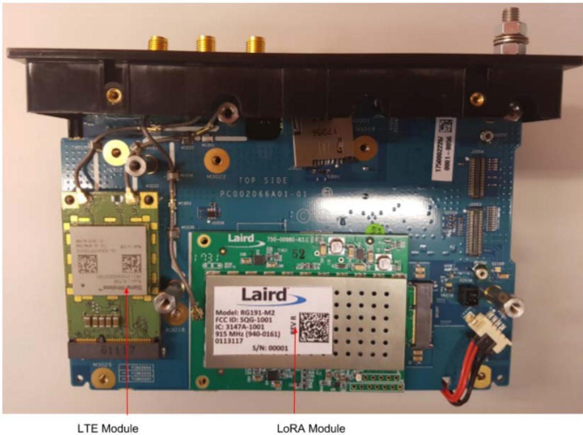
MC-EDGE Piggy Board Top View With Front Panel (APX4000 7/800 Removed, with LORA and LTE)
