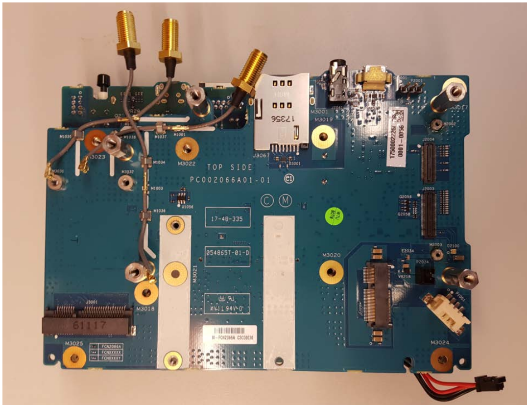
MC-EDGE Piggy Board Top View Without Front Panel (APX4000 7/800 Removed)
