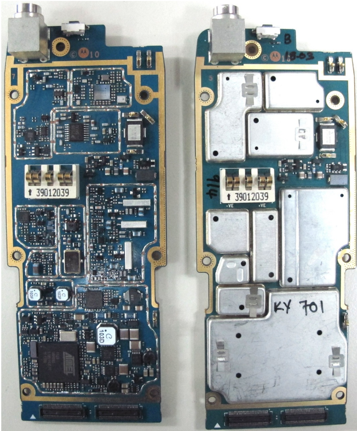
APX4000 7/800 Board Without and With Shields (Bottom)
