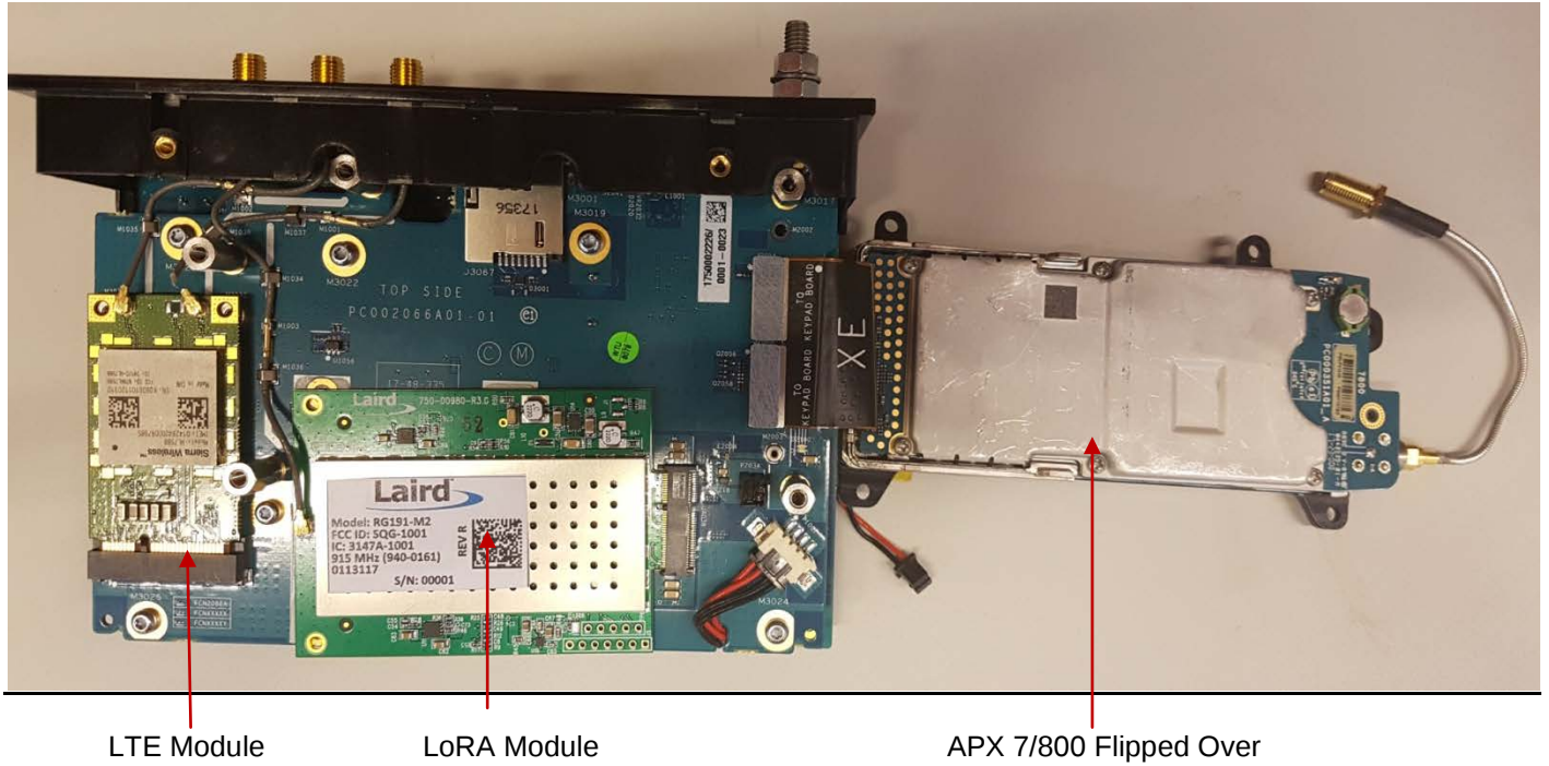
MC-EDGE Piggy Board Top View With Front Panel (APX4000 7/800 Flipped over, with LORA and LTE)
