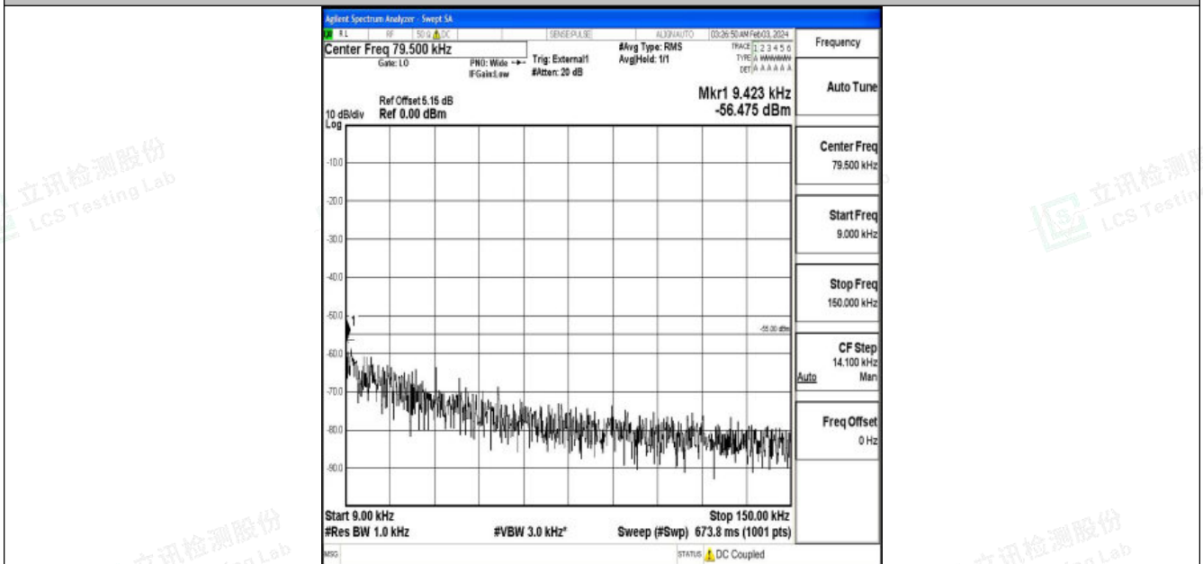
Band38_5MHz_16QAM_37775_1RB#0_0.009~0.15_0.009~0.15
