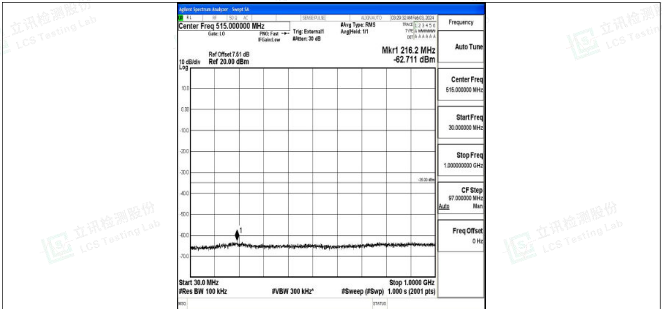
Band38_5MHz_QPSK_38000_1RB#0_30~1000_30~1000
