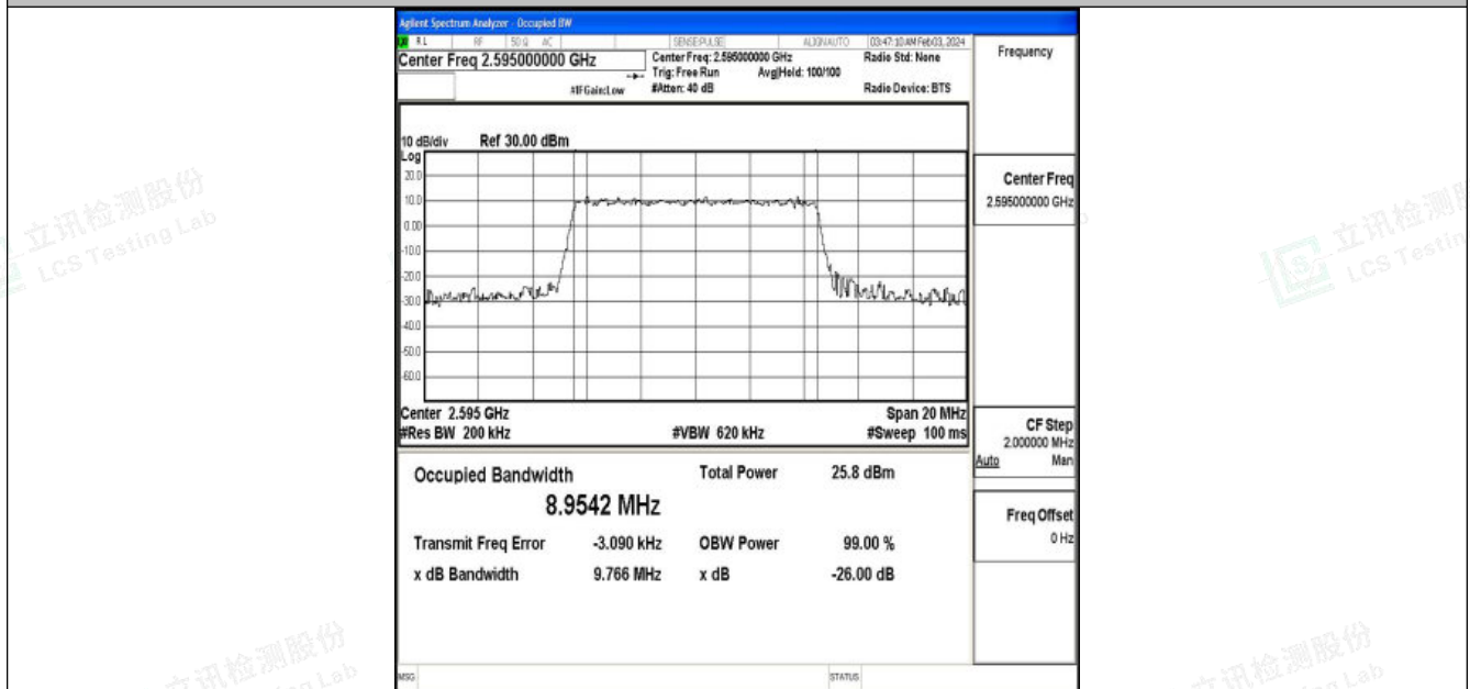
Band38-10MHz-16QAM-38000-50RB#0-PASS
