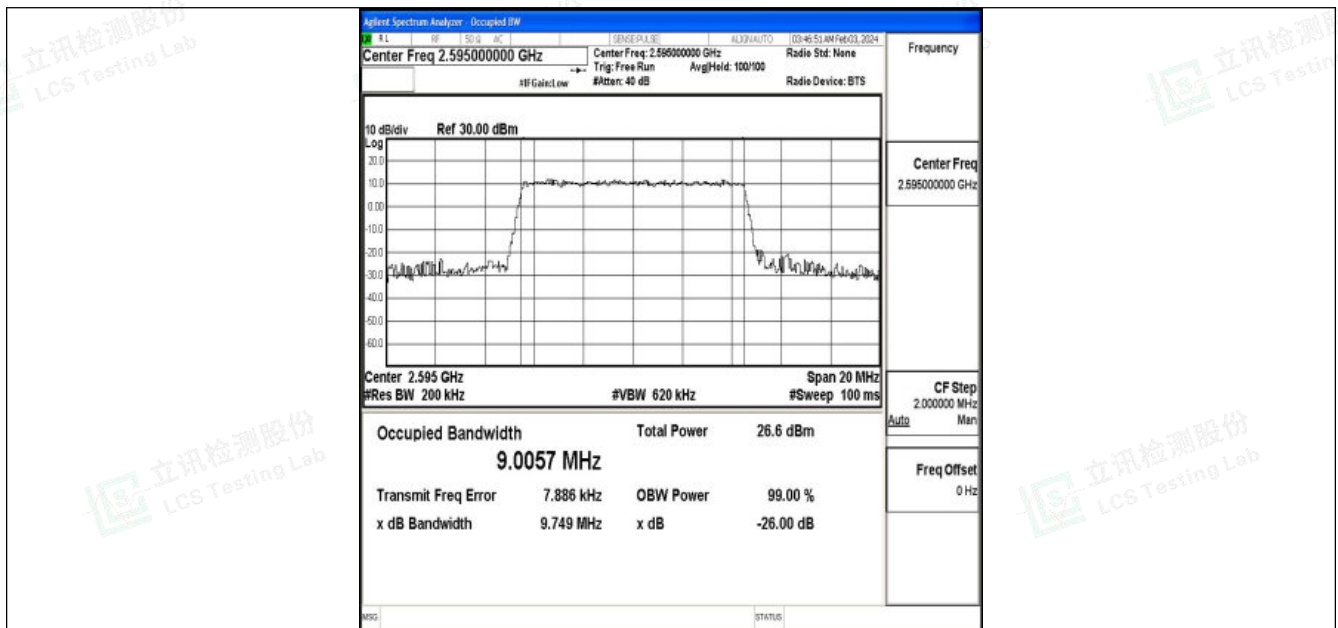
Band38-10MHz-QPSK-38000-50RB#0-PASS
