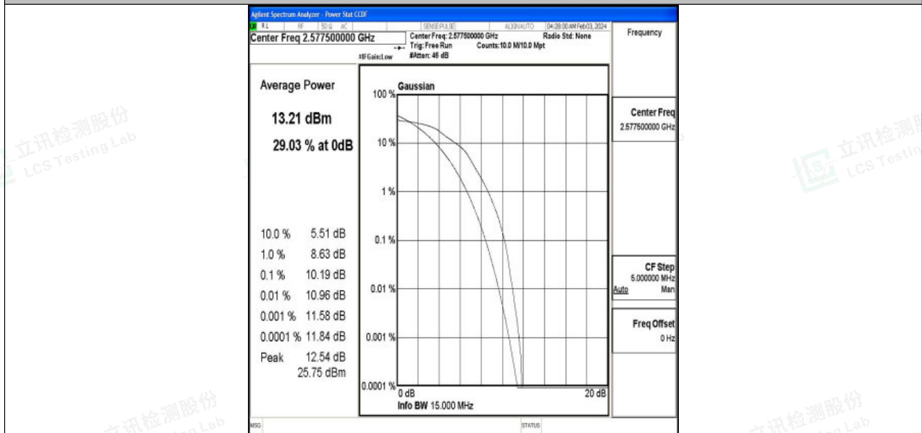
Band38-15MHz-16QAM-37825-75RB#0-PASS
