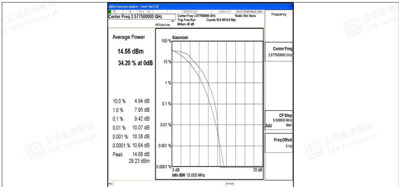
Band38-15MHz-QPSK-37825-75RB#0-PASS
