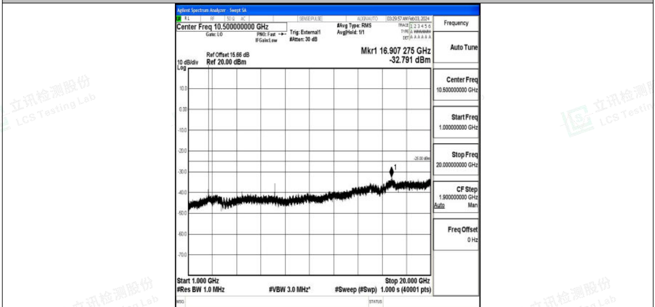
Band38_5MHz_QPSK_38000_1RB#0_1000~20000_1000~20000
