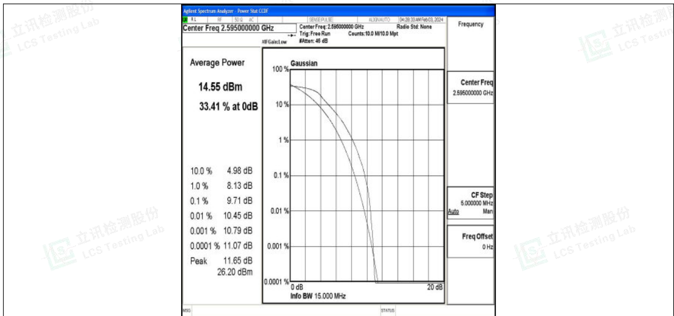
Band38-15MHz-QPSK-38000-75RB#0-PASS
