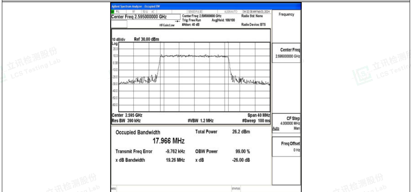
Band38-20MHz-16QAM-38000-100RB#0-PASS
