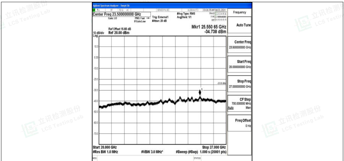
Band38_5MHz_QPSK_37775_1RB#0_20000~27000_20000~27000
