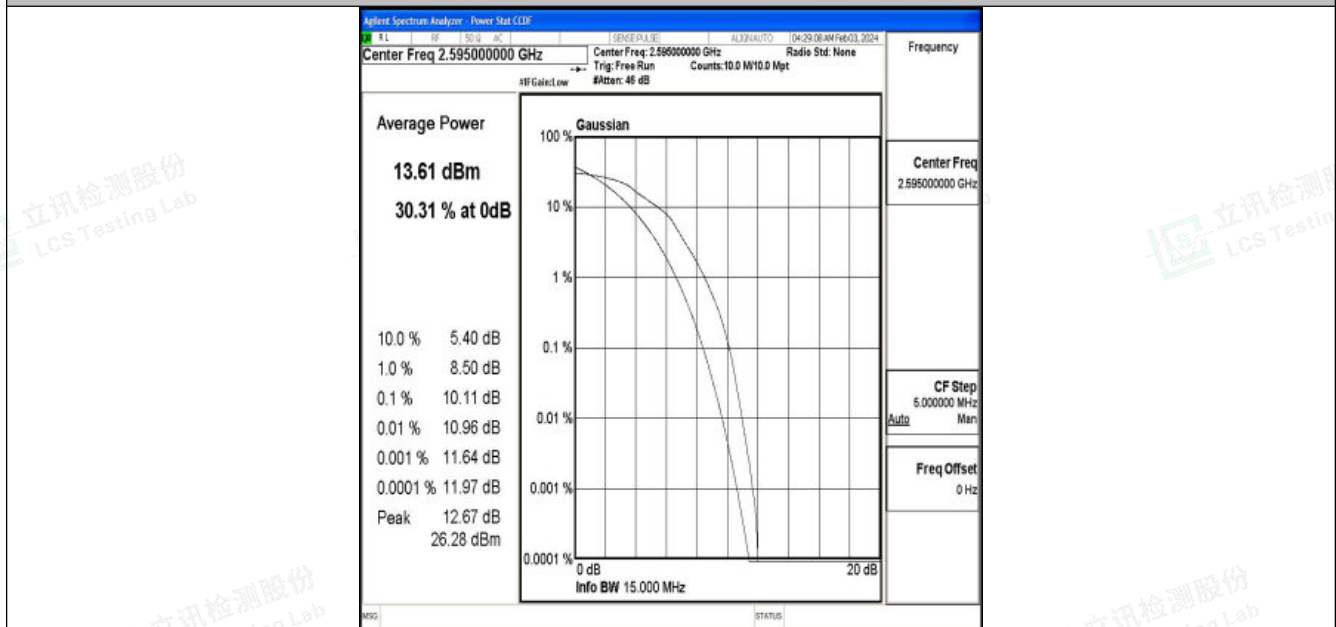
Band38-15MHz-16QAM-38000-75RB#0-PASS
