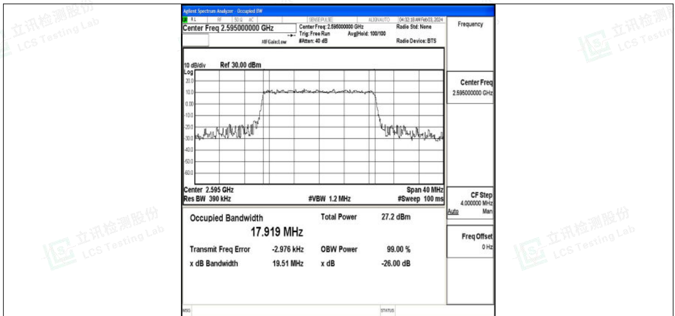
Band38-20MHz-QPSK-38000-100RB#0-PASS
