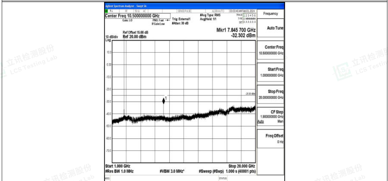
Band38_5MHz_QPSK_38225_1RB#0_1000~20000_1000~20000
