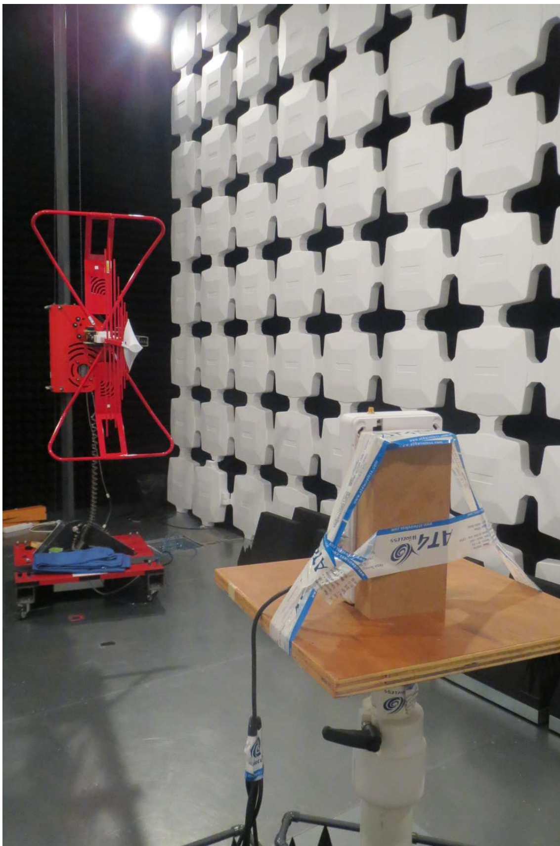
Set-up with internal antenna
