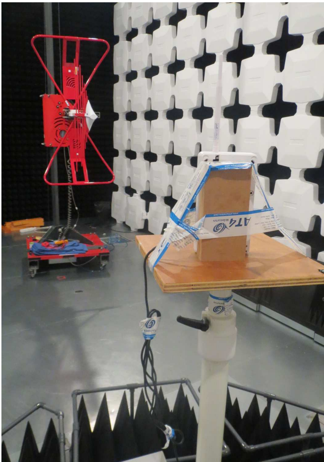
Set-up with external antenna
