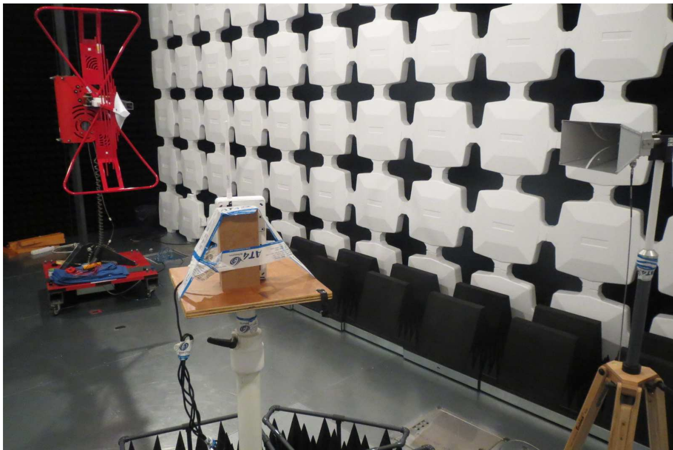
Set-up with external antenna
