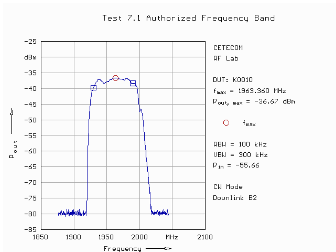
Fig. 8: Frequency response in downlink in band 2.
