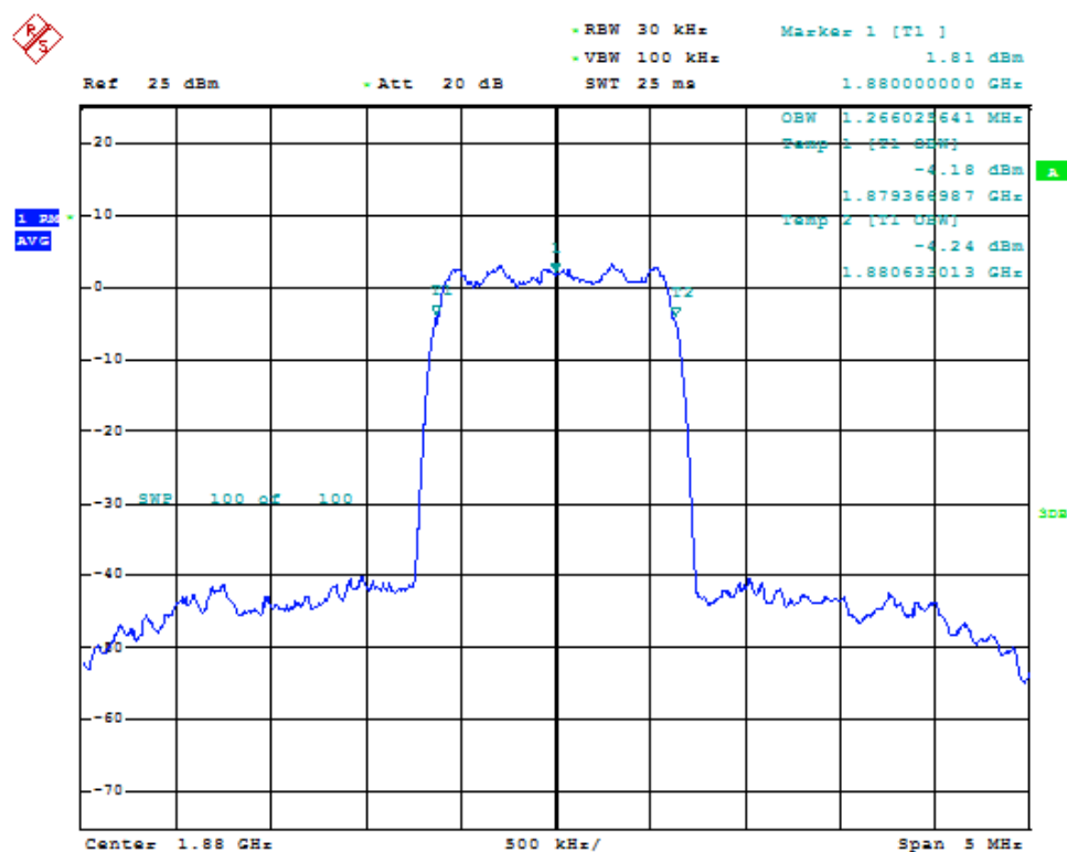
Fig. 220: Occupied bandwidth for CDMA signal in band 2 uplink.
