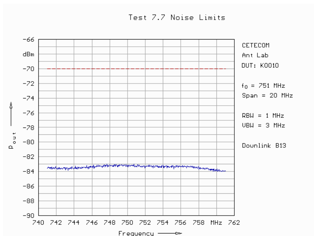
Fig. 177: Noise limits in downlink in band 13.
