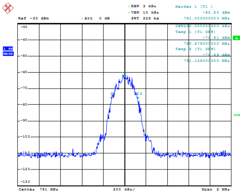
Fig. 217: Occupied bandwidth for GSM signal when using a through in band 13 downlink.
