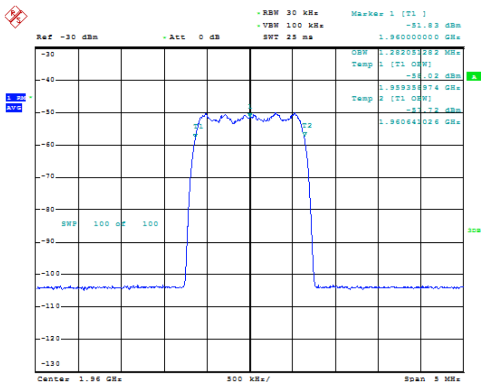
Fig. 222: Occupied bandwidth for CDMA signal in band 2 downlink.
