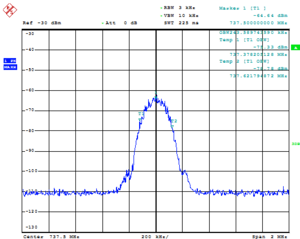
Fig. 213: Occupied bandwidth for GSM signal when using a through in band 12 downlink.
