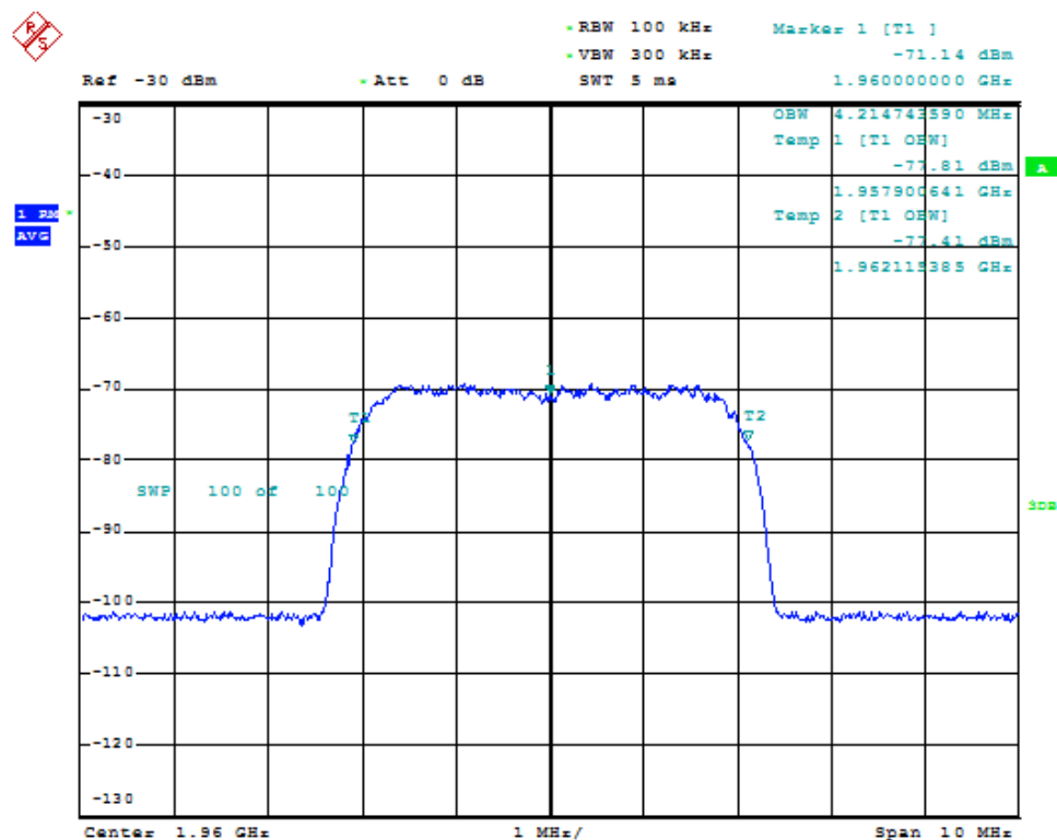
Fig. 241: Occupied bandwidth for WCDMA signal when using a through in band 2 downlink.
