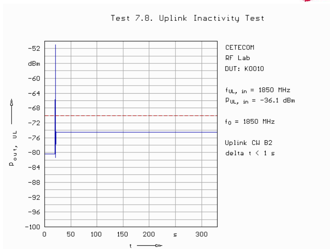
Fig. 179: Uplink inactivity test in band 2.
