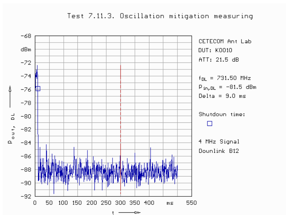
Fig. 300: Band 12 downlink shut down time.
