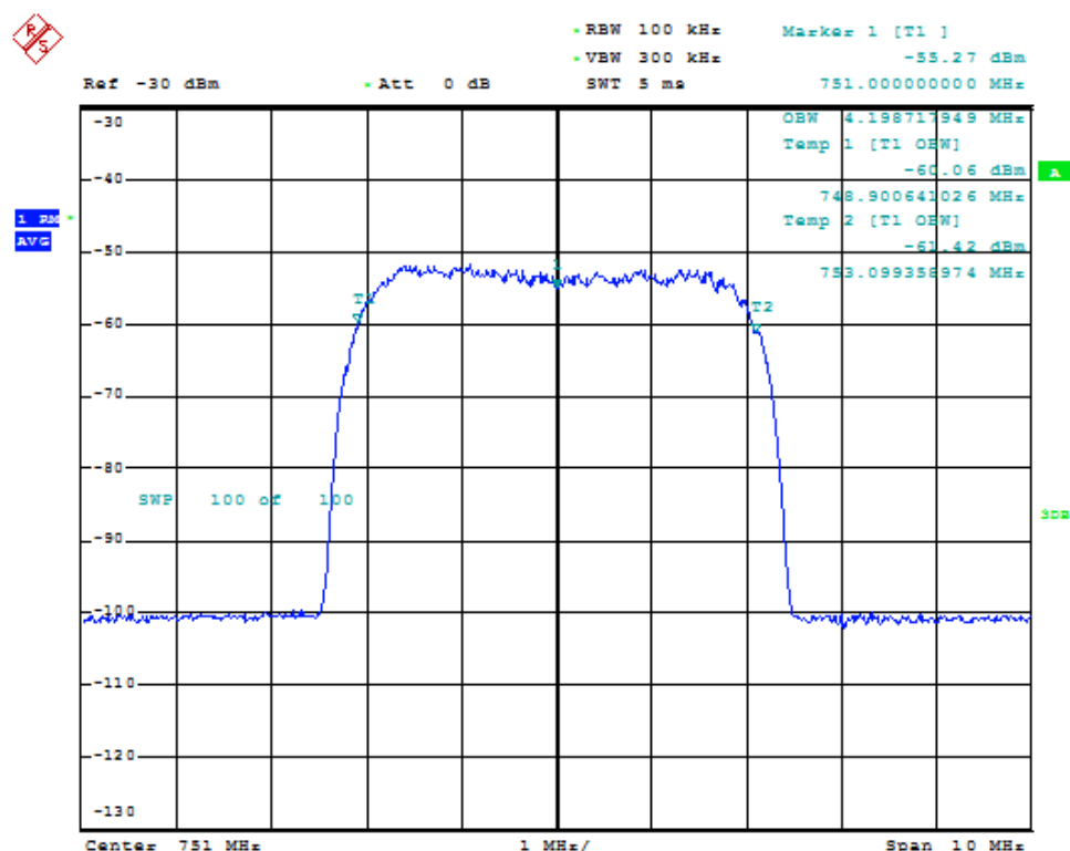
Fig. 257: Occupied bandwidth for WCDMA signal when using a through in band 13 downlink.
