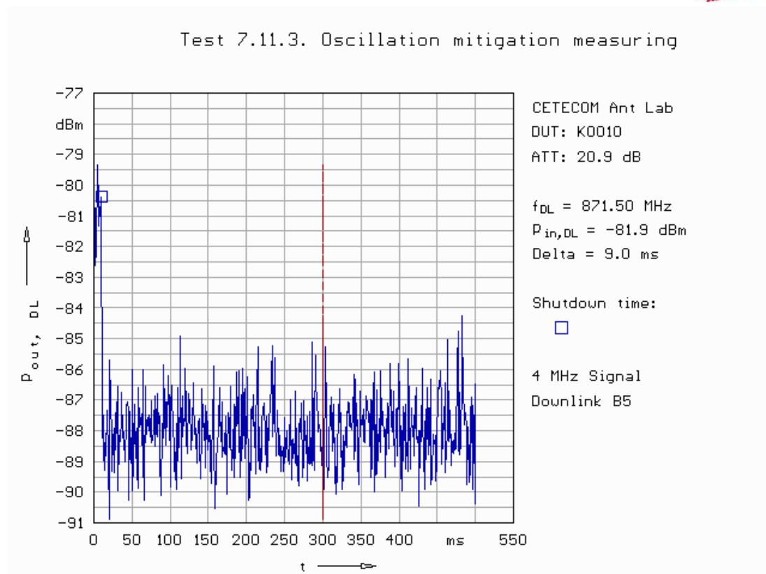
Fig. 299: Band 5 downlink shut down time.
