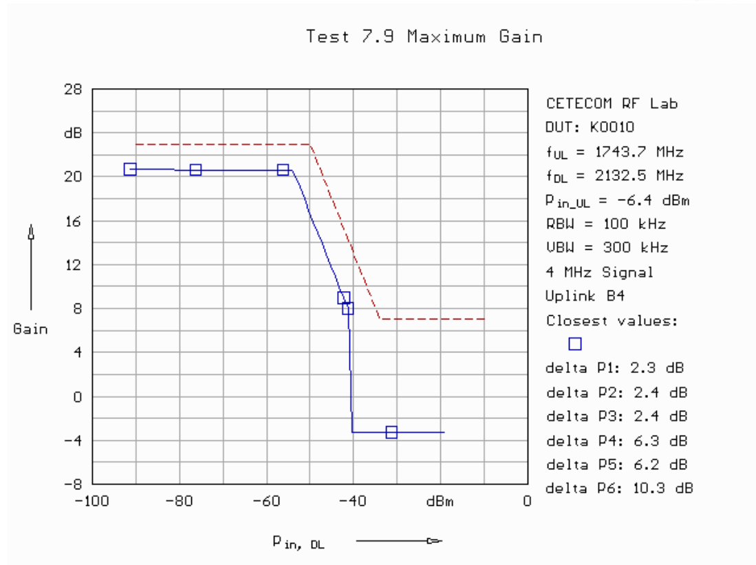
Fig. 188: Variable RSSI dependent uplink gain in band 4.
