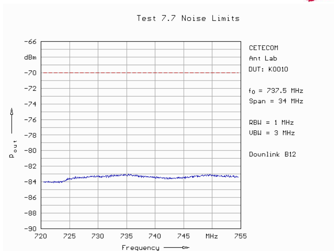
Fig. 176: Noise limits in downlink in band 12.
