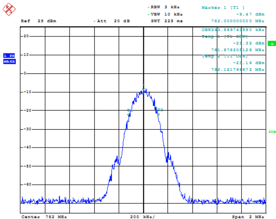
Fig. 215: Occupied bandwidth for GSM signal when using a through in band 13 uplink.
