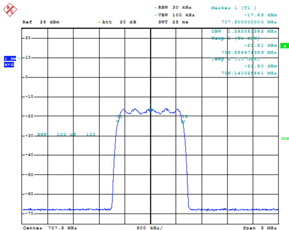
Fig. 231: Occupied bandwidth for CDMA signal when using a through in band 12 uplink.
