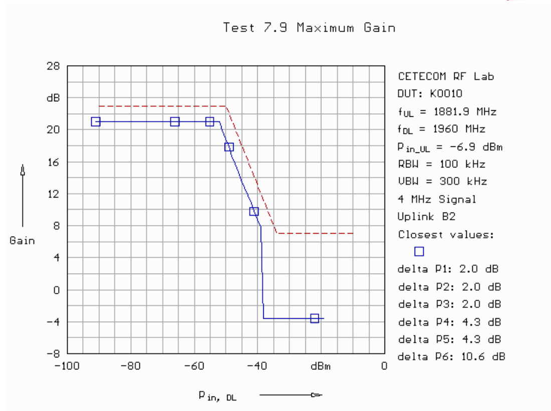
Fig. 186: Variable RSSI dependent uplink gain in band 2.
