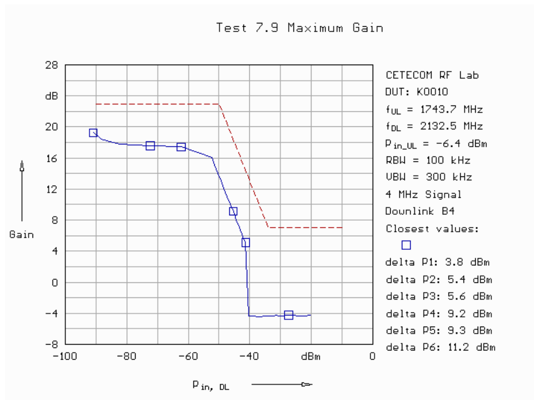
Fig. 189: Variable RSSI dependent downlink gain in band 4.
