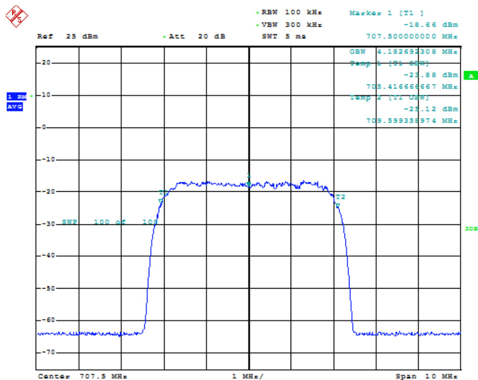
Fig. 251: Occupied bandwidth for WCDMA signal when using a through in band 12 uplink.
