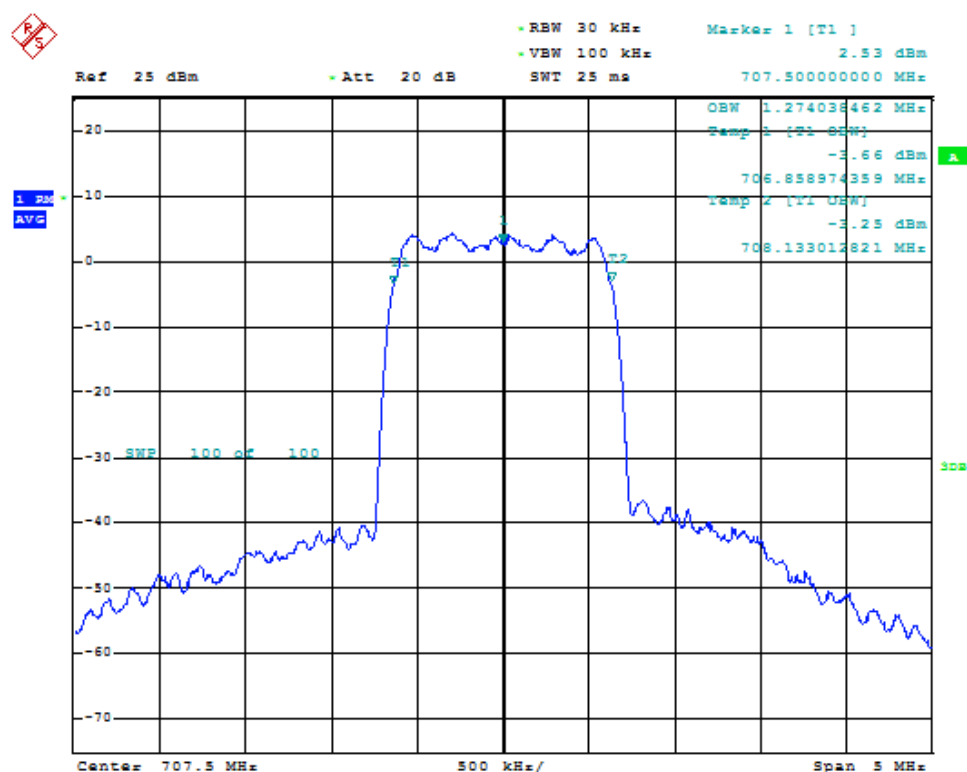
Fig. 232: Occupied bandwidth for CDMA signal in band 12 uplink.
