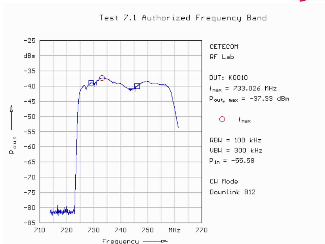
Fig. 11: Frequency response in downlink in band 12.
