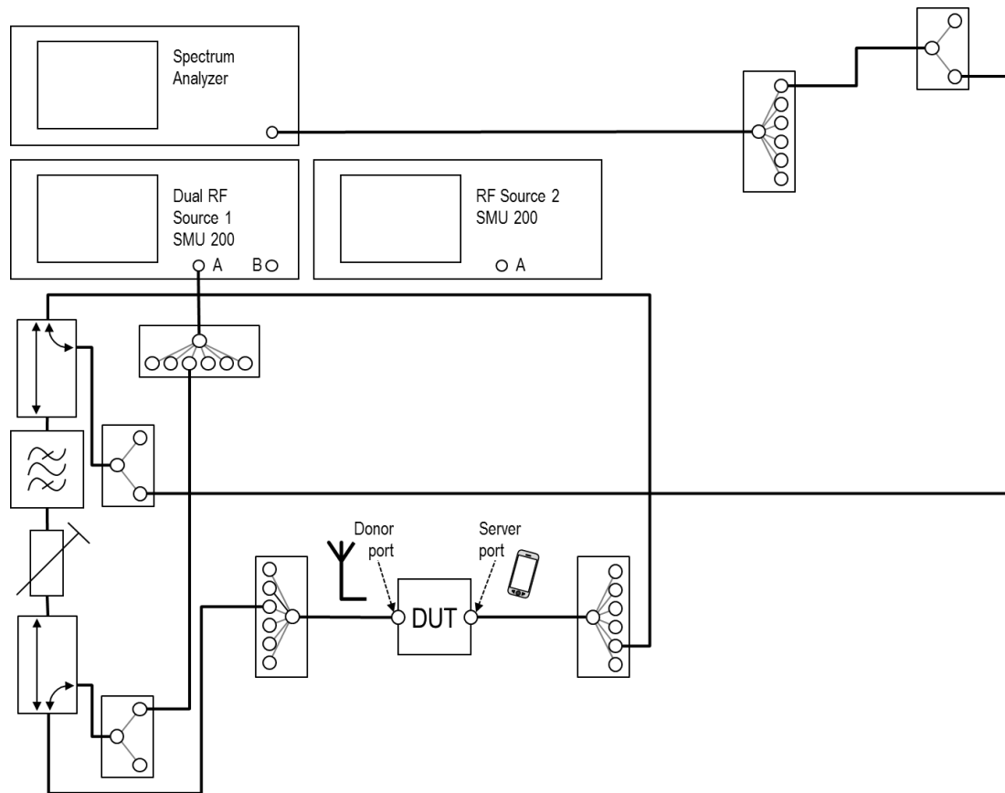
Fig. 260: Set up for oscillation detection and mitigation tests in downlink.
