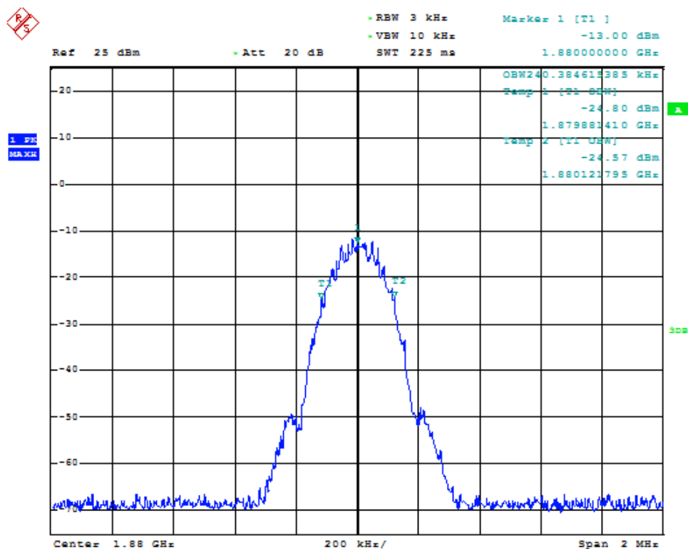
Fig. 199: Occupied bandwidth for GSM signal when using a through in band 2 uplink.
