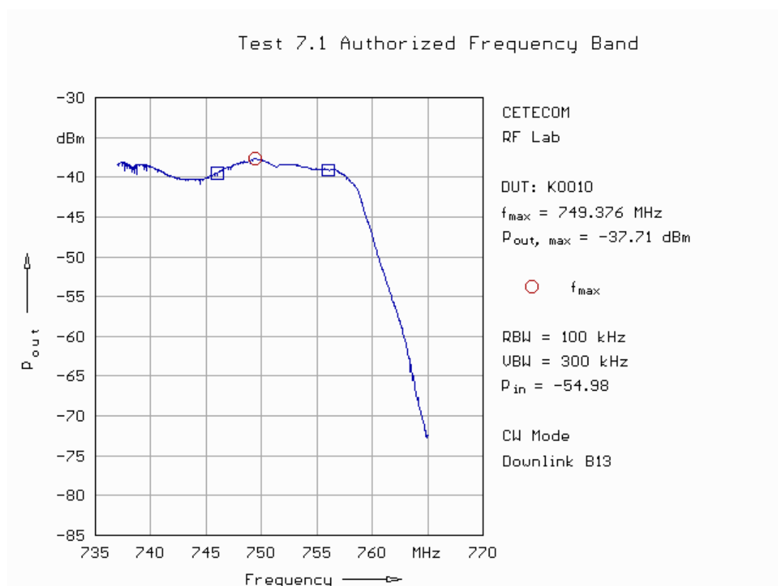
Fig. 12: Frequency response in downlink in band 13.
