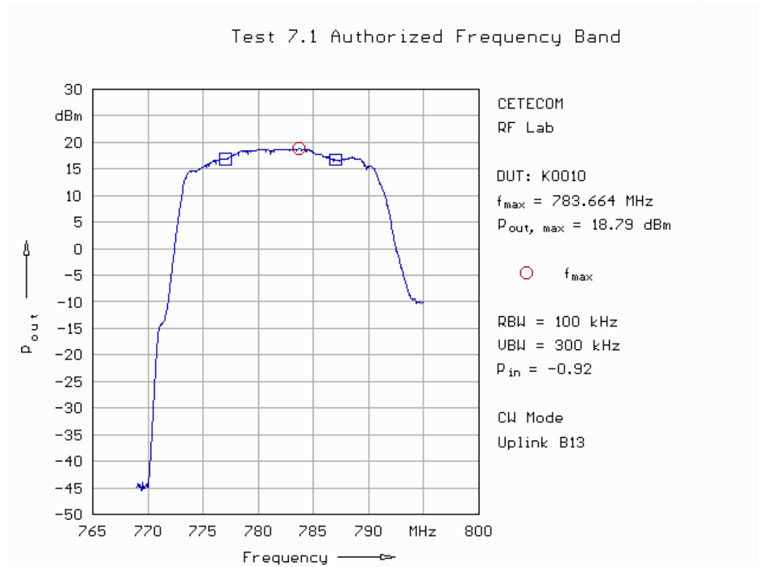
Fig. 7: Frequency response in uplink in band 13.
