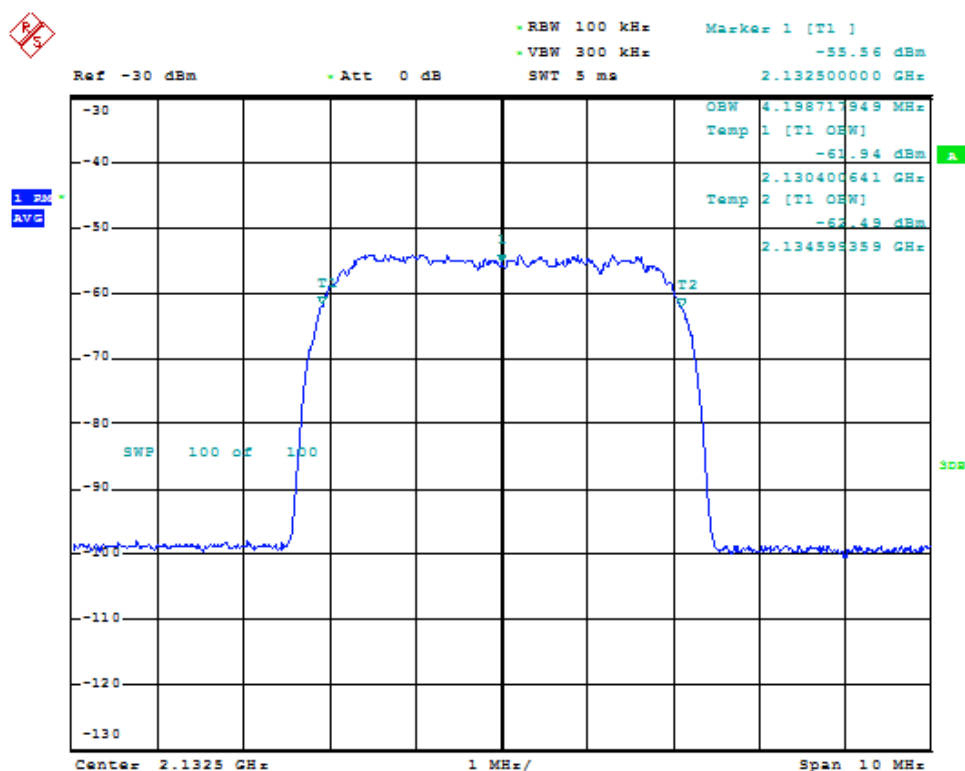
Fig. 246: Occupied bandwidth for WCDMA signal in band 4 downlink.
