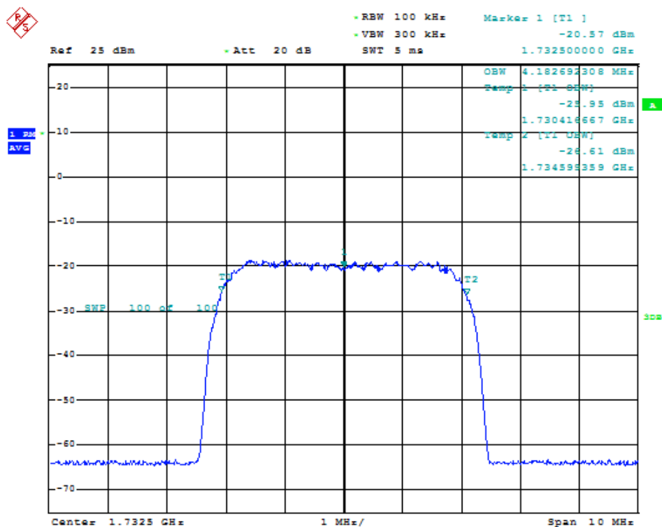
Fig. 243: Occupied bandwidth for WCDMA signal when using a through in band 4 uplink.
