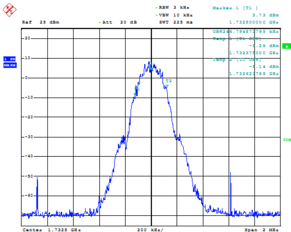
Fig. 204: Occupied bandwidth for GSM signal in band 4 uplink.
