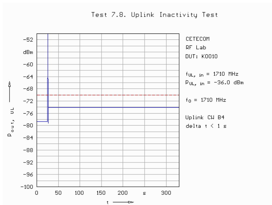
Fig. 180: Uplink inactivity test in band 4.
