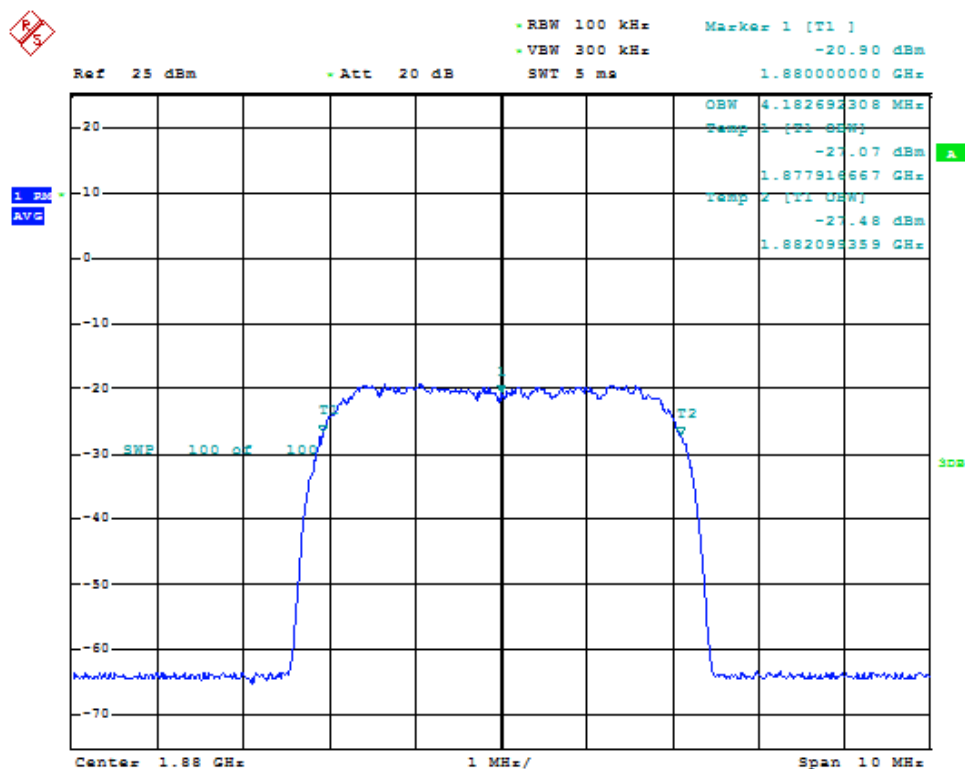
Fig. 239: Occupied bandwidth for WCDMA signal when using a through in band 2 uplink.
