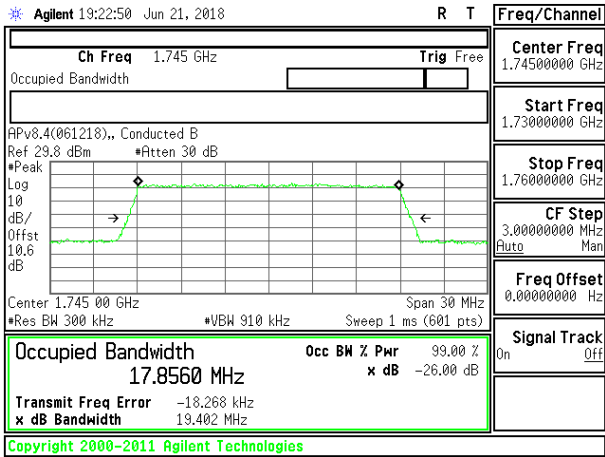
LTE B66 20MHz 64QAM Mid Channel RB100-0
