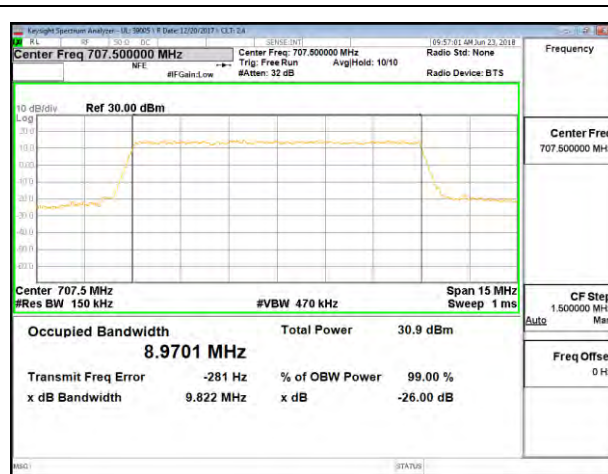
LTE B12 10MHz QPSK Mid Channel RB50-0
