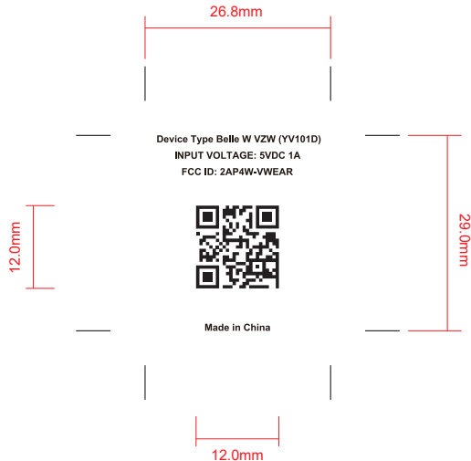
laser label is on back site of sample
