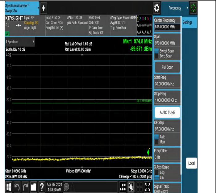
Band4_5MHz_QPSK_19975_1RB#24_30~1000_30~1000
