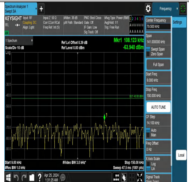
Band4_3MHz_QPSK_20385_1RB#14_0.009~0.15_0.009~0.15
