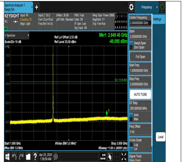
Band4_5MHz_QPSK_20175_1RB#0_1000~3000_1000~3000
