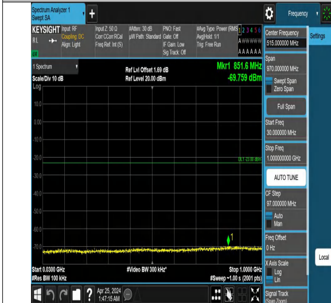
Band4_10MHz_QPSK_20175_1RB#0_30~1000_30~1000
