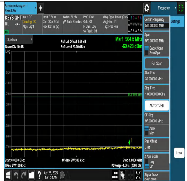
Band4_3MHz_QPSK_20385_1RB#14_30~1000_30~1000
