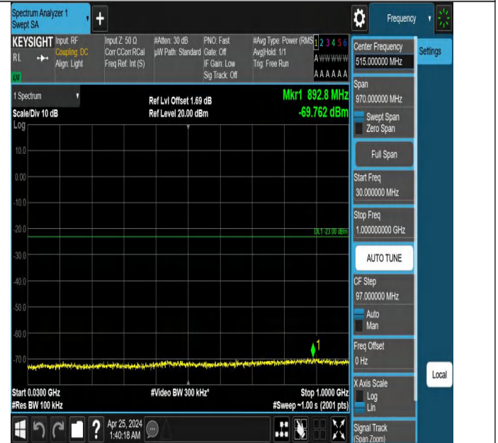
Band4_5MHz_QPSK_20375_1RB#24_30~1000_30~1000
