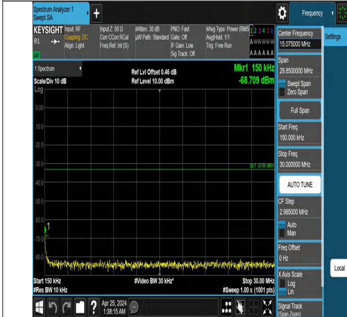
Band4_5MHz_QPSK_19975_1RB#24_0.15~30_0.15~30
