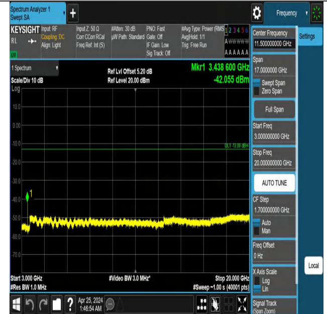
Band4_10MHz_QPSK_20000_1RB#49_3000~20000_3000~20000
