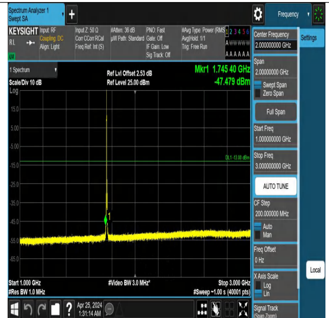
Band4_3MHz_QPSK_20385_1RB#0_1000~3000_1000~3000
