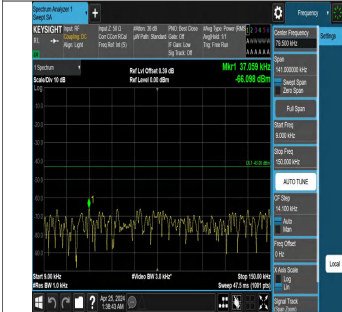
Band4_5MHz_QPSK_20175_1RB#0_0.009~0.15_0.009~0.15
