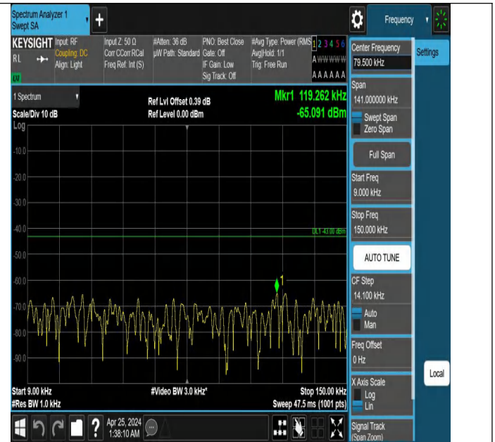
Band4_5MHz_QPSK_19975_1RB#24_0.009~0.15_0.009~0.15
