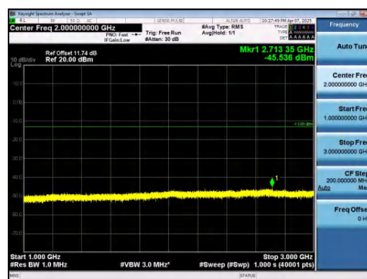
Band12-1.4MHz-QPSK-23173-1RB#0-1000~3000 0-PASS
