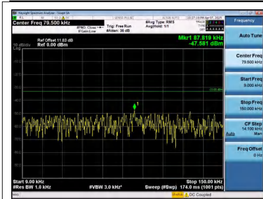
Band12-1.4MHz-QPSK-23173-1RB#0-0.009~0.1 5-PASS
