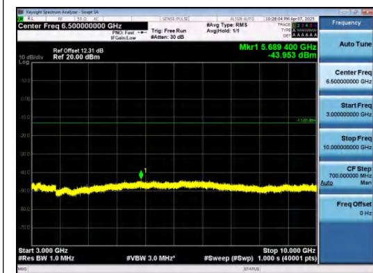
Band12-1.4MHz-QPSK-23173-1RB#0-3000~10000 00-PASS
