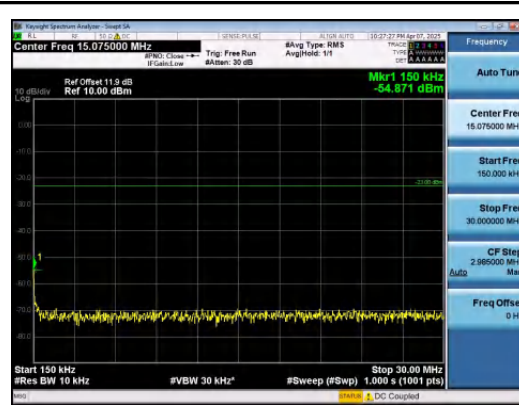
Band12-1.4MHz-QPSK-23173-1RB#0-0.15~30-P ASS
