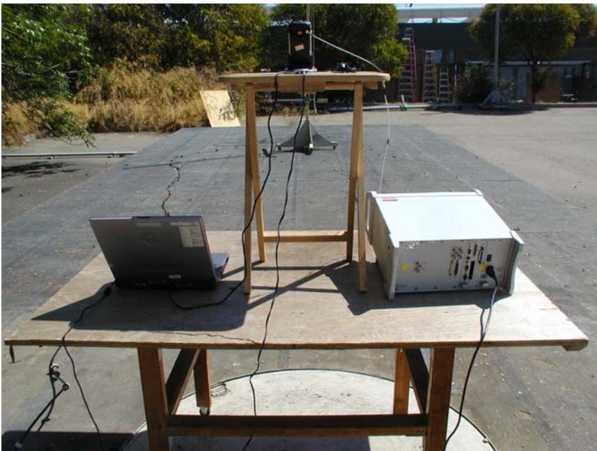
GSM Radiated Emission - Rear View
