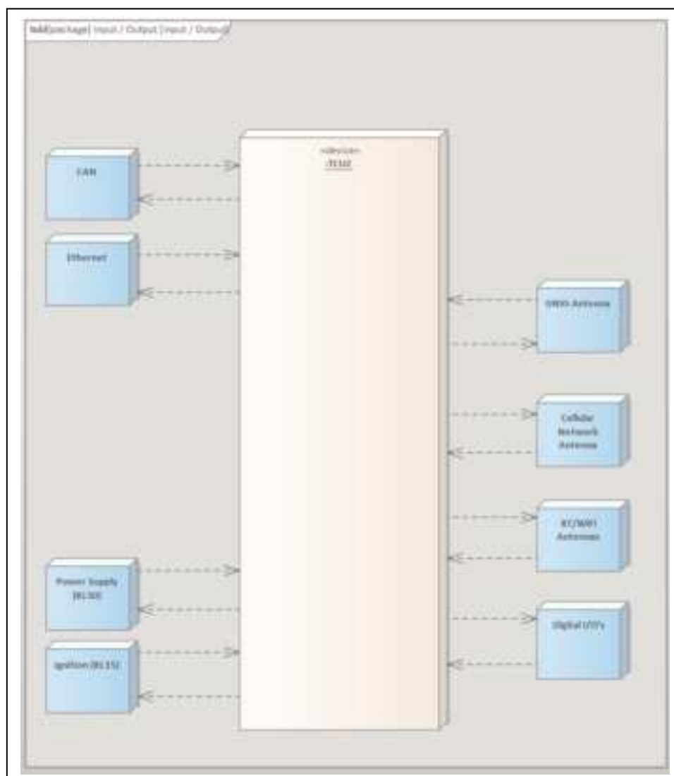
Figure 1: TCU2 in the system context
