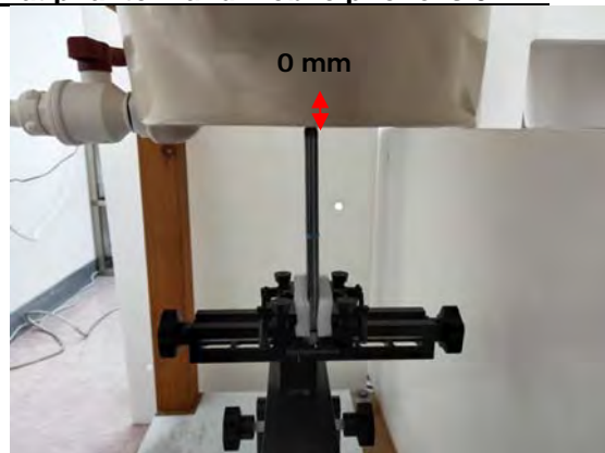
Fig.18 EUT Bottom side to flat phantom
