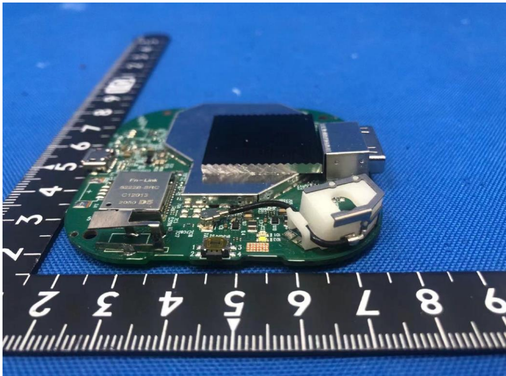
(4) Antenna Photo
