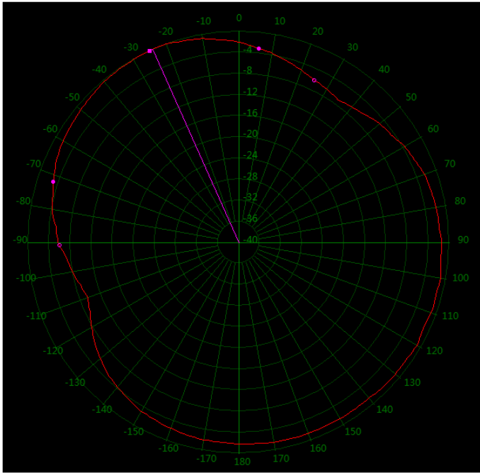
150 MHz Horizontal 360°
