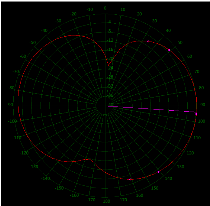
158 MHz Vertical 70°
