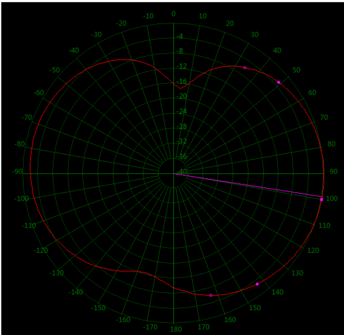
163 MHz Vertical 71°
