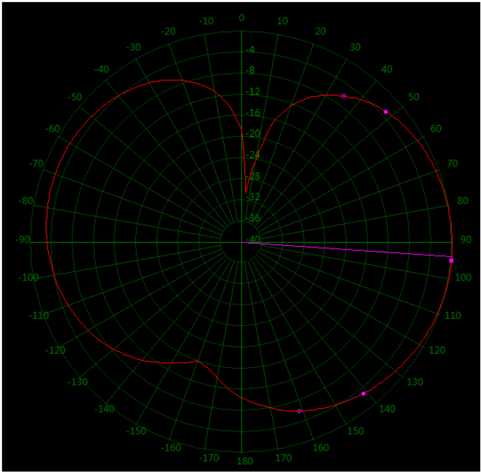
149 MHz Vertical 71°
