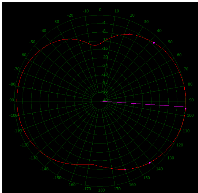
174 MHz Vertical 72°
