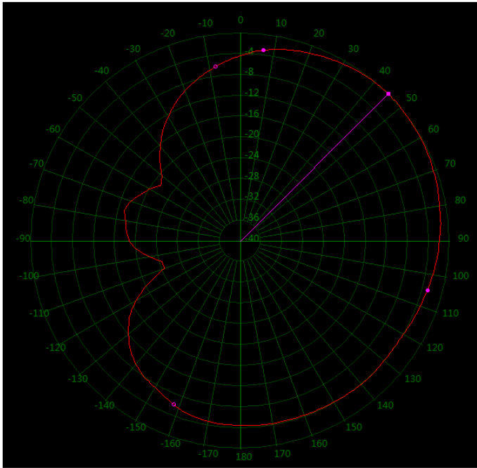
149 MHz Horizontal 360°
