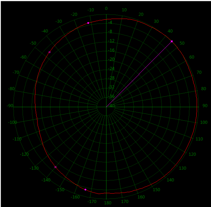
168 MHz Horizontal 360°
