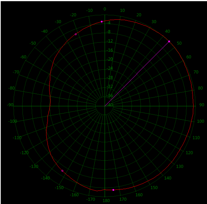
153 MHz Horizontal 360°
