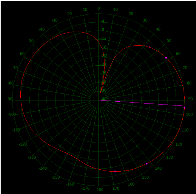
162 MHz Vertical 69°
