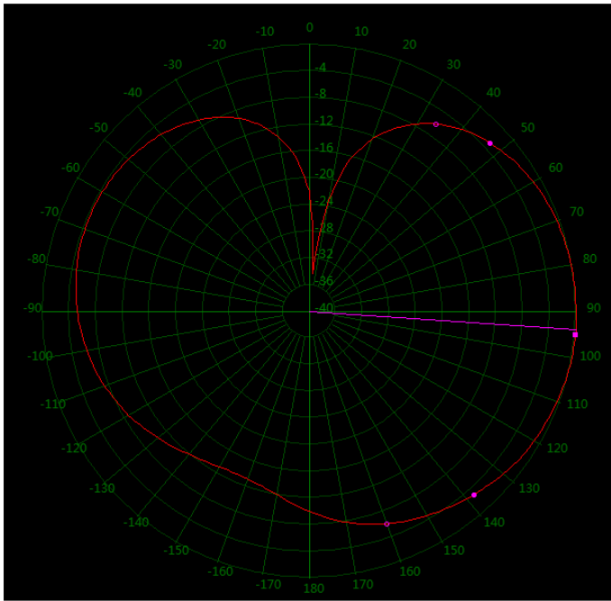
140 MHz Vertical 70°
