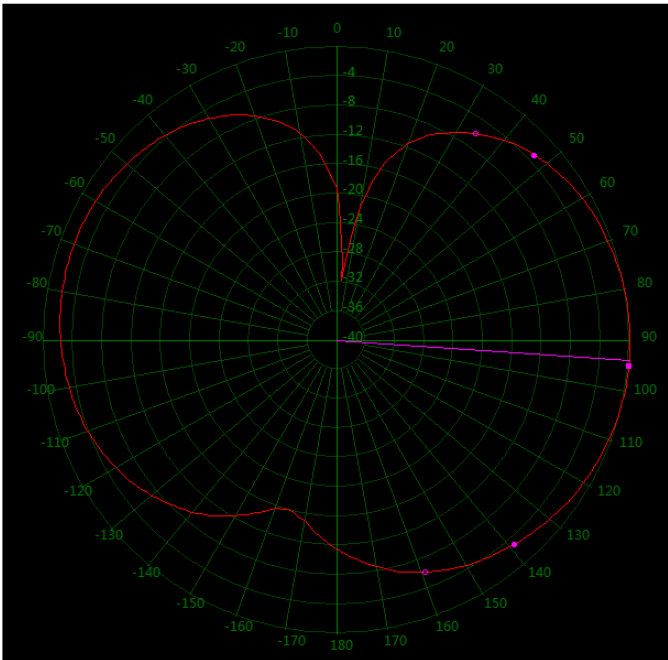
153 MHz Vertical 71°
