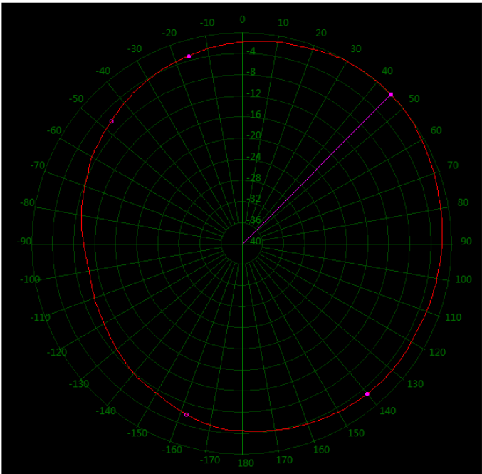
163 MHz Horizontal 360°
