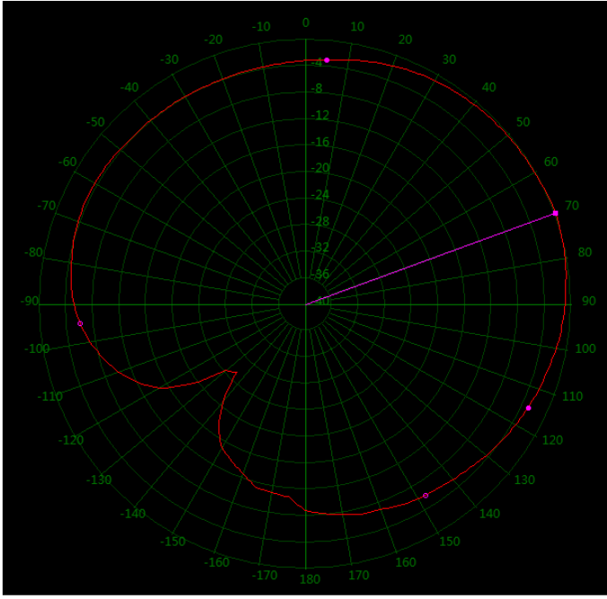
140 MHz Horizontal 360°
