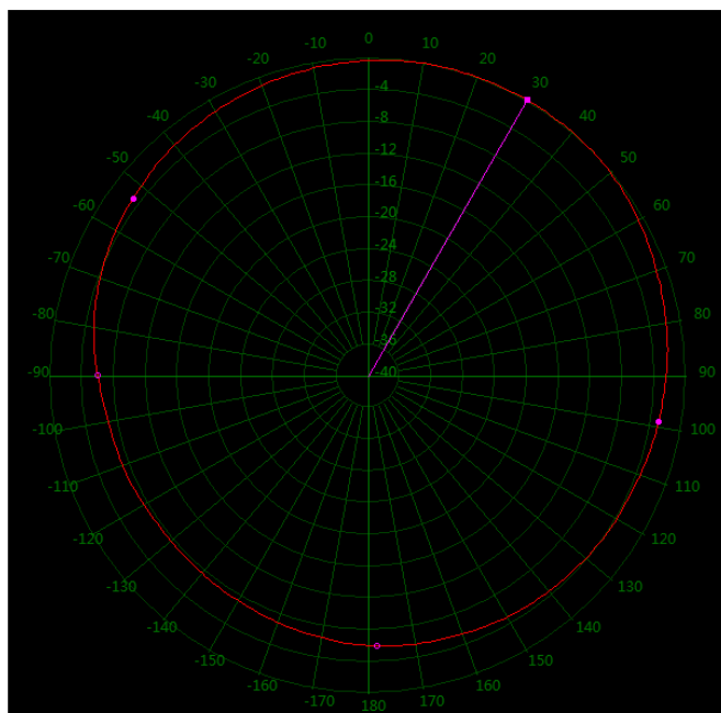
174 MHz Horizontal 360°
