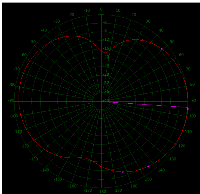
164 MHz Vertical 72°
