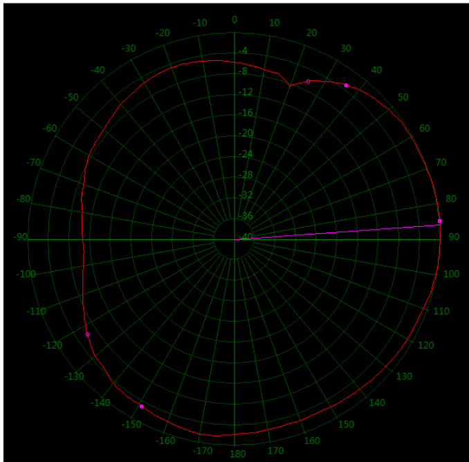
162 MHz Horizontal 360°
