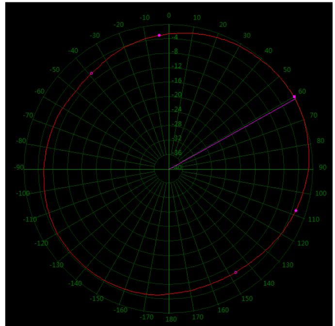
174 MHz Horizontal 360°
