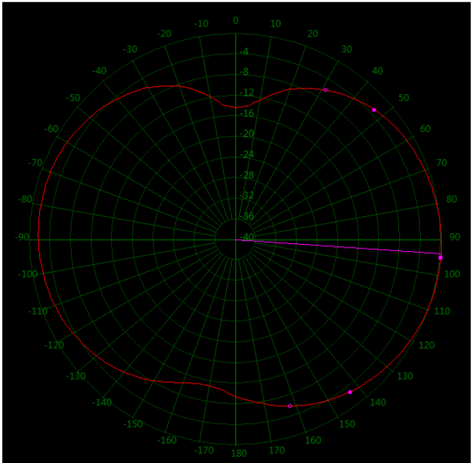
168 MHz Vertical 72°
