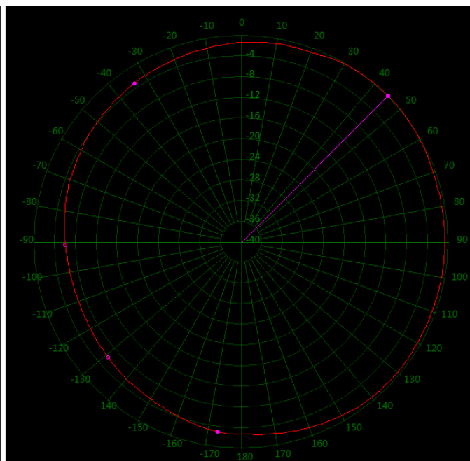
164 MHz Horizontal 360°
