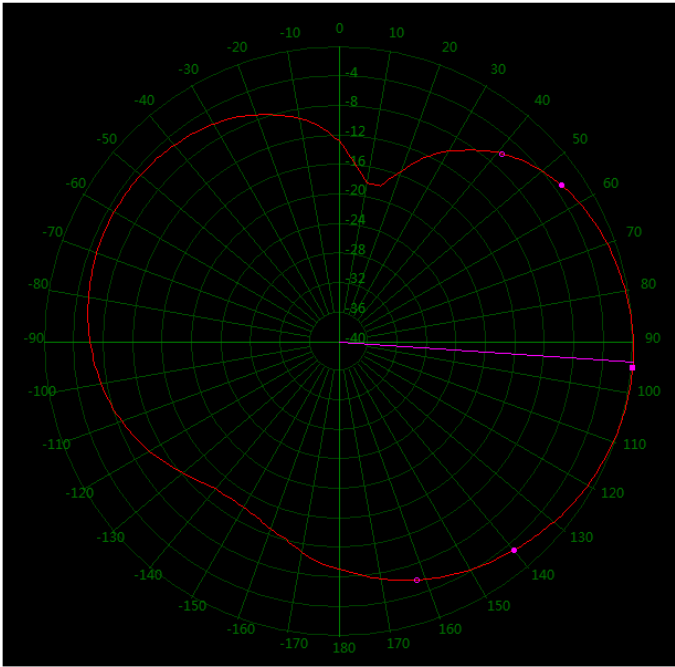
150 MHz Vertical 69°
