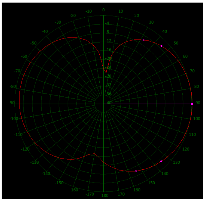
150 MHz Vertical 69°
