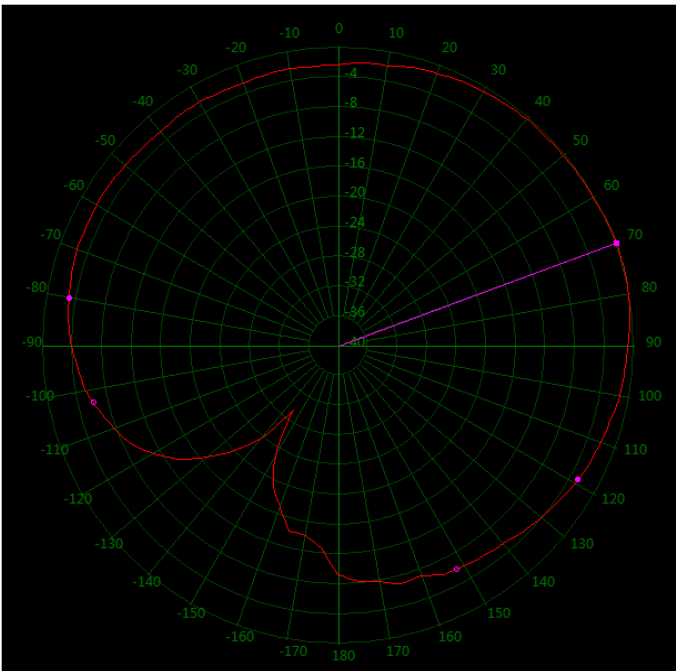
136 MHz Horizontal 360°
