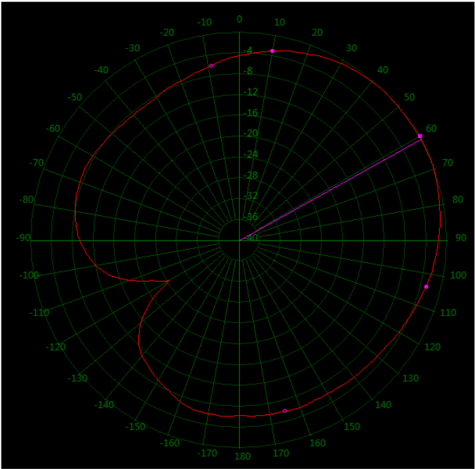
144 MHz Horizontal 360°
