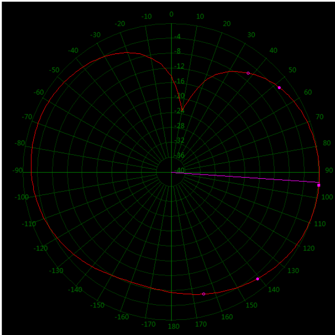
174 MHz Vertical 71°
