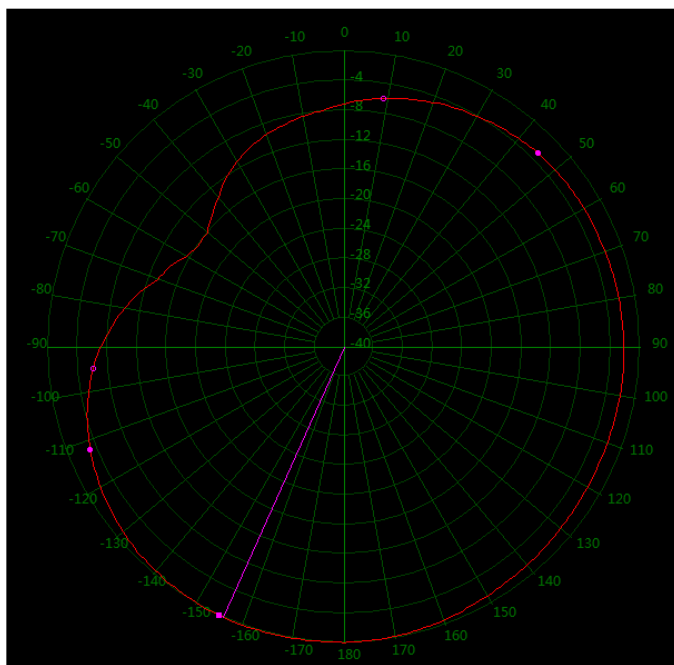
150 MHz Horizontal 360°
