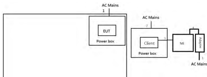
Test Setup Diagram – AC Line Conducted Emission Test –Beamforming
