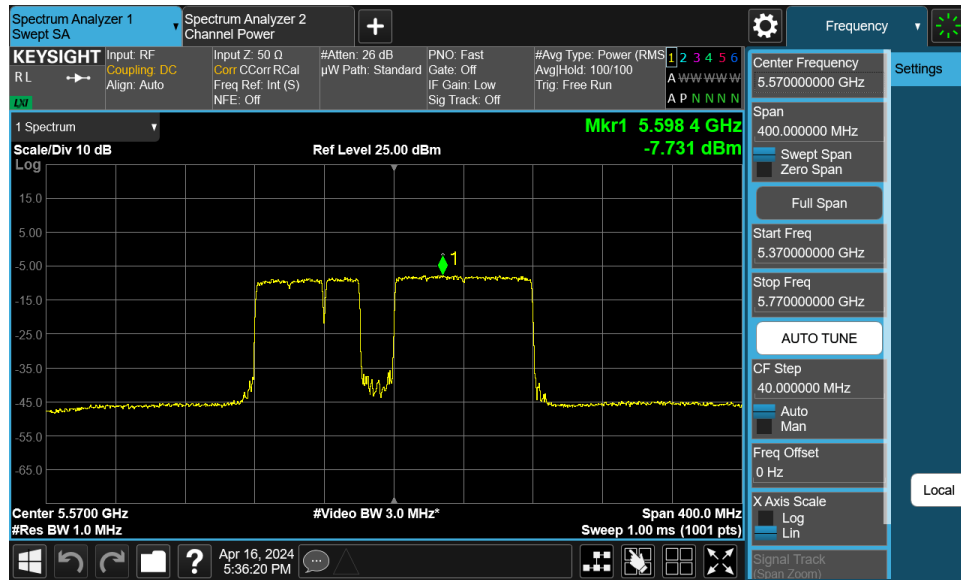
Plot 7-169. Power Spectral Density Plot MIMO ANT1 (160MHz BW 802.11be (UNII Band 2C) – Ch. 114)
