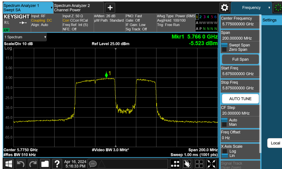
Plot 7-170. Power Spectral Density Plot MIMO ANT1 (80MHz BW 802.11be (UNII Band 3) – Ch. 155)
