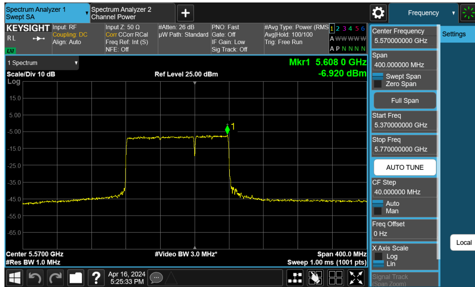
Plot 7-177. Power Spectral Density Plot MIMO ANT2 (160MHz BW 802.11be (UNII Band 2C) – Ch. 114)
