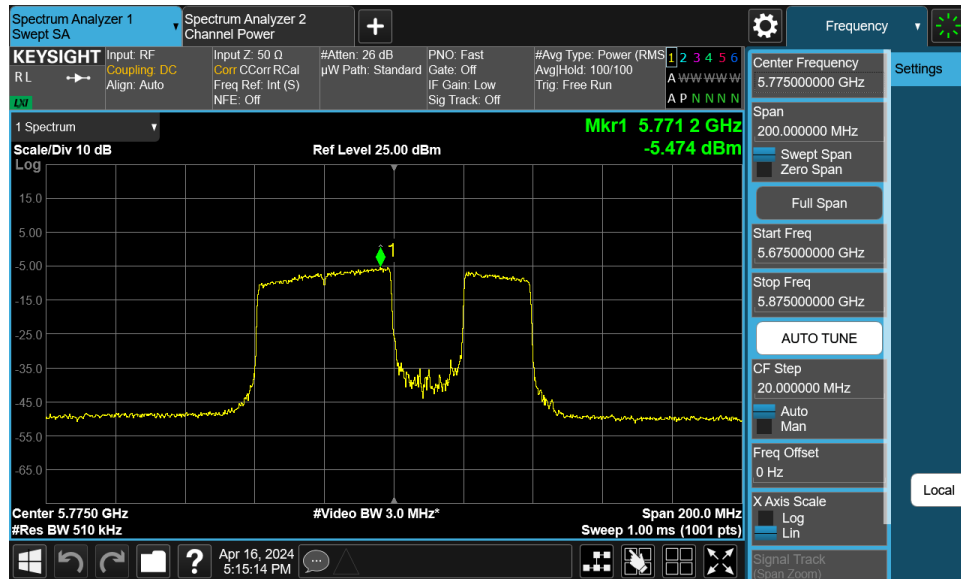
Plot 7-178. Power Spectral Density Plot MIMO ANT2 (80MHz BW 802.11be (UNII Band 3) – Ch. 155)
