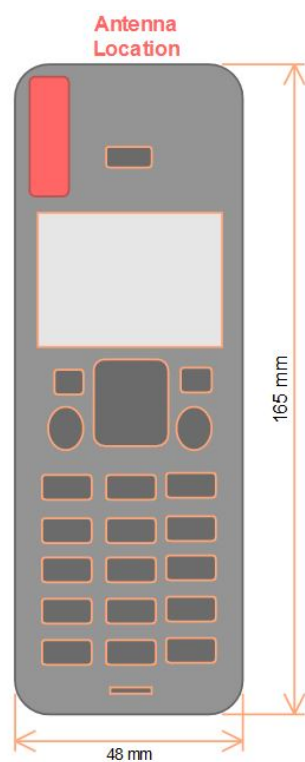
Fig. 1: Sketch of DUT and antenna location.
